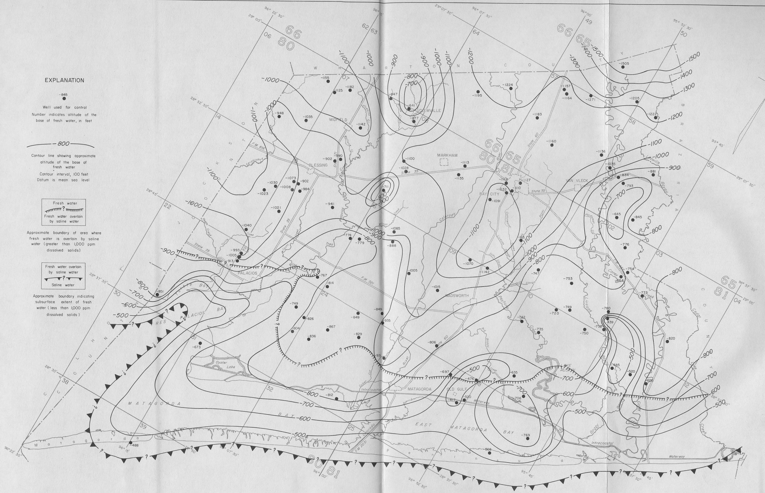
Figure 26 Approximate Altitude of the Base of Fresh Water (Less Than 1,000 ppm Dissolved Solids)
