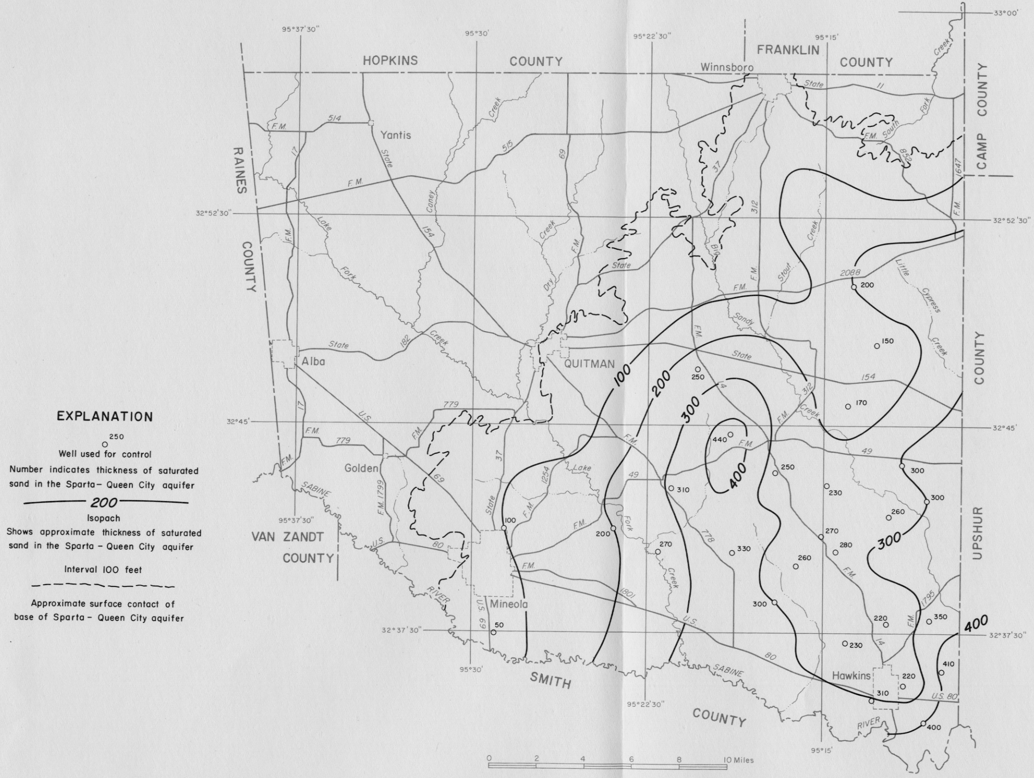
Figure 17 Approximate Thickness of Sand Containing Fresh Water in the Sparta-Queen City Aquifer
