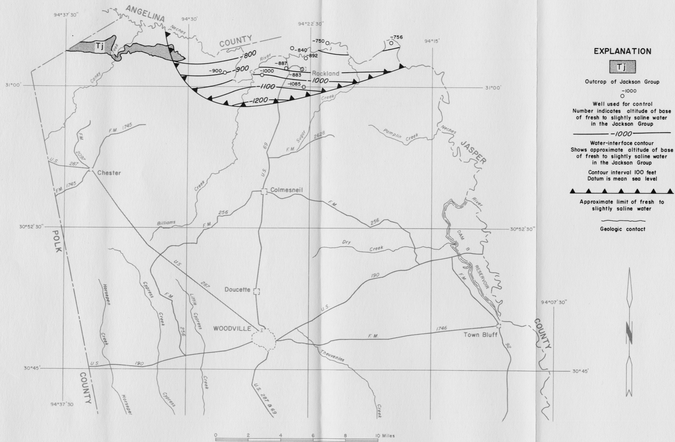
Figure 10 Approximate Altitude of the Base of Fresh to Slightly Saline Water in the Jackson Group, Northern Tyler County
