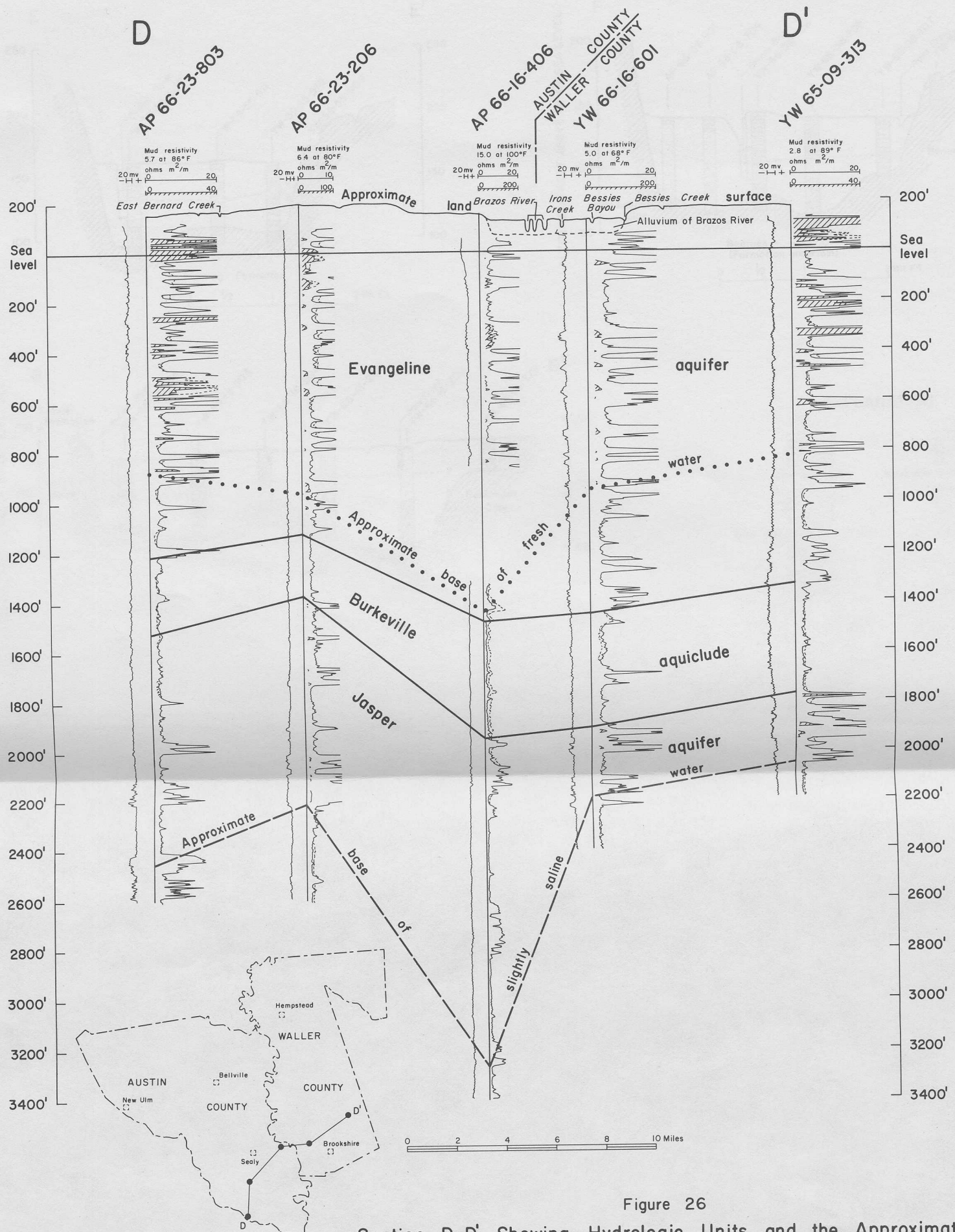
Section D-D', Showing Hydrologic Units and the Approximate Base of Fresh and Slightly Saline Water
