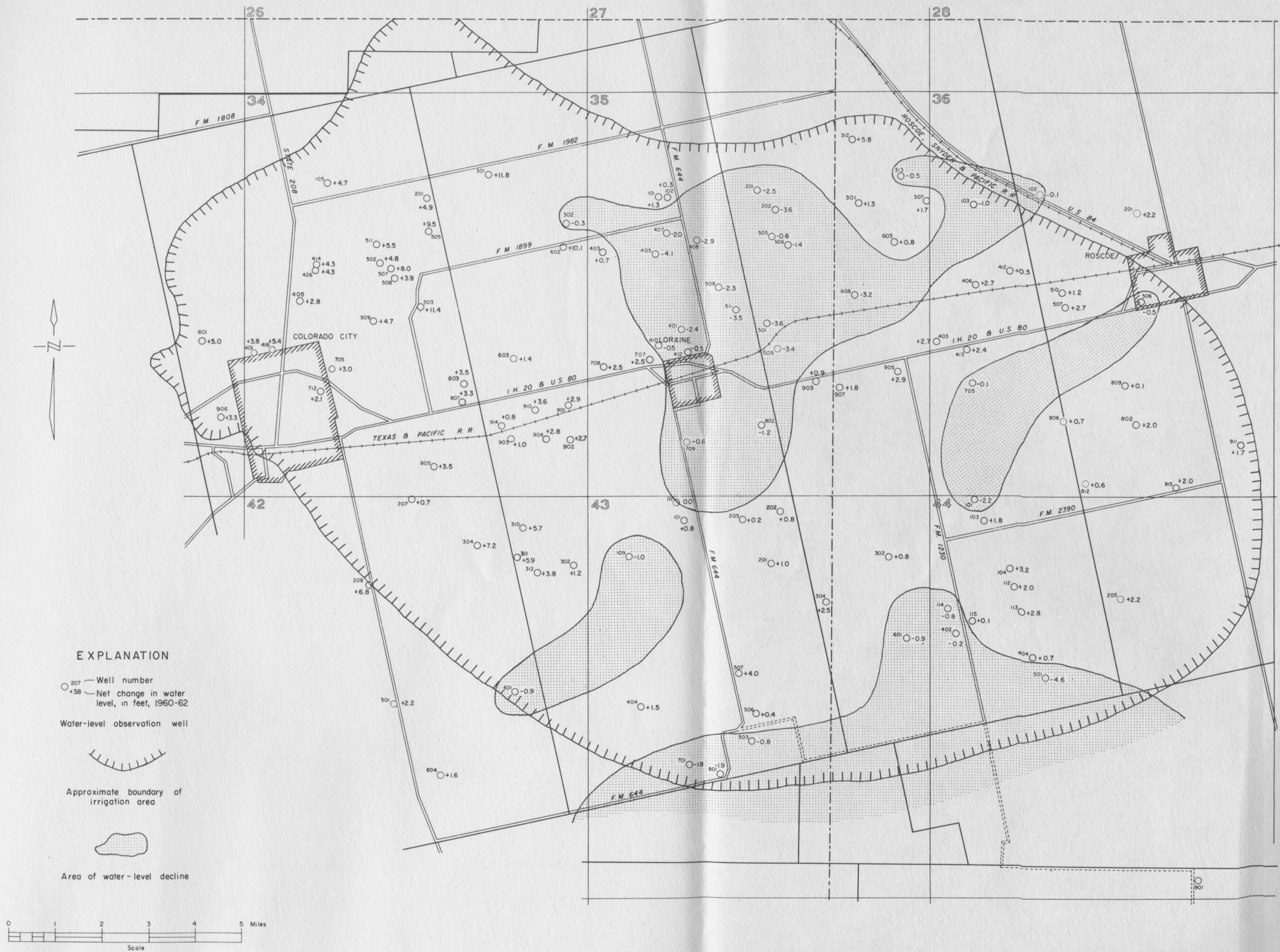
Figure 18 Changes in Winter Static Water Levels in Selected Wells in the Irrigation Area, 1960-62
