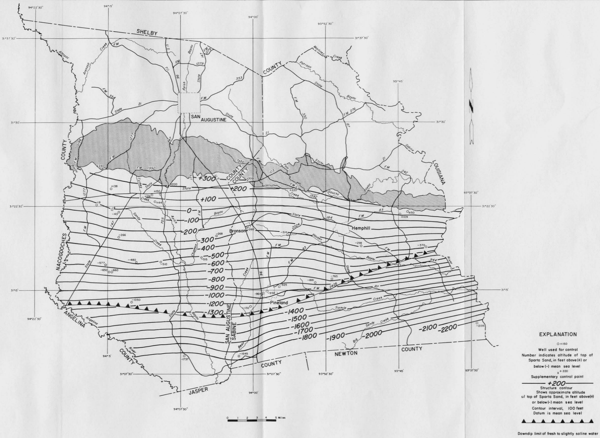
Figure 4 Structure-Contour Map of the Top of the Sparta Sand
