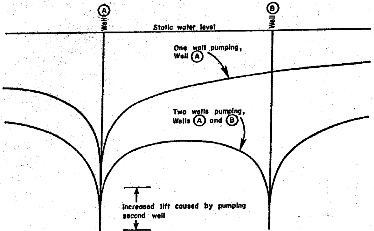
Figure 6 - Idealized Cross Section Showing Drawdown Interference Between Two Pumping Wells
