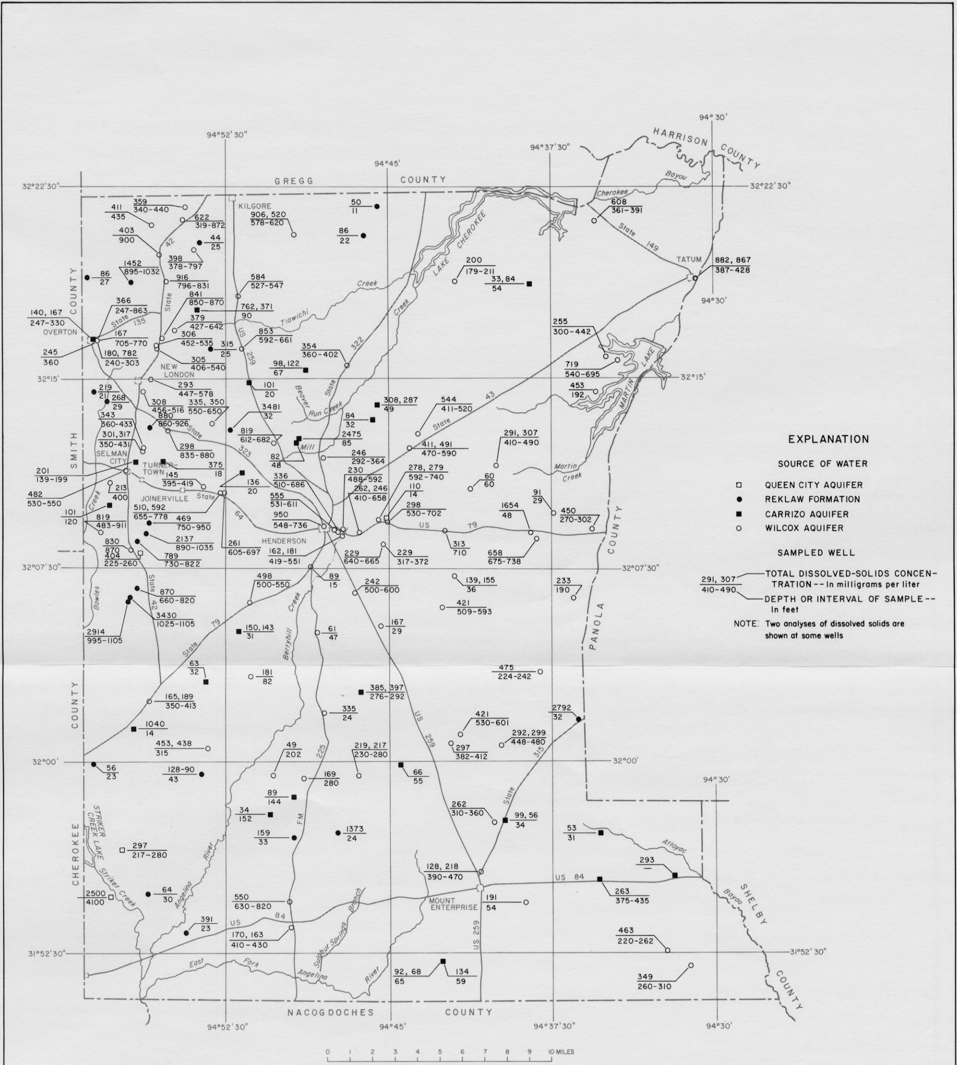
Figure 18 Total Dissolved-Solids Concentrations in Water From Selected Wells Screened in the Wilcox, Carrizo, and Queen City Aquifers and in the Reklaw Formation, 1981
