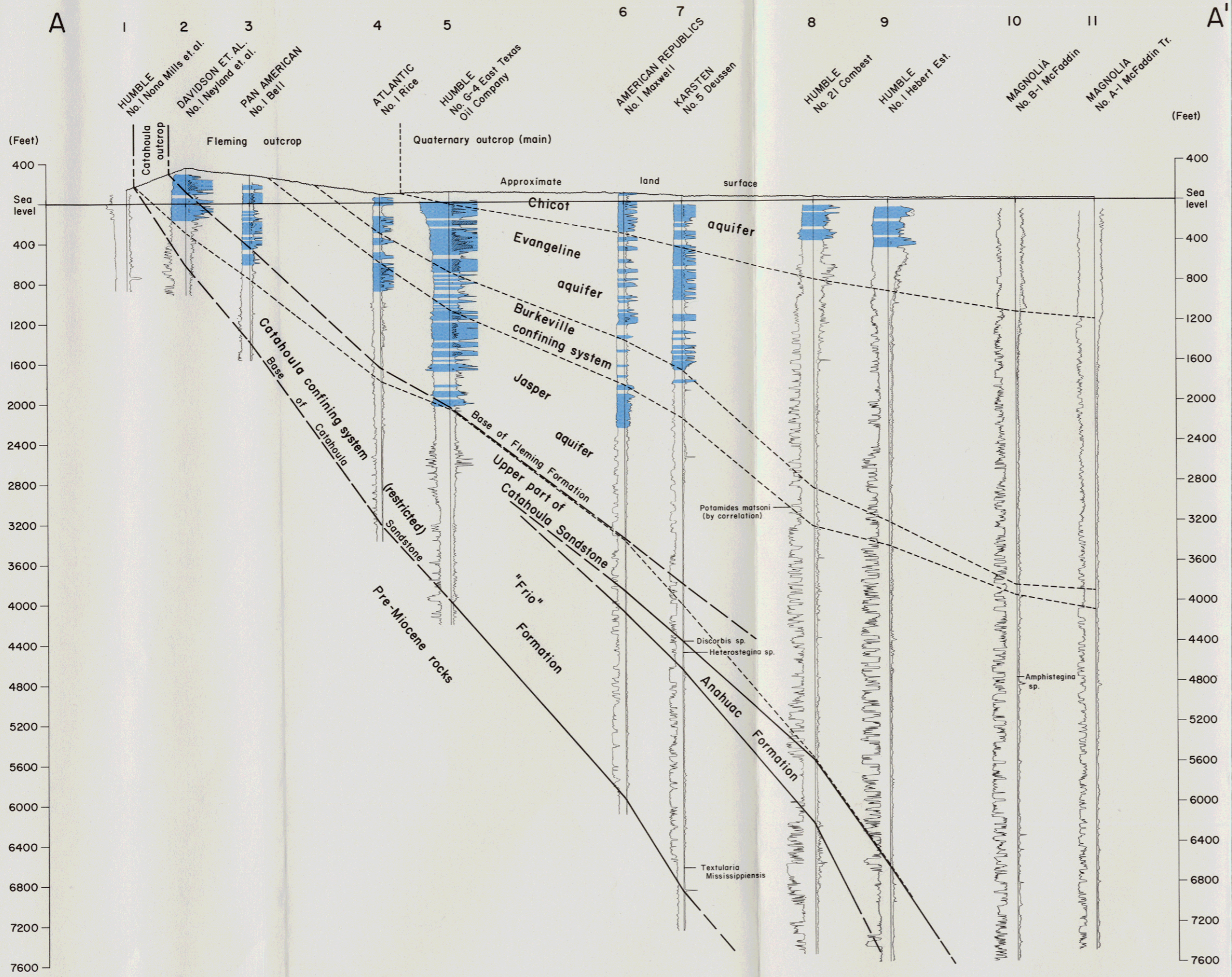
Figure 3 Stratigraphic and Hydrologic Section, A-A'
