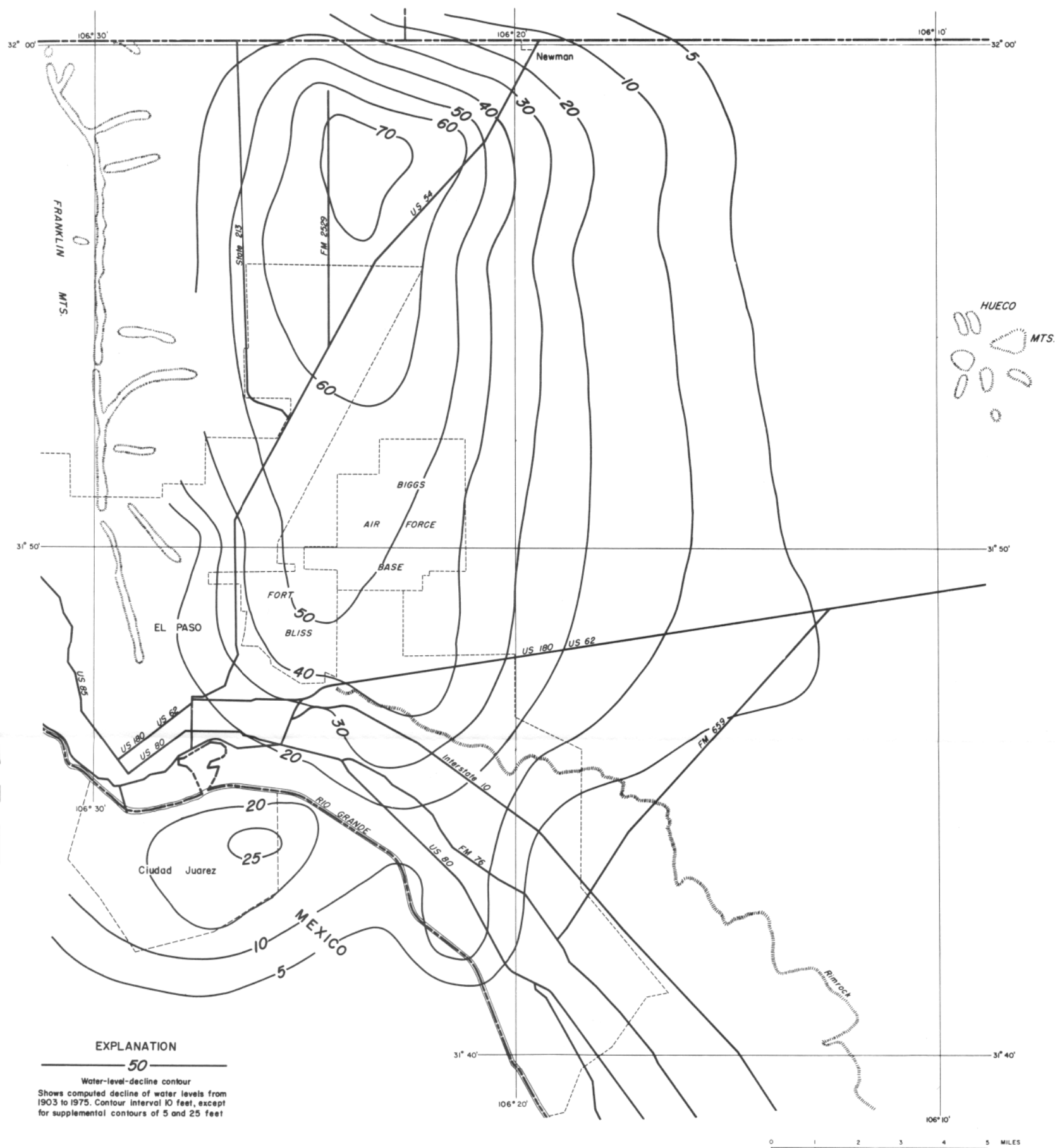
Figure II Predicted Decline in Water Levels, 1903-75, as Computed by Electrical-Analog Model
