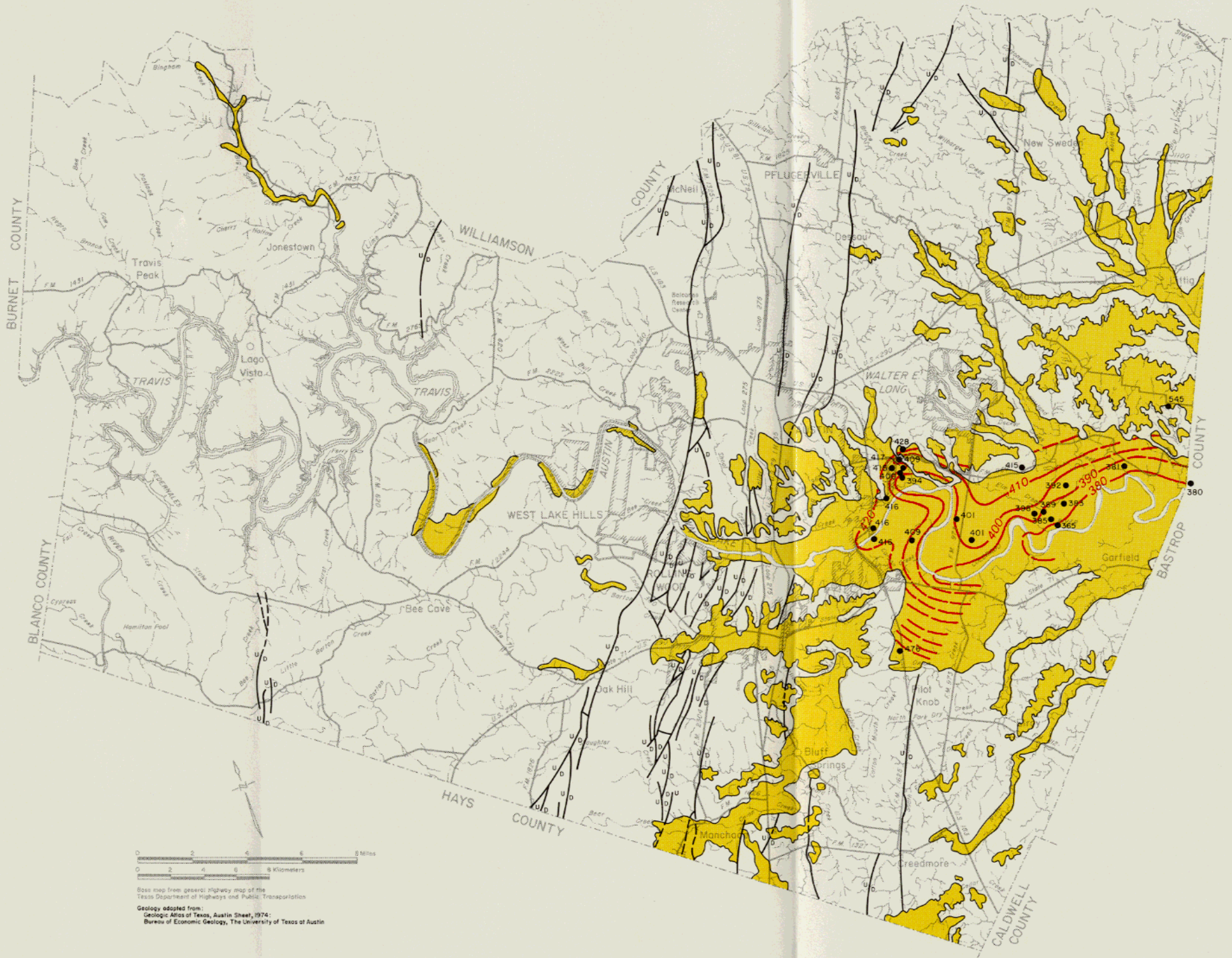
Figure 22 Approximate Altitude of Water Levels in Selected Wells Completed in the Alluvium and Terrace Deposits, Spring 1978
