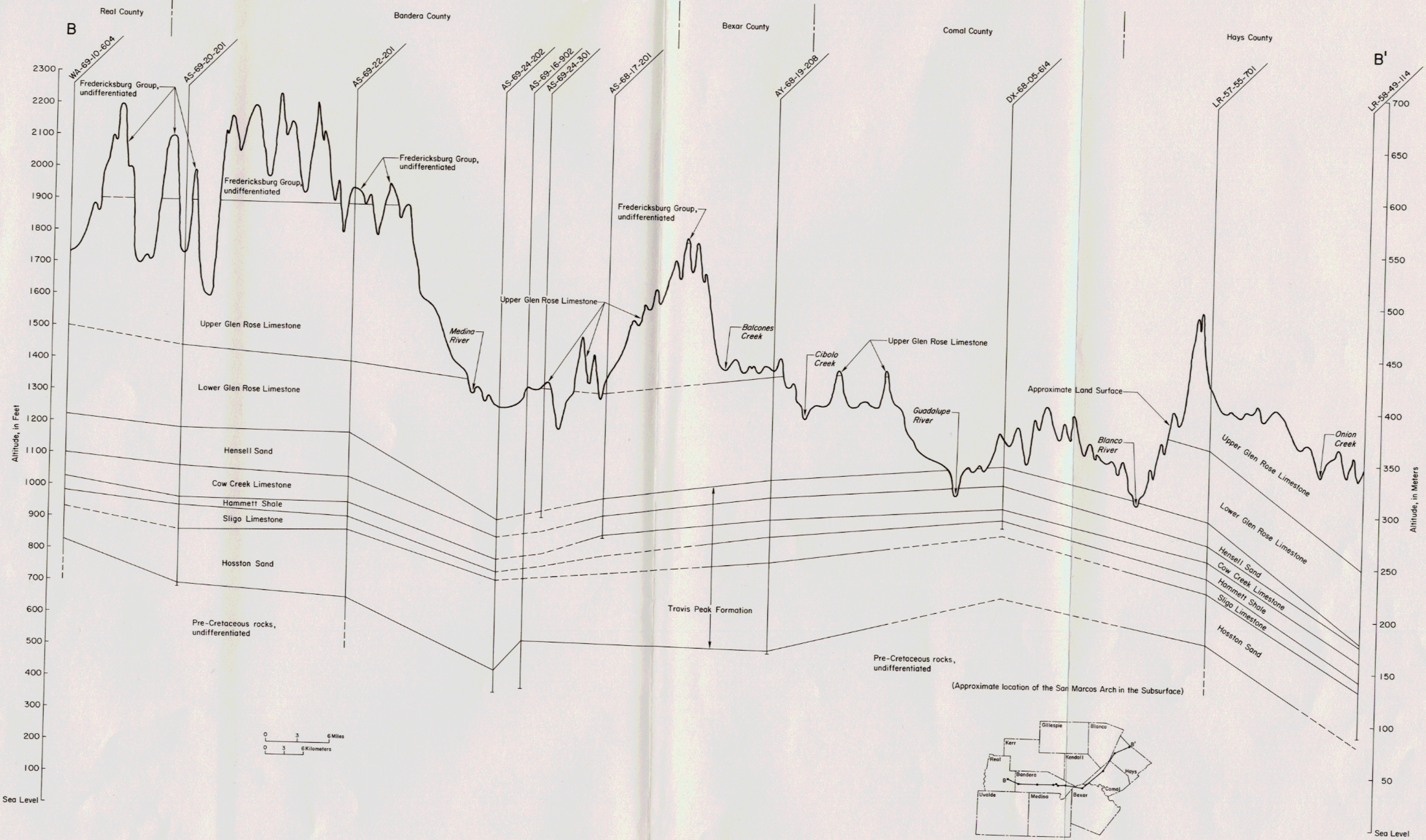
Figure 7 Geologic Section B-B'
