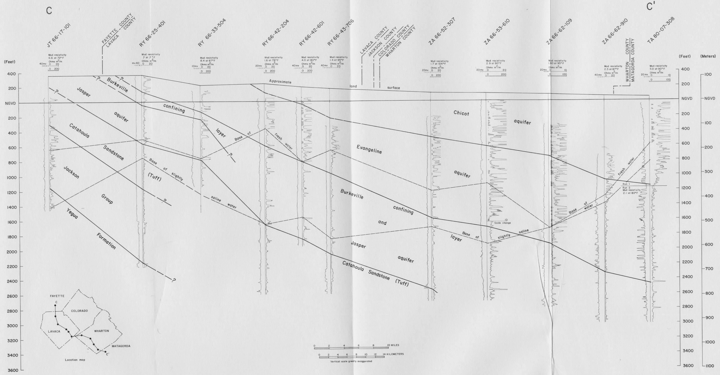
Figure 7 Geohydrologic Section C-C', Fayette, Lavaca, Wharton, and Matagorda Counties
