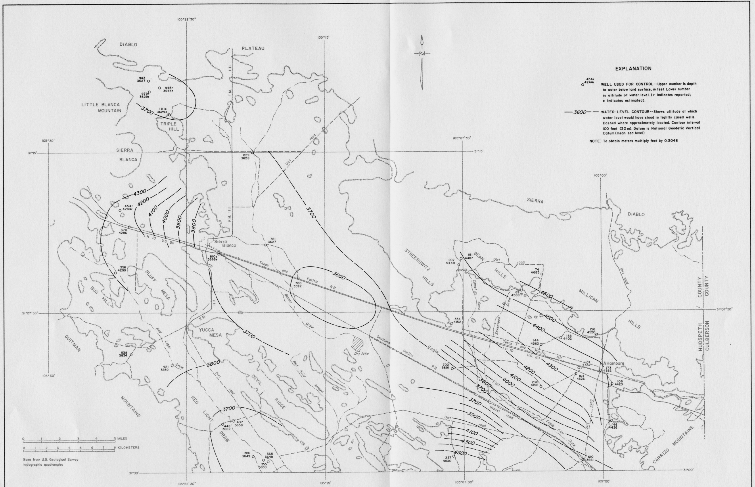
Figure 18 Water Levels in 1972-74 in Eagle Flat, Northern Red Light Draw, and Adjacent Areas
