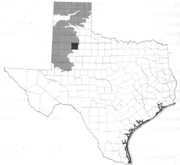
Location of Crosby County, and Extent of the Ogallala Aquifer in Texas
