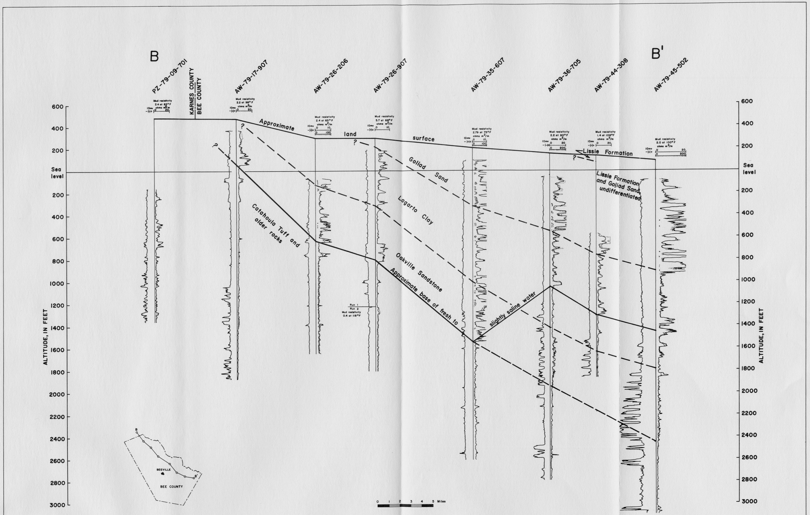
Plate 3 Geologic Section B-B', Karnes and Bee Counties U.S. Geological Survey in cooperation with the Texas Water Development Board
