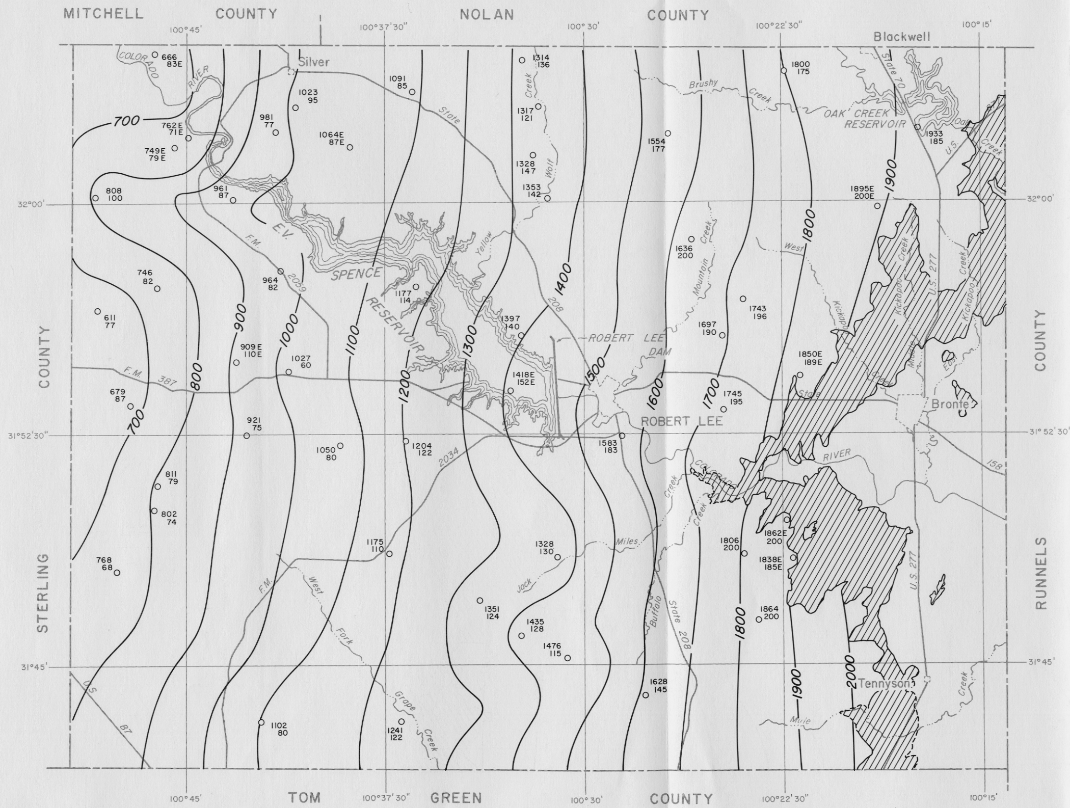
Figure 9 Approximate Thickness and Approximate Altitude of the Top of the San Angelo Sandstone
