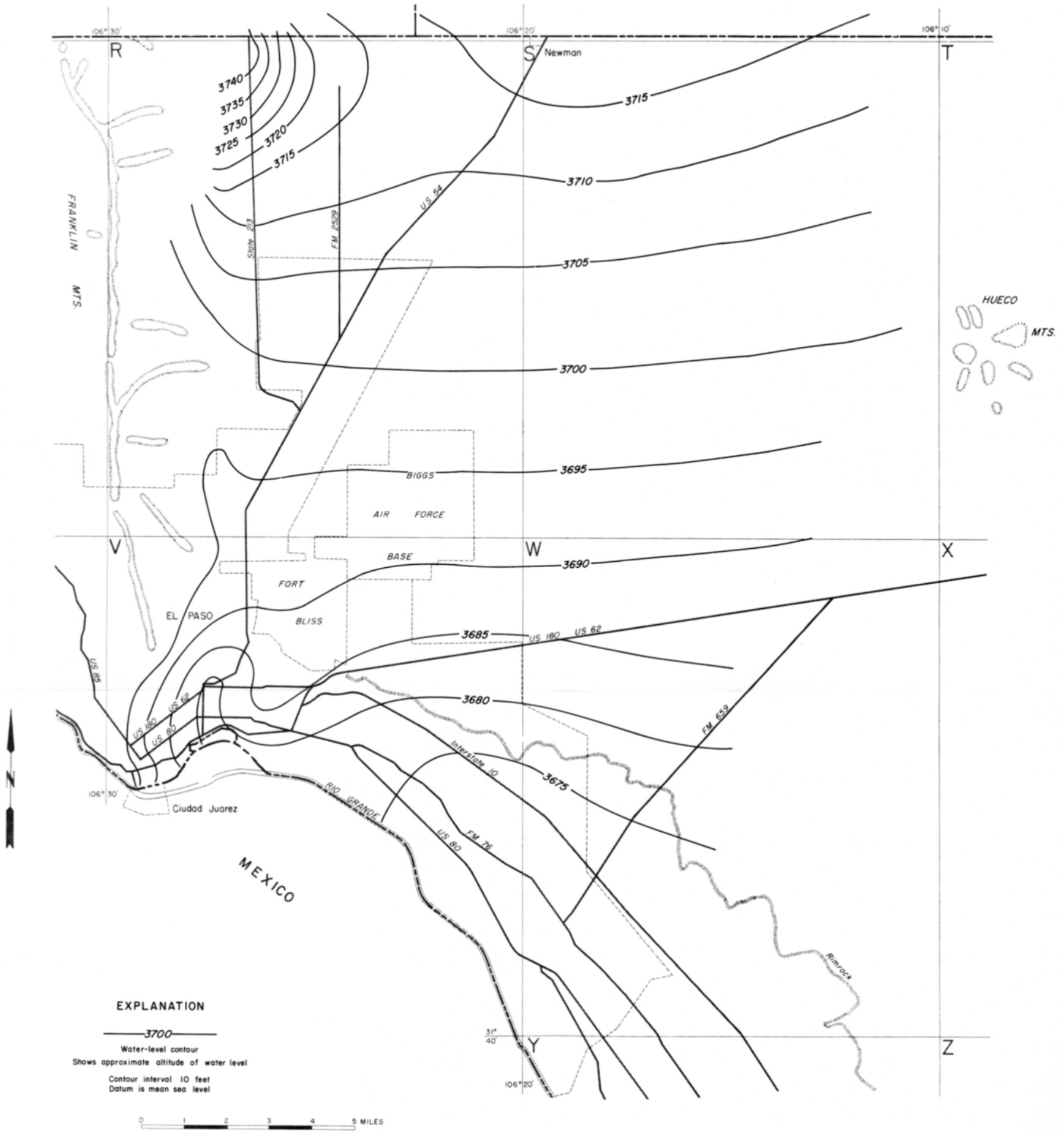
Figure 8 Approximate Altitude of Water Levels in the Hueco Bolson, 1903
