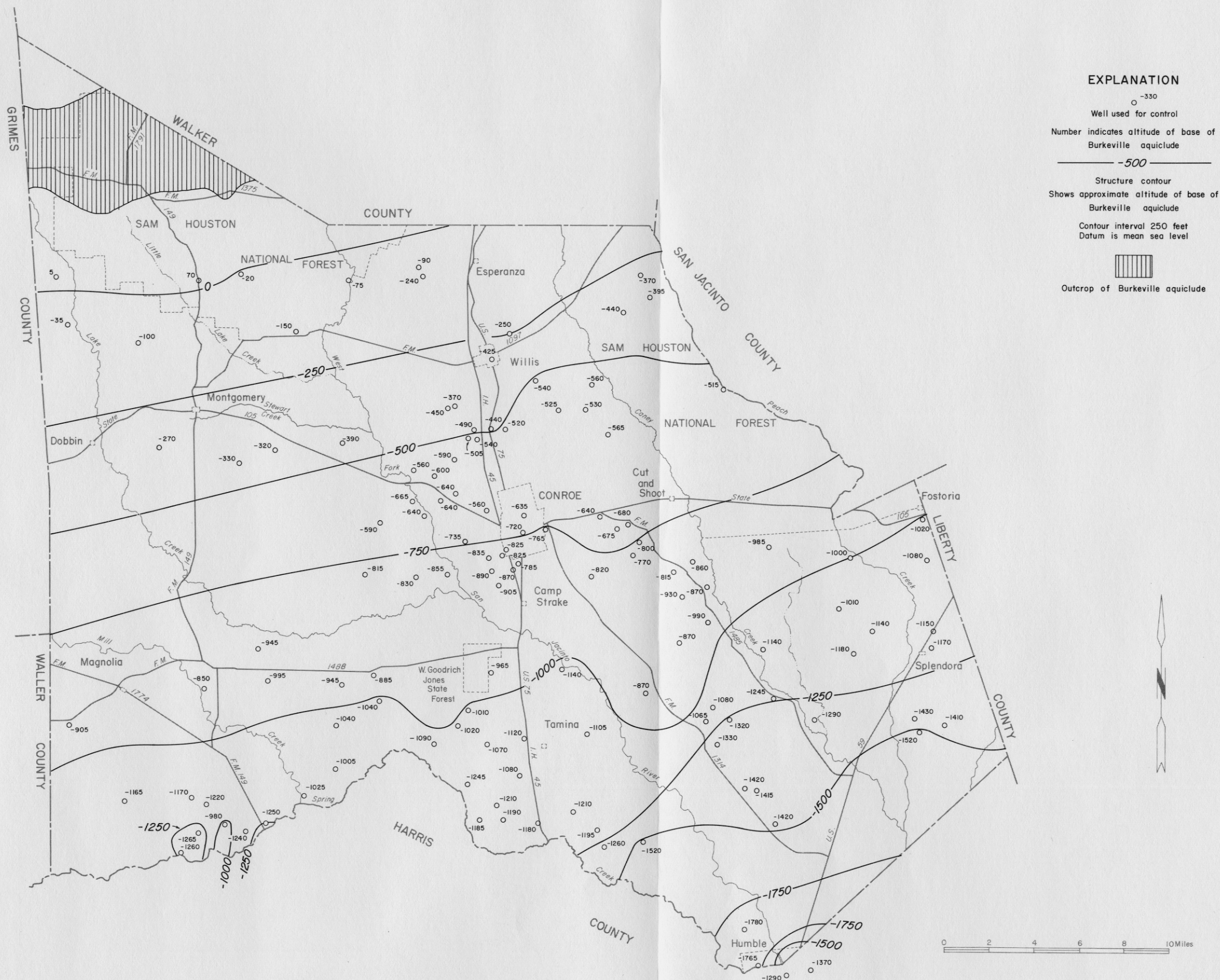
Figure 10 Approximate Altitude of the Base of the Burkeville Aquiclude
