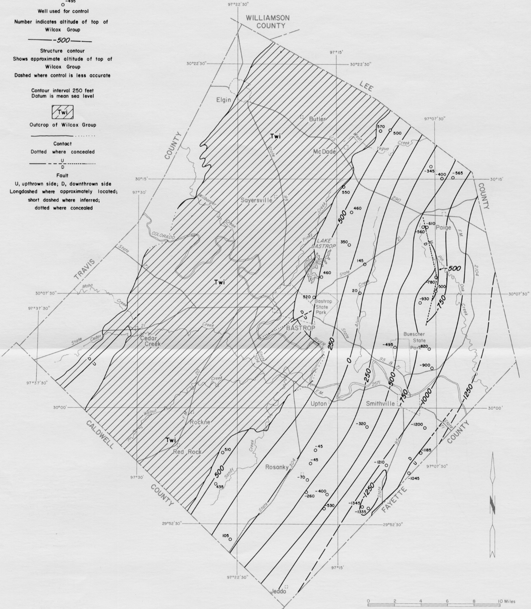
Figure 6 APPROXIMATE ALTITUDE OF THE TOP OF THE WILCOX GROUP
