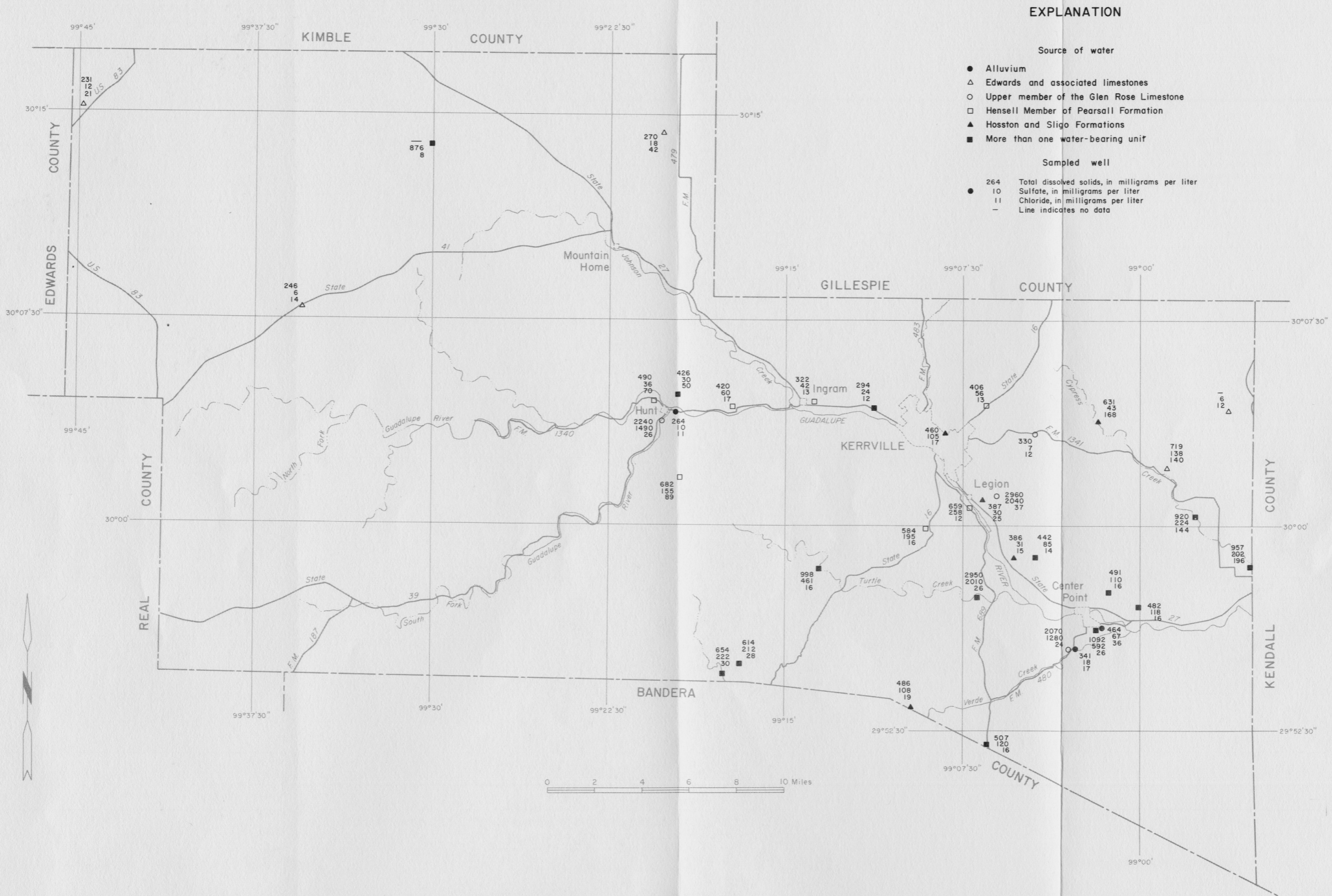
Figure 9 Dissolved-Solids, Sulfate, and Chloride Content of Water from Wells and Springs
