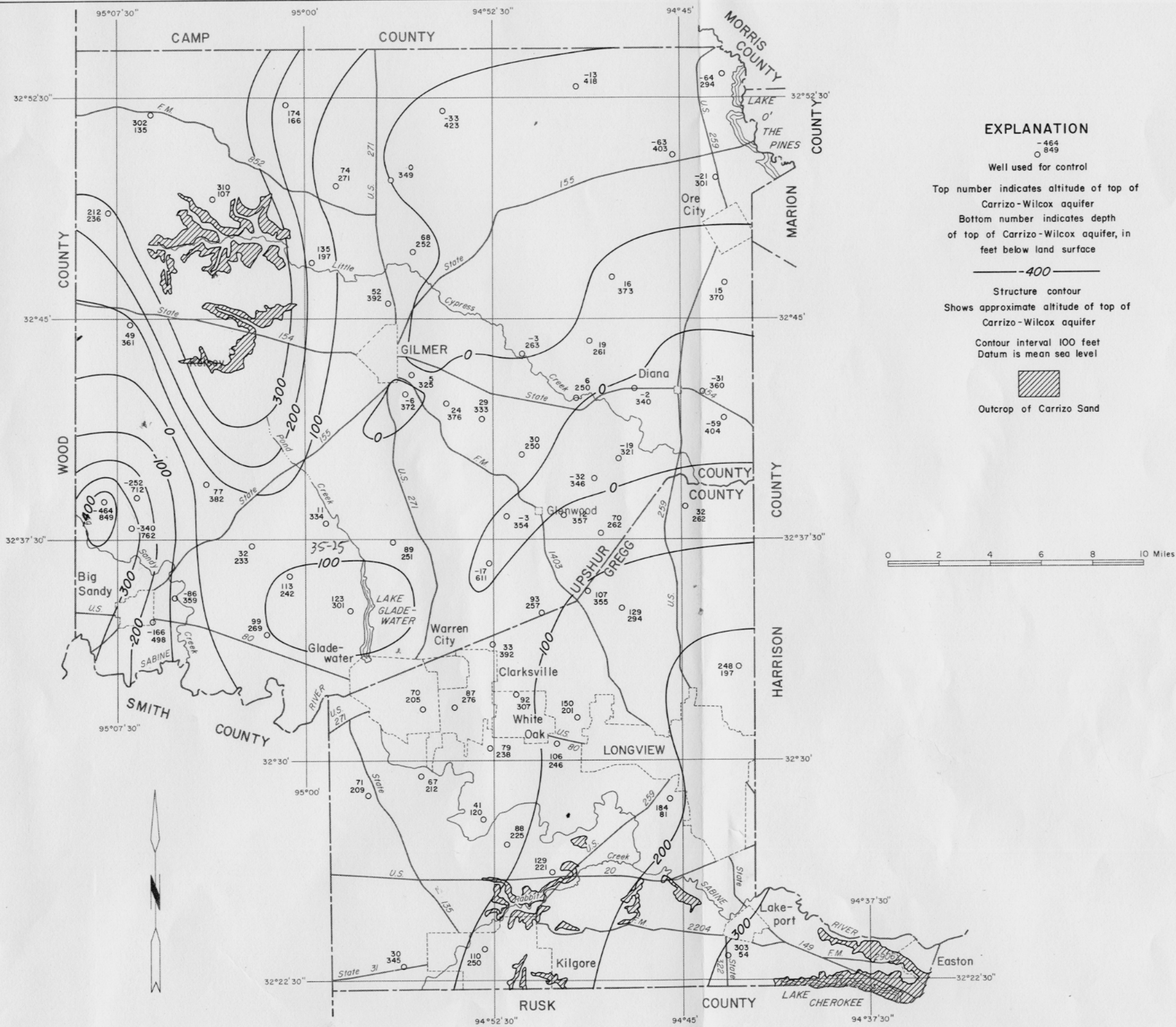
Figure 4 Approximate Altitude of and Depth to the Top of the Carrizo-Wilcox Aquifer
