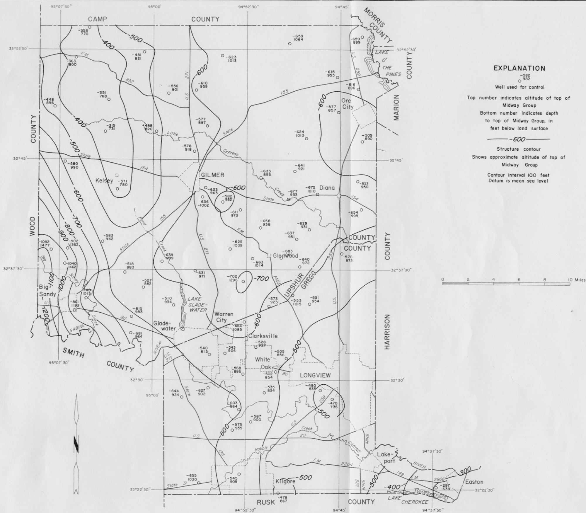
Figure 3 Approximate Altitude of and Depth to the Top of the Midway Group
