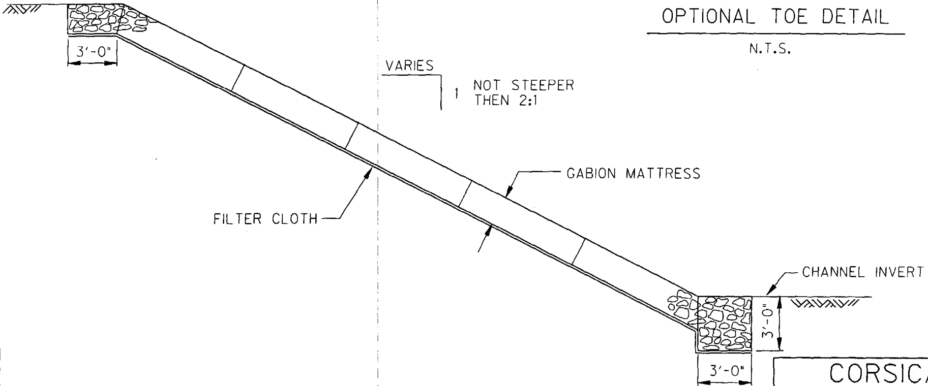
TYPICAL GABION MATTRESS SECTION
