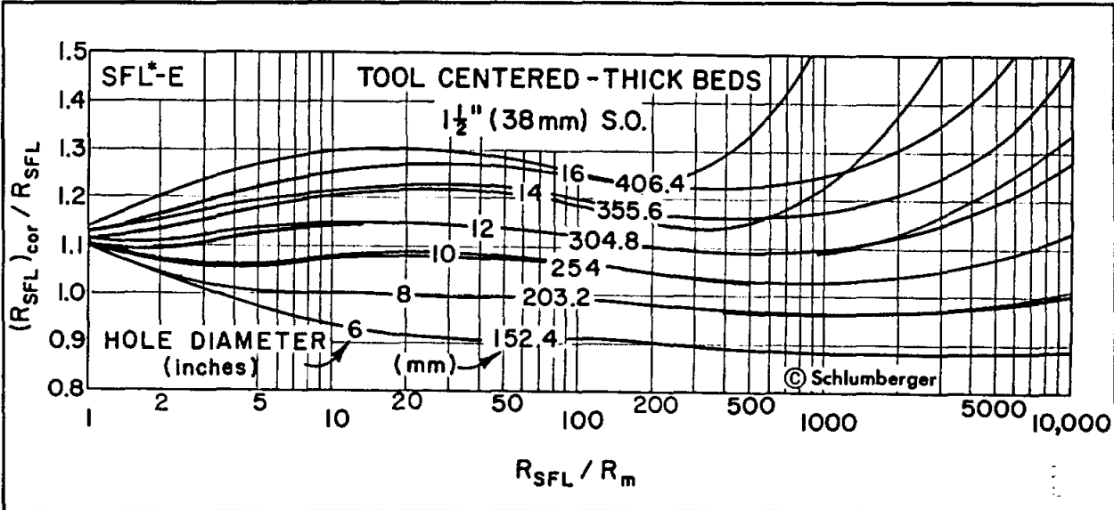
Figure 9-4. Borehole size and R_m correction chart for the Schlumberger SFL tool. R_m must be at formation temperature. S.O. is standoff (From Schlumberger, 1979).
