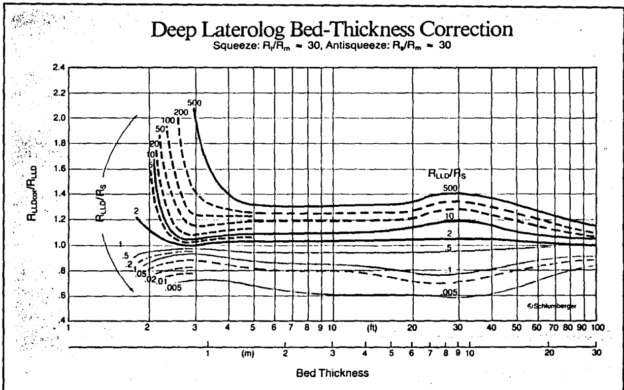
Figure 9-6. Bed thickness and adjacent bed departure curve for Schlumberger's LLD (Version DLS-D/E). The chart assumes no invasion, semi-infinite adjacent beds, and an 8 inch borehole (From Schlumberger, 1989).
