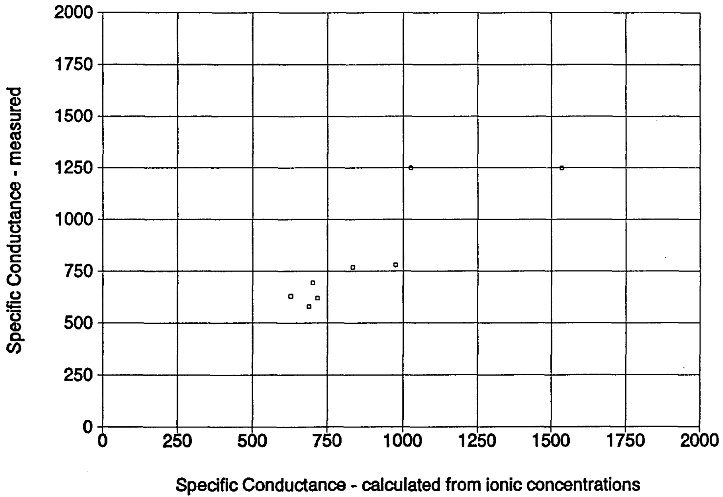
Figure 2-12. A graph of C_{w, \text{Measured}} versus C_{w, \text{Ion Conc.}} values ranging between 0 and 2,000 \mu\text{mhos/cm} . The data are from water analyses performed by Texas Testing Laboratories.
