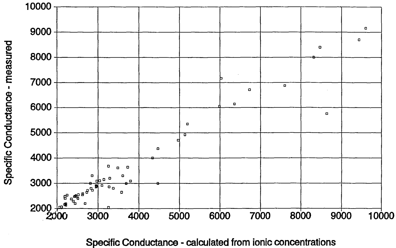
Figure 2-2. A graph of C_{w, \text{Measured}} versus C_{w, \text{Ion Conc.}} values ranging between 2,000 and 10,000 \mu\text{mhos/cm} . The data are from water analyses performed by Cortis, Edna Wood, Microbiology Service, Pope Testing, Texas Testing, and Texas Department of Health Laboratories.
