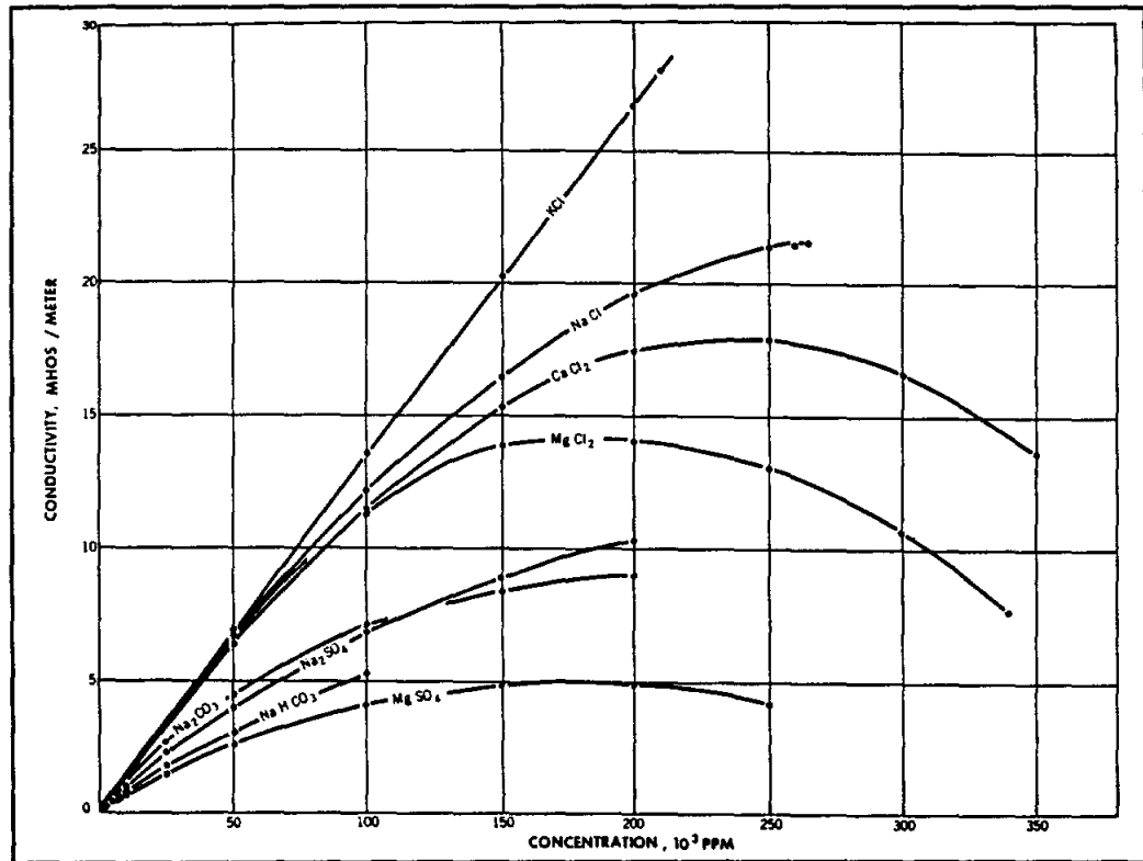
Figure 2-22. Conductivity of salt solutions at 18° C (From Moore, 1966).
