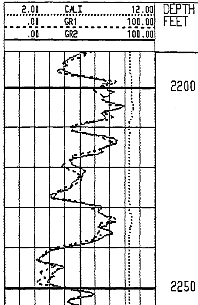
Figure 10-2. The effect of statistical variations on gamma ray curves. Both passes are the same eccentric tool pulled at 40 feet per minute. Differences are due to statistical variations. Shales are reading about 70 API units. The sandstones are shaly. Bed boundaries have excellent repeatability. The caliper shows slight washouts in two of the shales. The borehole fluid is fresh water bentonite mud. The log is the Paluxy Sandstone in Grayson County, Texas. Figures 9-21, 9-23, 10-1, 10-6 and 11-5 are from the same well.
