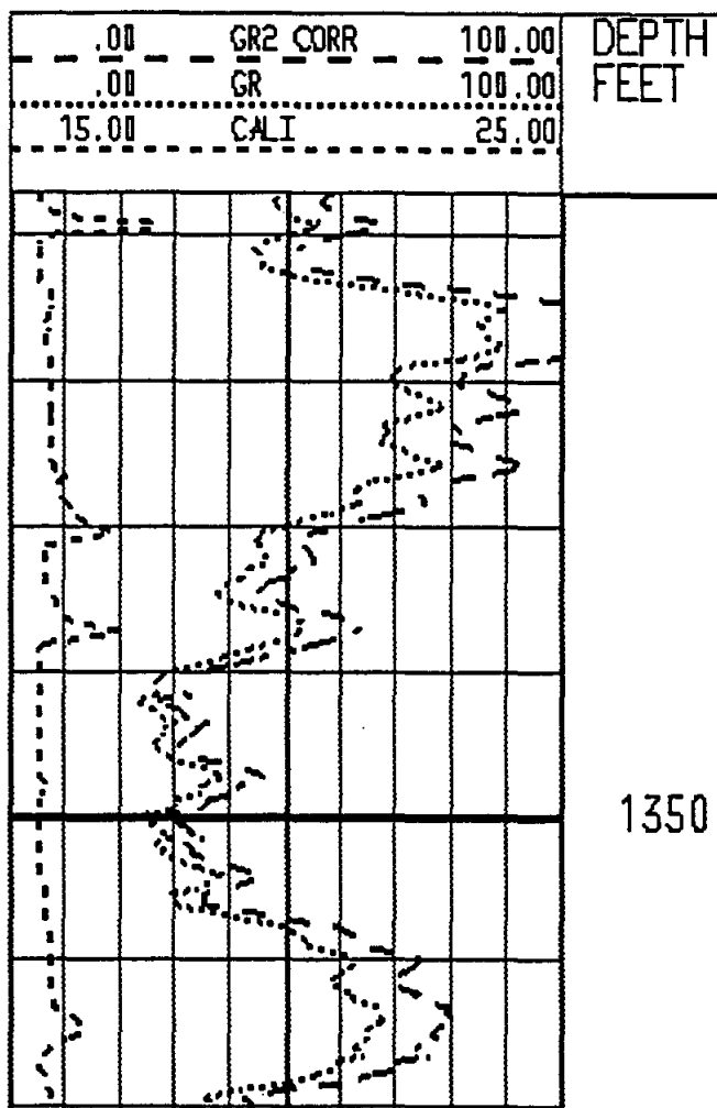
Figure 10-6. The effect of hole size and mud weight corrections on a gamma ray curve. GR2 CORR is the corrected curve. The corrected curve shape remains the same, but the entire curve is shifted. Bit size is 14.75 inches and mud weight is 9 lb/gal. The log is the Paluxy Sandstone in Grayson County, Texas. Figures 9-21, 9-23, 10-1, 10-2 and 11-5 are from the same well.
