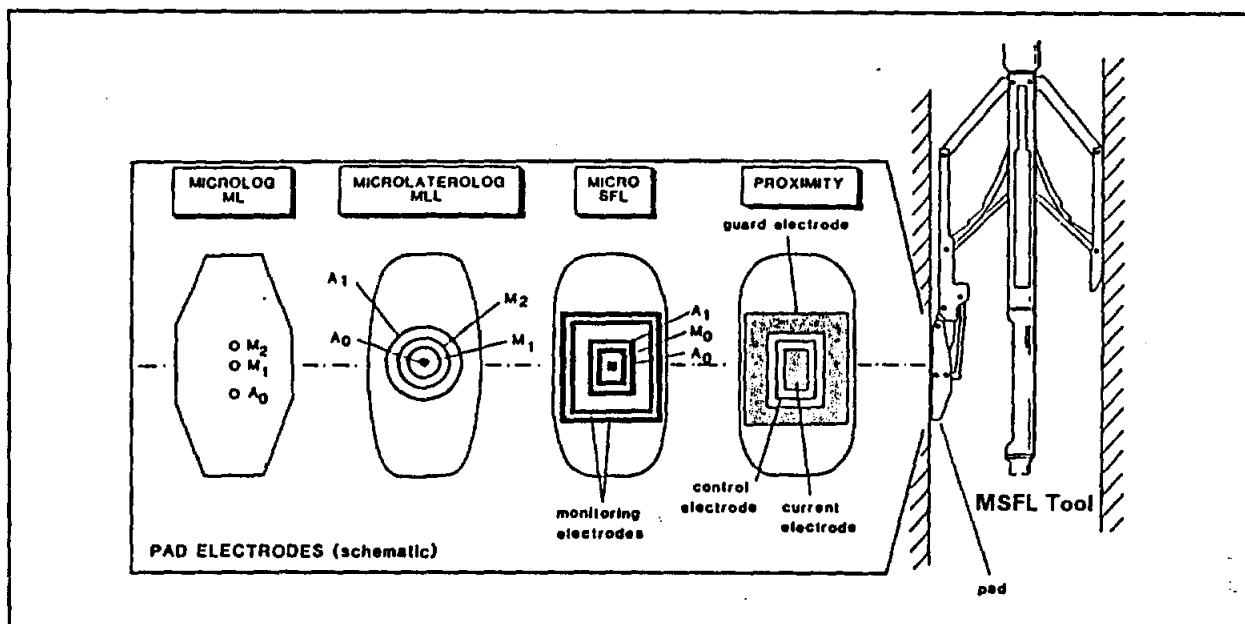
Figure 9-9. Schematic electrode configuration of focused pad microelectrode tools. A and M are electrodes (From Rider, 1986).
