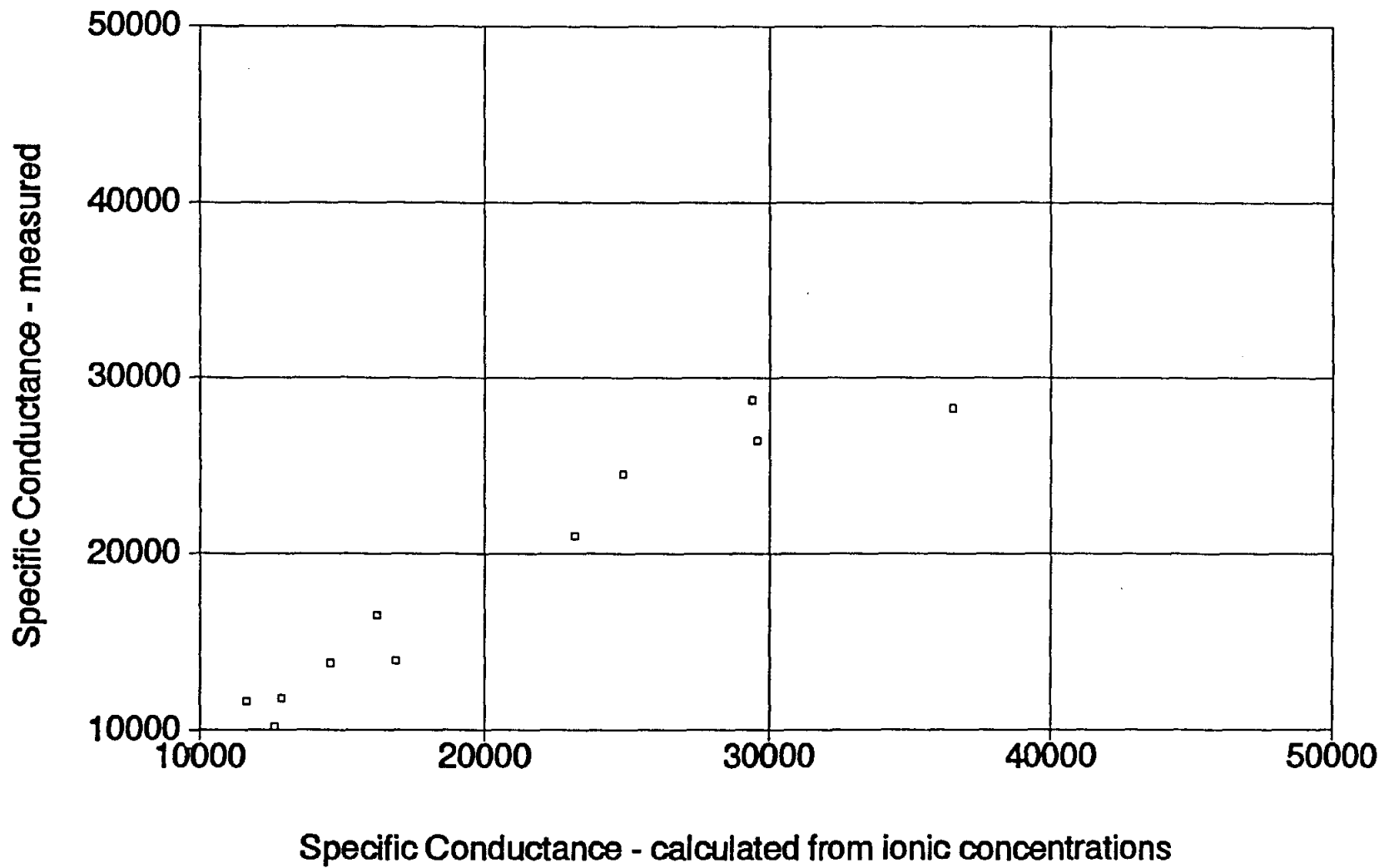
Figure 2-3. A graph of C_{w, \text{Measured}} versus C_{w, \text{Ion Conc.}} values ranging between 10,000 and 50,000 \mu\text{mhos/cm} . The data are from water analyses performed by Curtis, Edna Wood, Microbiology Service, Pope Testing, Texas Testing, and Texas Department of Health Laboratories.
