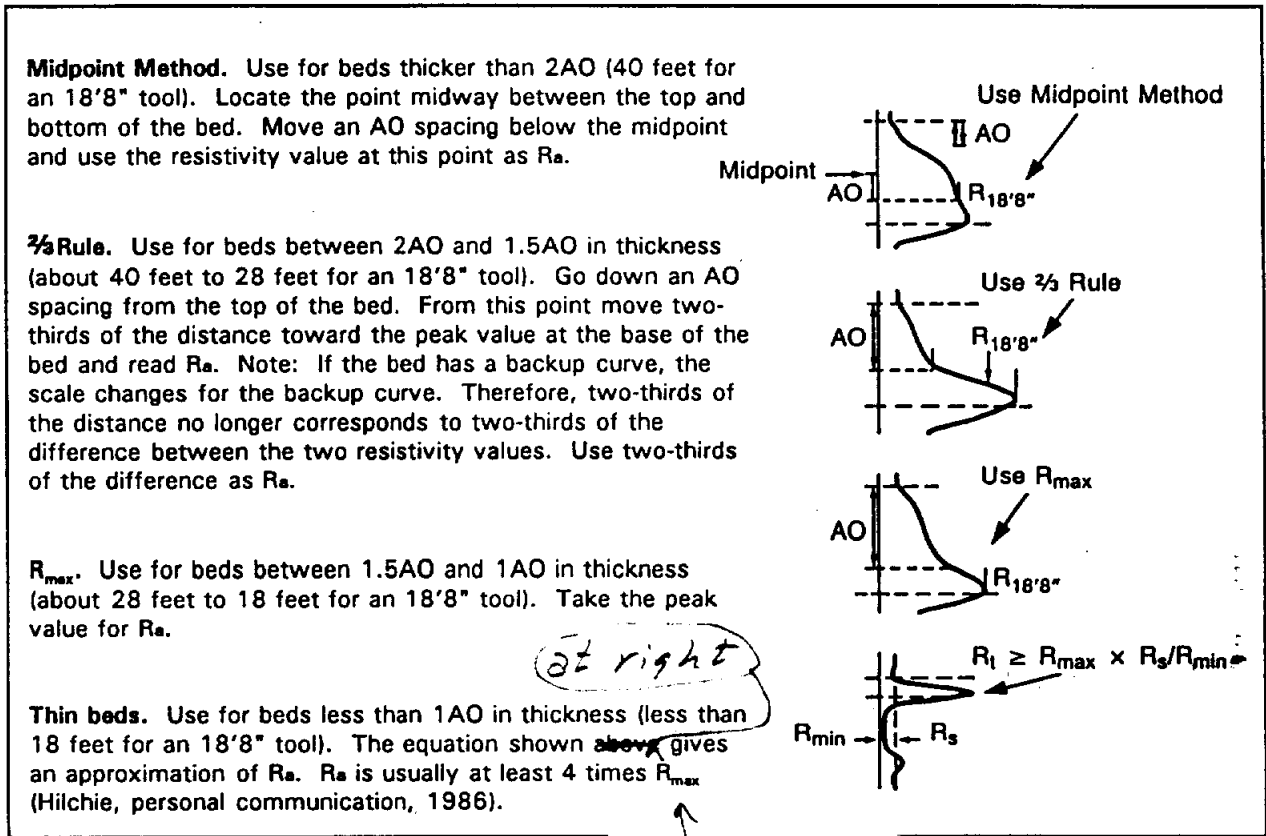
Figure 8-26. Guidelines for picking the lateral resistivity of varying thicknesses when the surrounding beds are homogenous. The AO is 18' 8". R_s is the resistivity of the side bed (Modified from Schl
