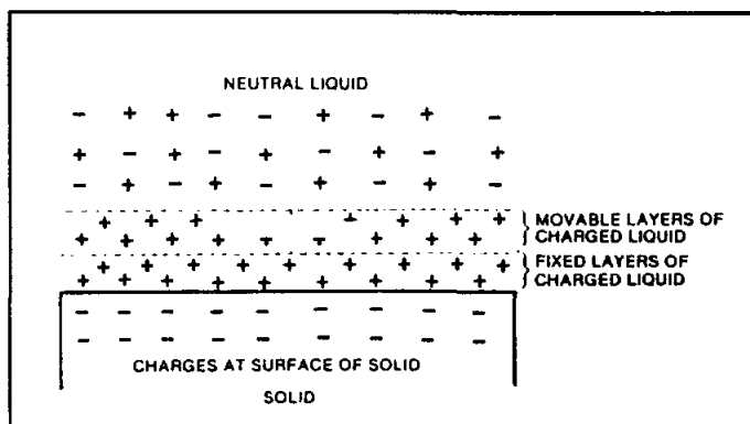
Figure 12-5. The ionic double layer produces an electrokinetic potential when the movable layer is sheared by fluid flow (Modified from Dresser Atlas, 1982).
