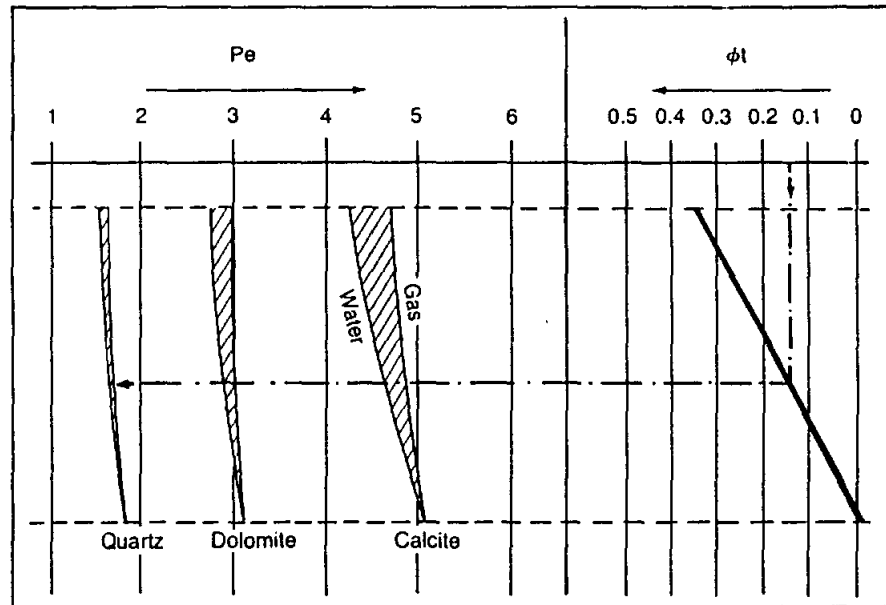
Figure 13-10. Photoelectric absorption factor as a function of total porosity ( \phi_t ) and fluid type (From Dewan, 1983, after Gardner and Dumanoir, 1980).
