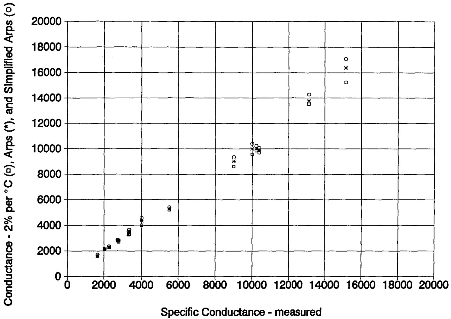
Figure 2-23. Comparison of the accuracy at which three different equations correct specific conductance for temperature changes.
