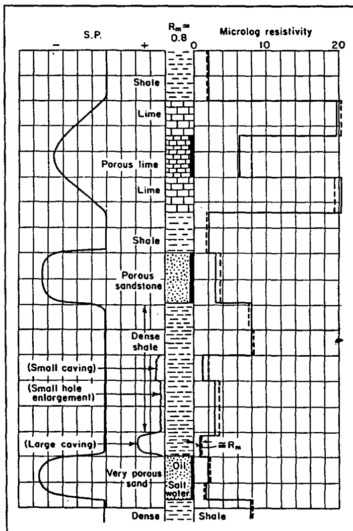
Figure 8-31. Principles of qualitative microlog interpretation (Pirson, 1963, after Schlumberger).
