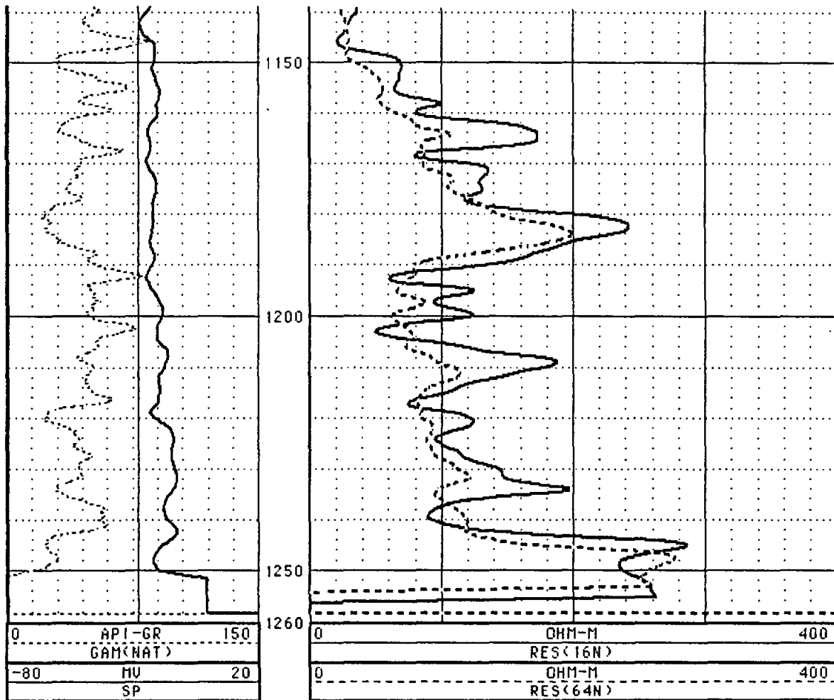
Figure 8-20. This log illustrates several of the problems inherent in interpreting normal curves:
