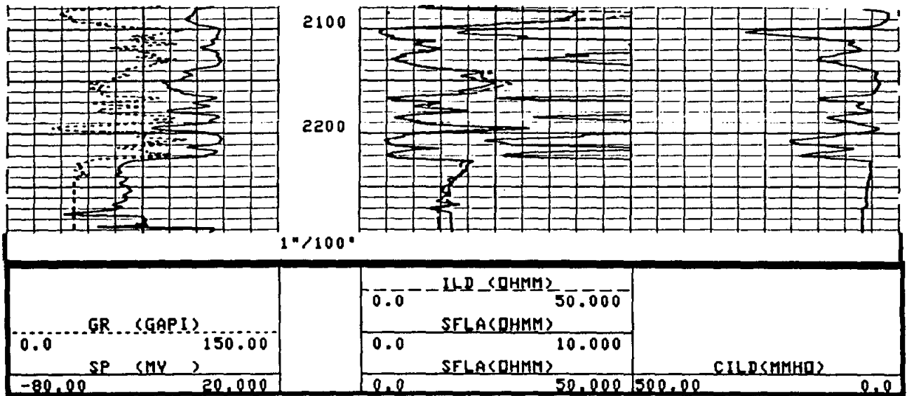
Figure 5-7. A 1 inch per 100 feet depth scale with linear curve scales. The log has been reduced in size to fit this page.
