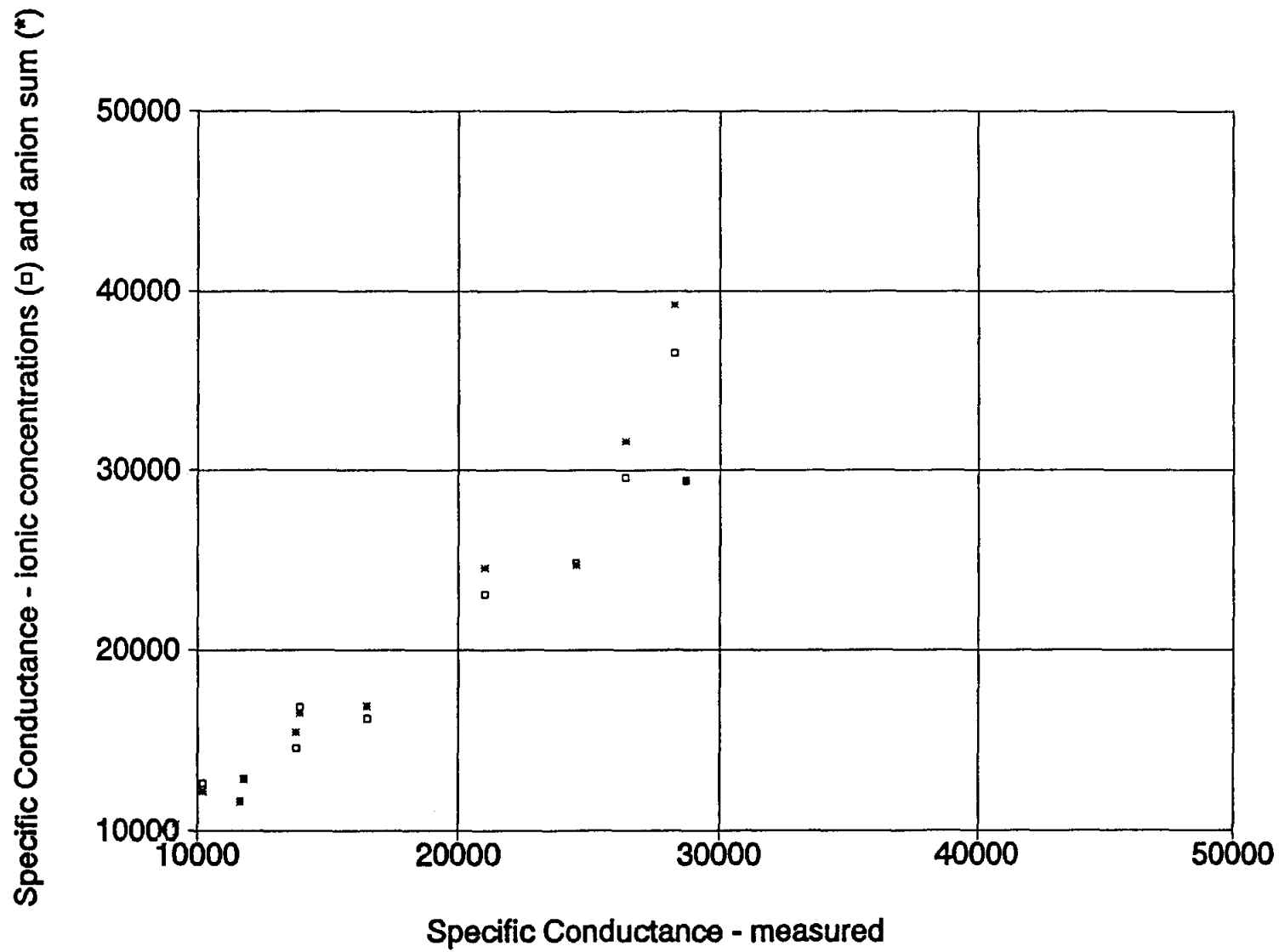
Figure 2-21. A graph of C_{W_{Measured}} versus C_{W_{Ion Conc.}} and C_{W_{Anion Sum}} values ranging between 10,000 and 50,000 \mu\text{mhos/cm} . The data are from water analyses performed by Curtis, Microbiology Services, and Edna Wood Laboratories.
