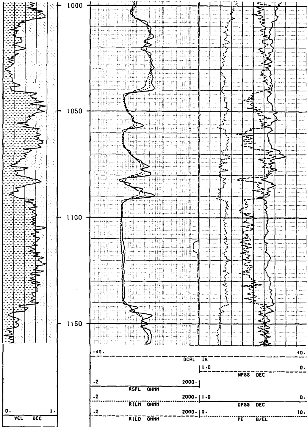
Figure 13-9. Identification of shaly sandstones and shales from density (DP) and neutron (NP) logs. Both curves are calculated on a sandstone matrix (SS) in decimal fractions (DEC), so when the formation is shale-free sandstone the curves overlay. In shaly zones the neutron reads higher than the density, with the density porosity being more accurate. The Pe curve reads 1.8 in sandstones and 1.8 to 2.5 in shaly zones. Dual Induction curves are in Track 2. The lithology column in Track 1 is calculated from the log data. VCL is volume of clay in decimal fractions (DEC). The log is the Gulf Coast Aquifer. Figures 10-10, 11-1, 13-3, and 13-4 provide additional information on this well.
