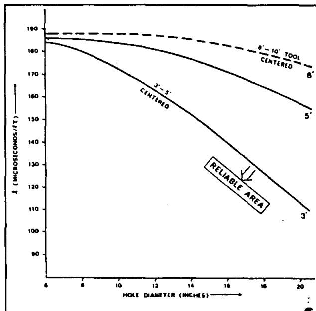
Figure 13-23. Effect of hole size on \Delta t for different transmitter-near receiver spacings (From Goetz et al., 1979, in Serra, 1984).
