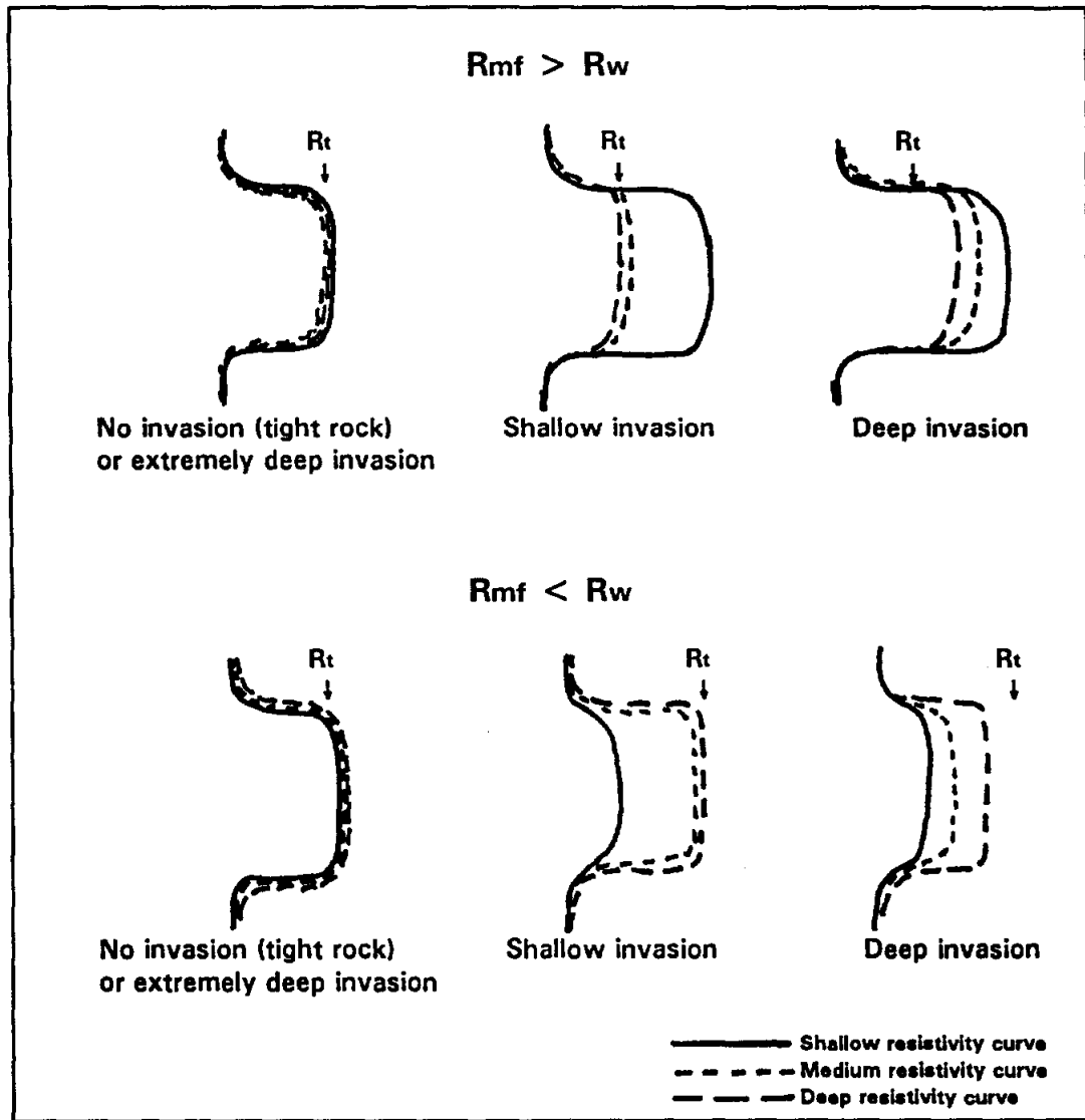
Figure 6-4. Generalized invasion profiles for estimating the depth of invasion and the effect of filtrate on the deep reading resistivity curve. The log patterns represent curves that already have been corrected for all other influences (e.g. R_m , bed thickness, and tool design).
