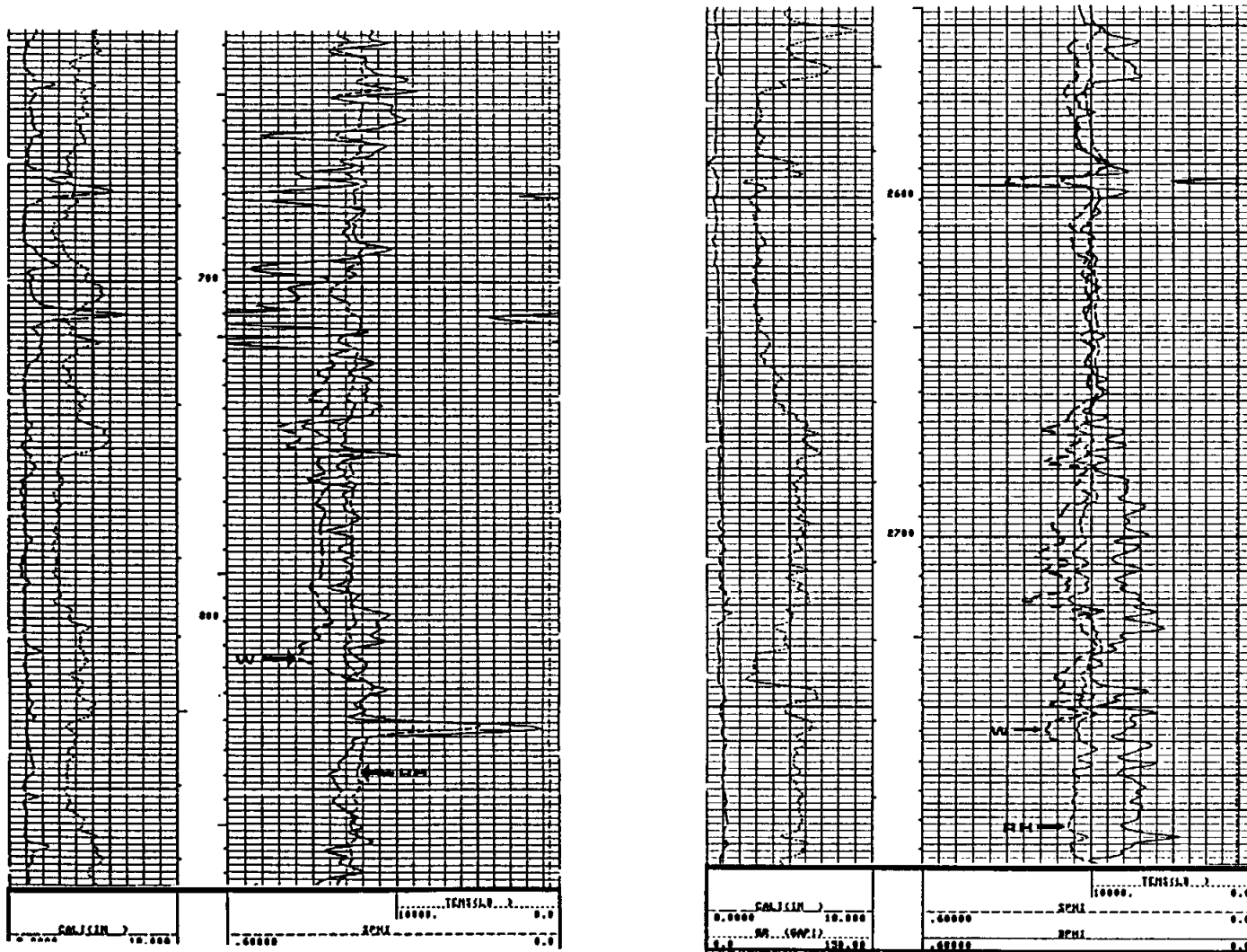
Figure 13-27 a & b. A comparison of the effect of compaction on porosities calculated with the Wyllie (W) and Raymer-Hunt (RH) transforms. At shallow depths (e.g. 750 to 790 feet) the Raymer-Hunt transform adequately corrects for a lack of compaction in the sandstones, while the Wyllie equation yields porosities that are too high. However, at deeper depths (e.g. 2600 to 2650 feet) the sandstones are compacted and both transforms calculate correct porosities. Density porosity is assumed to be true porosity. Figure 13-22 contains additional information on this well.
