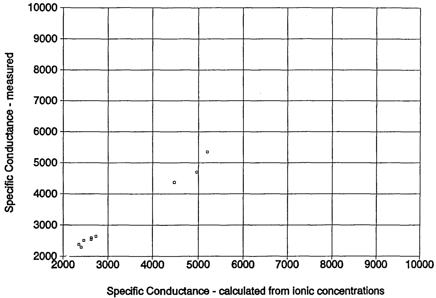
Figure 2-5. A graph of C_{W_{Measured}} versus C_{W_{Ion Conc.}} values ranging between 2,000 and 10,000 \mu\text{mhos/cm} . The data are from water analyses performed by Curtis Laboratories.
