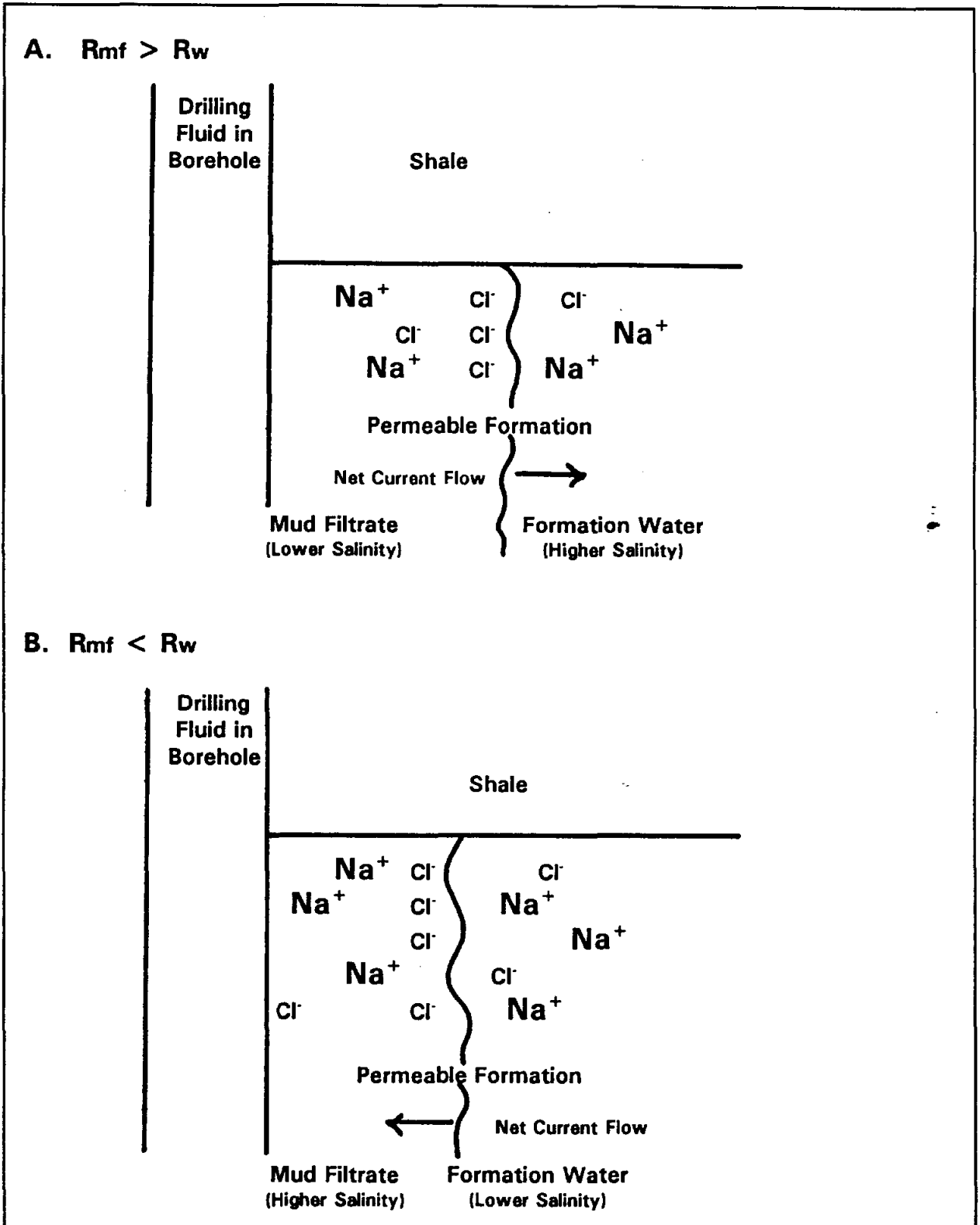
Figure 12-3. Liquid-junction potential generated with a NaCl formation water when R_{mf} is greater than R_w and when R_{mf} is less than R_w .
