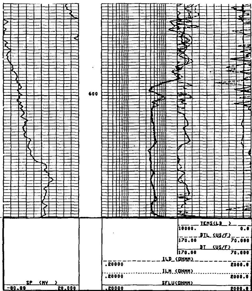
Figure 12-12a. The SP drift is caused by a poor electrical ground of the surface electrode. Tracks 2 and 3 are too cluttered, the sonic curves should be on a separate log. The sonic log has two \Delta t curves (a long and a short space curve), neither of which is working properly. The large rugose borehole (12 1/4 inches bit size and 15 1/2 inches caliper reading) and the uncompacted, unconsolidated nature of the rock precludes accurate sonic porosities. In places, the \Delta t curves are reading nothing but borehole fluid ( \Delta t 189 \mu\text{s}/\text{ft} ). \Delta t peaks greater than 190 \mu\text{s}/\text{ft} are cycle skips.
