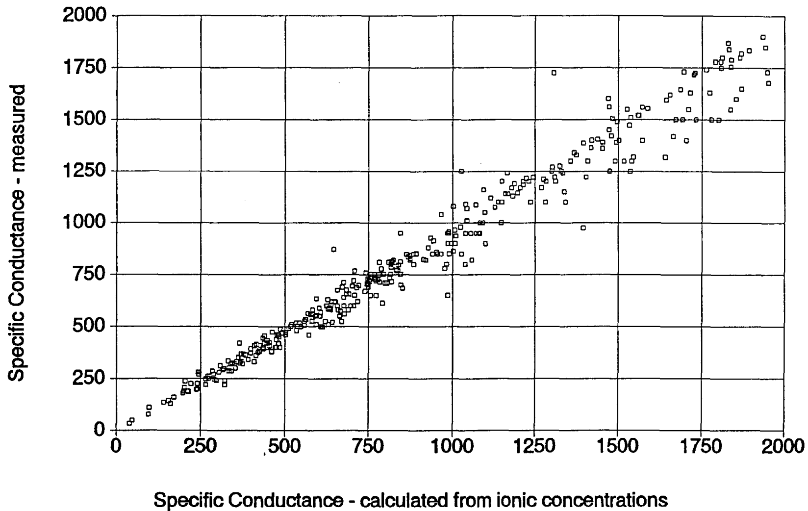
Figure 2-1. A graph of C_{W_{Measured}} versus C_{W_{Ion Conc.}} values ranging between 0 and 2,000 \mu\text{mhos/cm} . The data are from water analyses performed by Curtis, Edna Wood, Microbiology Service, Pope Testing, Texas Testing, and Texas Department of Health Laboratories.
