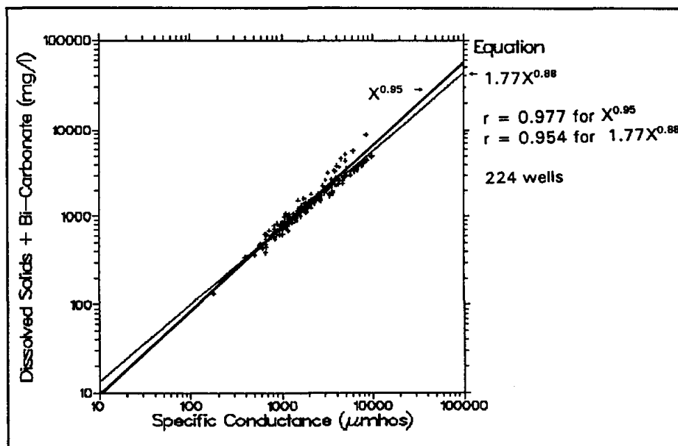
Figure 4-5. Comparison of the line fits generated by equations 4-2 and 4-4. Equation 4-2 gives the more accurate line fit. The plot is all the Jack County water analyses. The criteria used to construct Figures 4-4 and 4-5 are listed on page 73.
