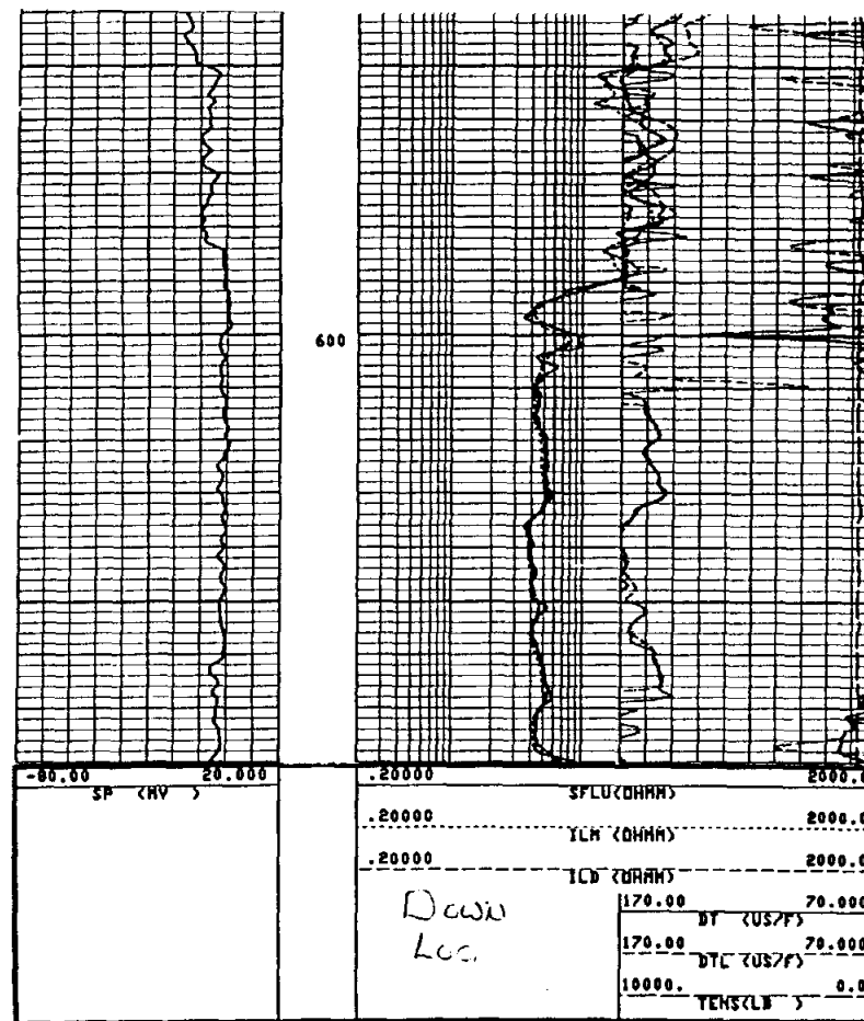
Figure 12-12b. Same log as Figure 12-12a. The SP curve is now working properly after corrosion was removed from the surface electrode. The SP curve does not have large deflections because R_{mf} is very close to R_w . The log was made going into the hole. The log is the Gulf Coast Sandstone Aquifer. The well is the Layne Western, M.U.D. 275 Plant #1, Harris County, Texas. At 700 feet R_m is 9.5 ohm-meters and R_{mf} is 7.6 ohm-meters at 85° F.
