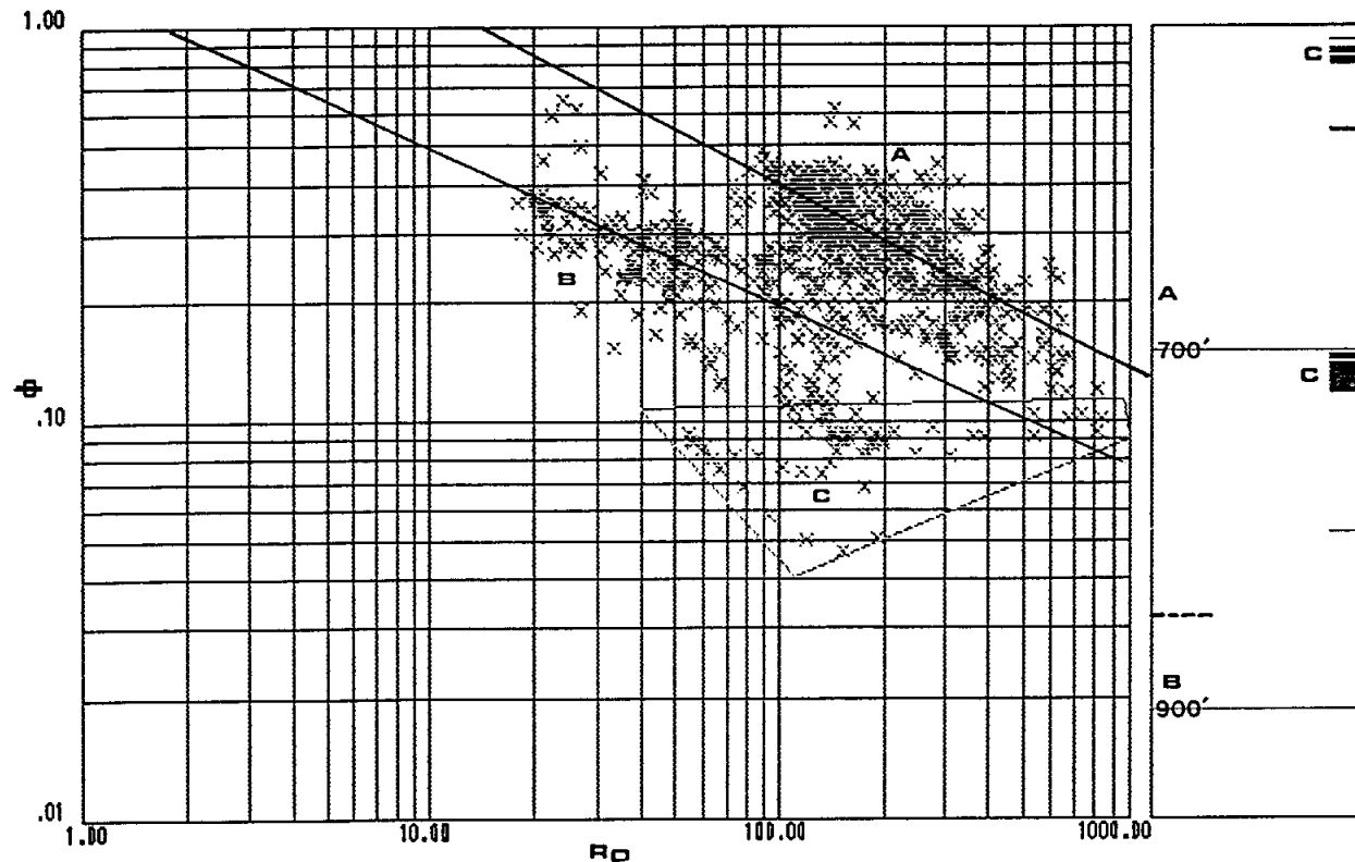
Figure 14-21. Using an R_o -Porosity graph to distinguish waters of different salinities. R_o values are from an averaged spherically focused curve and porosity values are from density-neutron crossplot porosity. The data is from the length of the entire borehole. The data cluster into three groups (A, B, and C), suggesting three different water salinities. Group C, however, is the Georgetown Formation and the Regional Dense Member of the Person Formation. Both are low porosity and very low permeability limestones. Therefore, in the case of group C the cluster represents a different pore structure, rather than a distinct water salinity. R_w values from water samples taken during pump tests confirm two R_w ranges: 16 to 17 ohm-meters for group A and 2 ohm-meters for group B. These R_w 's agree closely with R_w 's estimated from the graph. Group A has an m of A is 2.0 and B has an m of 2.2 (2 was used in the Formation Factor Equation). The column to the right of the graph identifies the intervals in the well that correspond to the groups. The well is in the Edwards Aquifer. It is the Edwards Underground Water District, C-1, New Braunfels, Texas (state well number 68-23-619). Poteet, Collier, and Maclay (1992) contains detailed information on the well.
