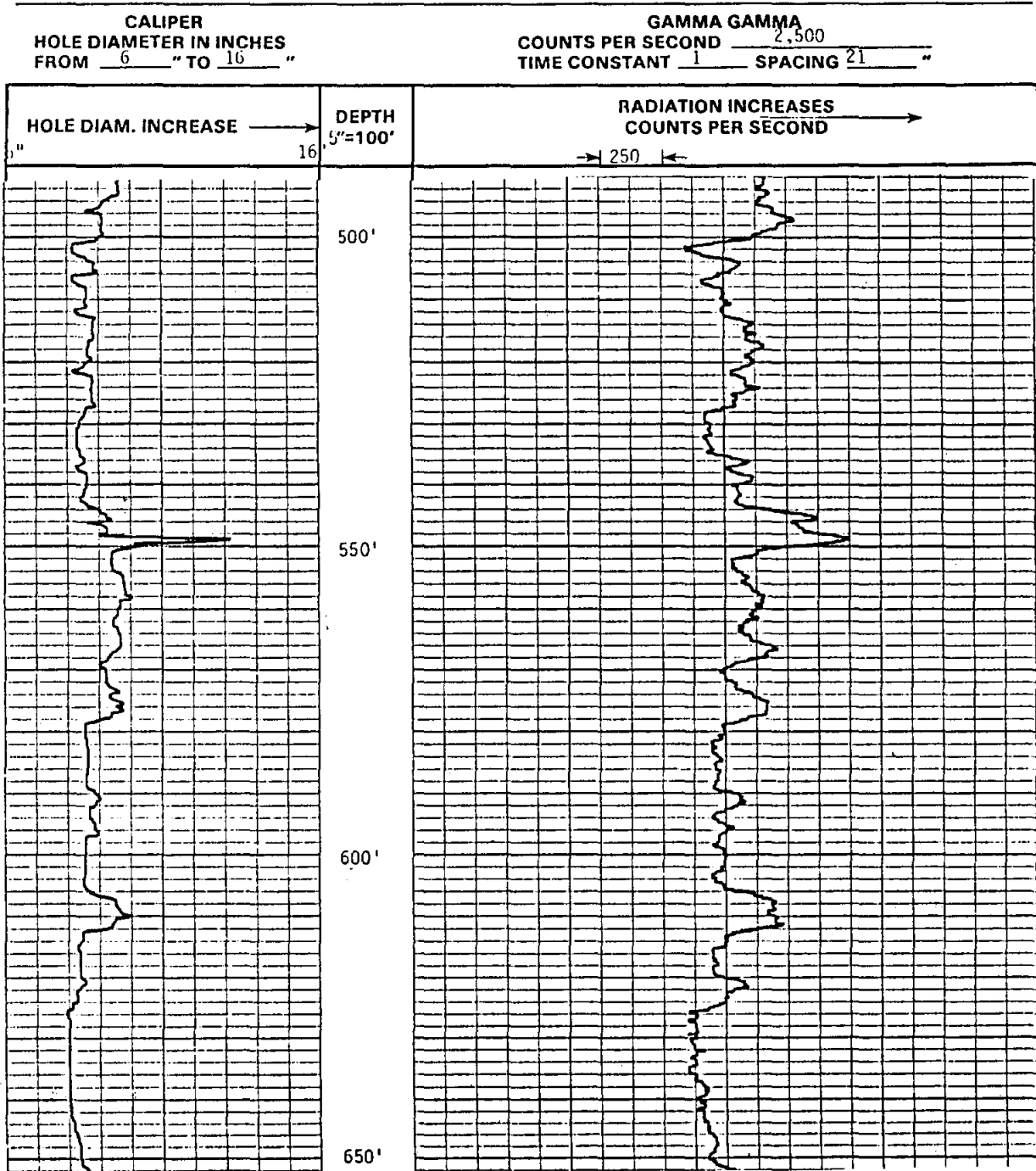
Figure 13-5. Typical slimhole density (gamma gamma) log presentation. Gamma ray count increases to the right, which means that porosity increases to the right. On conventional porosity logs porosity increases to the left. Figure 9-22 contains a conventional density log of this well. The count rate curve shows general trends in porosity, but is not as sensitive as the conventional log. It is hard to correlate the two logs. The slimhole caliper is more sensitive than the conventional caliper.
