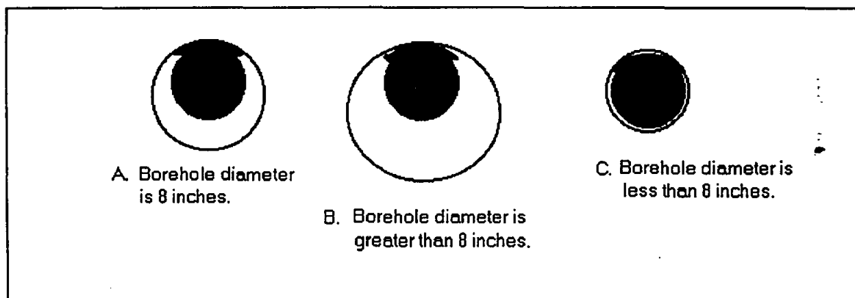
Figure 6-2. How a conventional eccentric tool fits in boreholes of various diameters.
