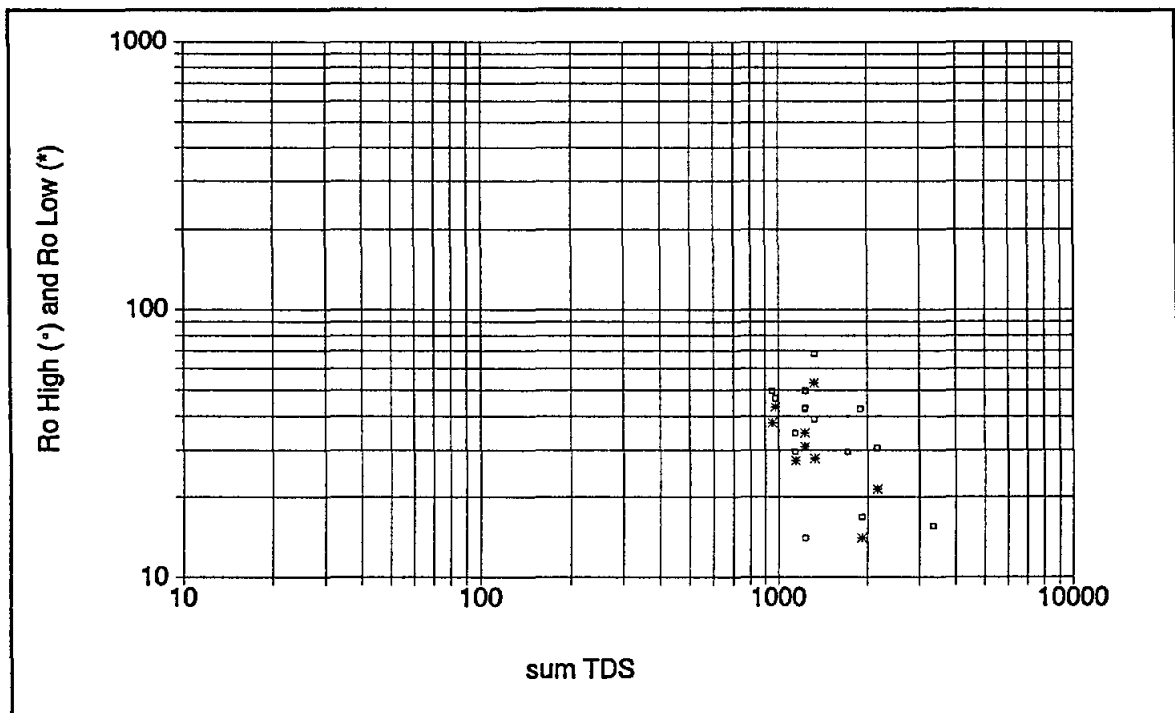
Figure 14-9. Ro_o -TDS graph for Dallas County. Ro_o was normalized to 77° F using site-specific geothermal gradients. The curve fit is no better than that of the Ro -TDS graph (Figure 14-2).
