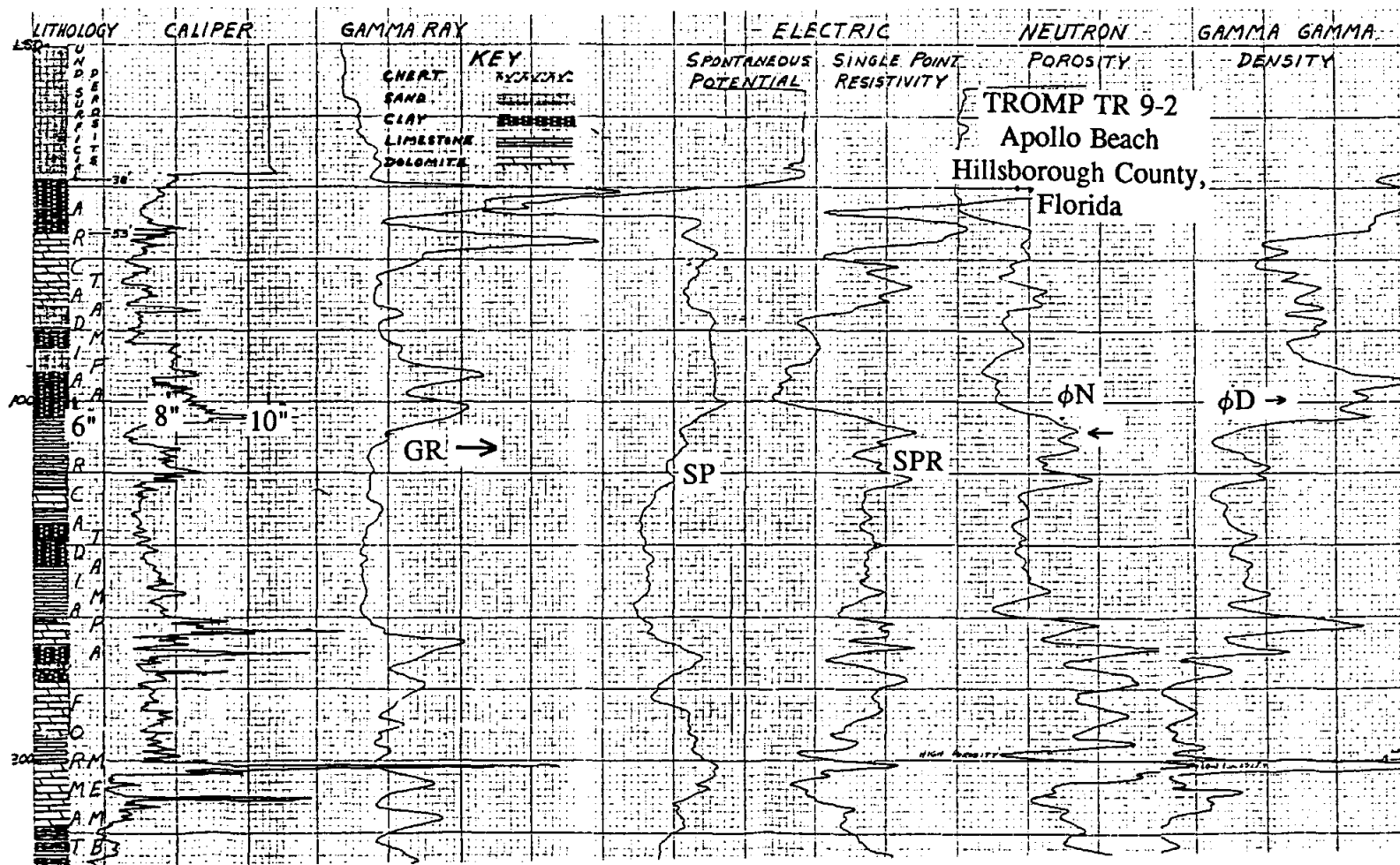
Figure 10-4. Shales with low gamma ray values occur from 46 to 50 feet and at 100 feet. The clay from 46 to 50 feet is kaolinite, which has a very low gamma ray response. The lithology column is based on core descriptions. The gamma ray, neutron, and density curves are scaled in unspecified counts per second. The logs are slimhole tools. The logs are not all on depth. The caliper, gamma ray, and SP curves correlate fairly well. Notice that the caliper is very sensitive to changes in hole size. The lithology is alternating clay, limestone, and dolomite. \phi is the symbol for porosity; an arrow denotes the direction of increasing porosity or gamma ray activity. The well is the TROMP TR 9-2, Apollo Beach, Hillsborough County, Florida.
