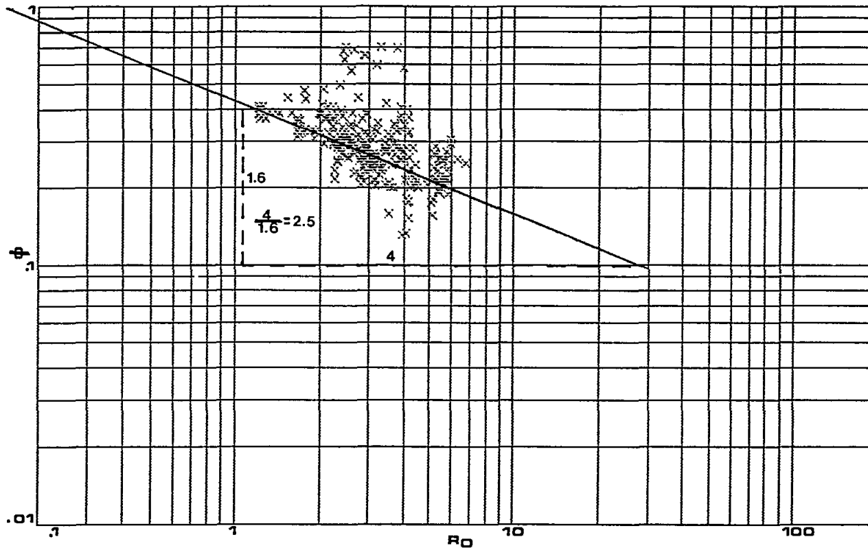
Figure 14-19. Using an Ro-Porosity plot to estimate R_w and m . R_o values are from the deep induction curve and porosity values are density-neutron crossplot porosity. The well is in the Edwards Aquifer and the data is from part of the Kirschberg Evaporite and Dolomitic Members of the Kainer Formation. The data is from an interval that has a constant R_w (1.8 ohm-meters at formation temperature). R_w is from water samples obtained during pump tests. Although there is scatter in the data, a fairly consistent pattern is present. The data is consistent enough to estimate R_w and/or m from the graph. Assuming an a of 1, a line with an R_w of 1.8 ohm-meters was fitted to the data. This line yields an m of 2.5, not an unreasonable value in a vuggy-moldic carbonate. However, an m of 2 was used in the Formation Factor Equation method and it gave accurate R_w 's (Plate 5). Not knowing R_w , a best fit line through the data would yield an R_w close to the actual value. The well is the Edwards Underground Water District, A-1. Figure 13-32 and Plate 5 contain additional information on this well.
