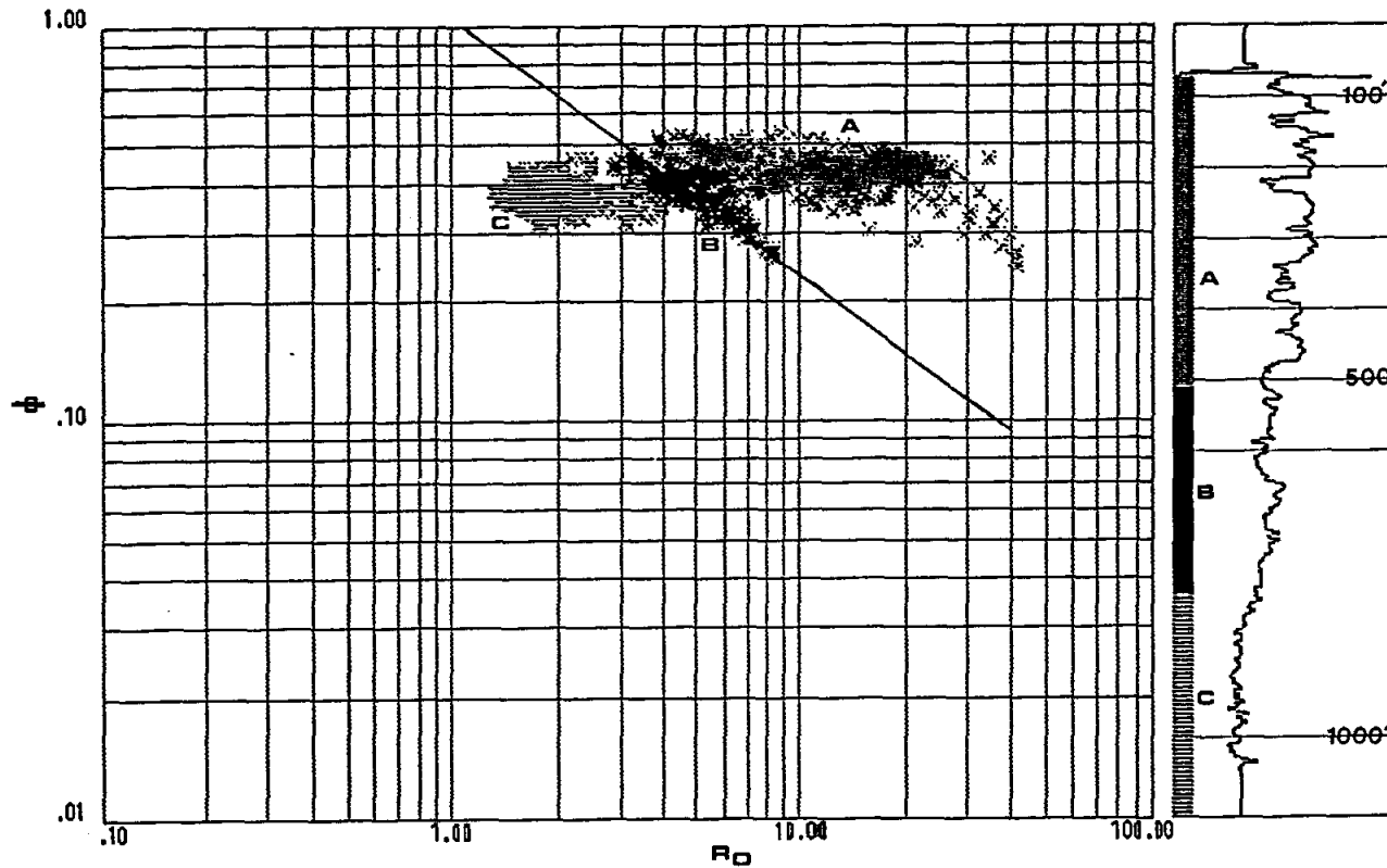
Figure 14-20. Using an Ro-Porosity graph to distinguish waters of different salinities. R_o values are from the deep induction curve and porosity values are from density-neutron crossplot porosity. The data is from the length of the entire borehole. The data cluster into three groups (A, B, and C), suggesting three different water salinities. R_w values from water samples taken during pump tests confirm three R_w ranges. The scatter in groups A and C is such that it is impossible to estimate either m or R_w . A good line fit can be drawn through group B, yielding an R_w that is too high (about 1.05 ohm-meters versus an actual R_w of about 0.54 ohm-meters at formation temperature) and an m of 1.3. This m is consistent with m 's of 1.1 and 1.4 estimated from the Formation Factor-Porosity graph (Figure 14-13). The column to the right of the graph contains the deep induction curve and a few 100 foot depth markers. It also identifies the intervals in the well that correspond to the three clusters of data. The well is the TWDB PUB Test Site F, Cameron County, Texas. Refer to Figure 13-12 and Plates 1 to 4 for additional information on this well.
