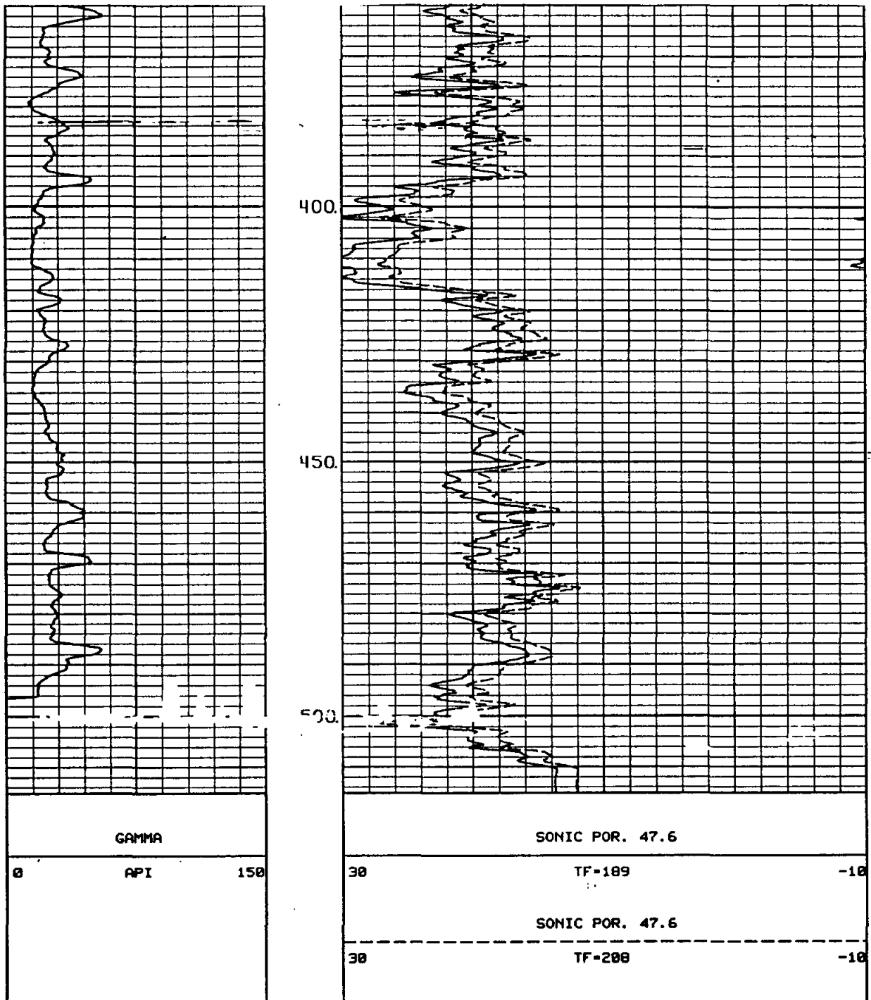
Figure 13-24. Comparison of sonic porosities calculated with the \Delta t 's of fresh and saline water. The salt water value for \Delta t ( 189 \mu\text{sec}/\text{ft} ), which is commonly used in oilfield logging, yields porosity values that are approximately 3 pu too large when the pore water is fresh. The \Delta t used for fresh water ( 208 \mu\text{sec}/\text{ft} ) is too high. 205 \mu\text{sec}/\text{ft} is a better value. However, there is little difference between porosity values calculated with the two. Porosities were calculated with the Wyllie time average equation. Bit size is 6 inches. The borehole fluid is fresh formation water. The aquifer is a Cretaceous limestone in South Texas.
