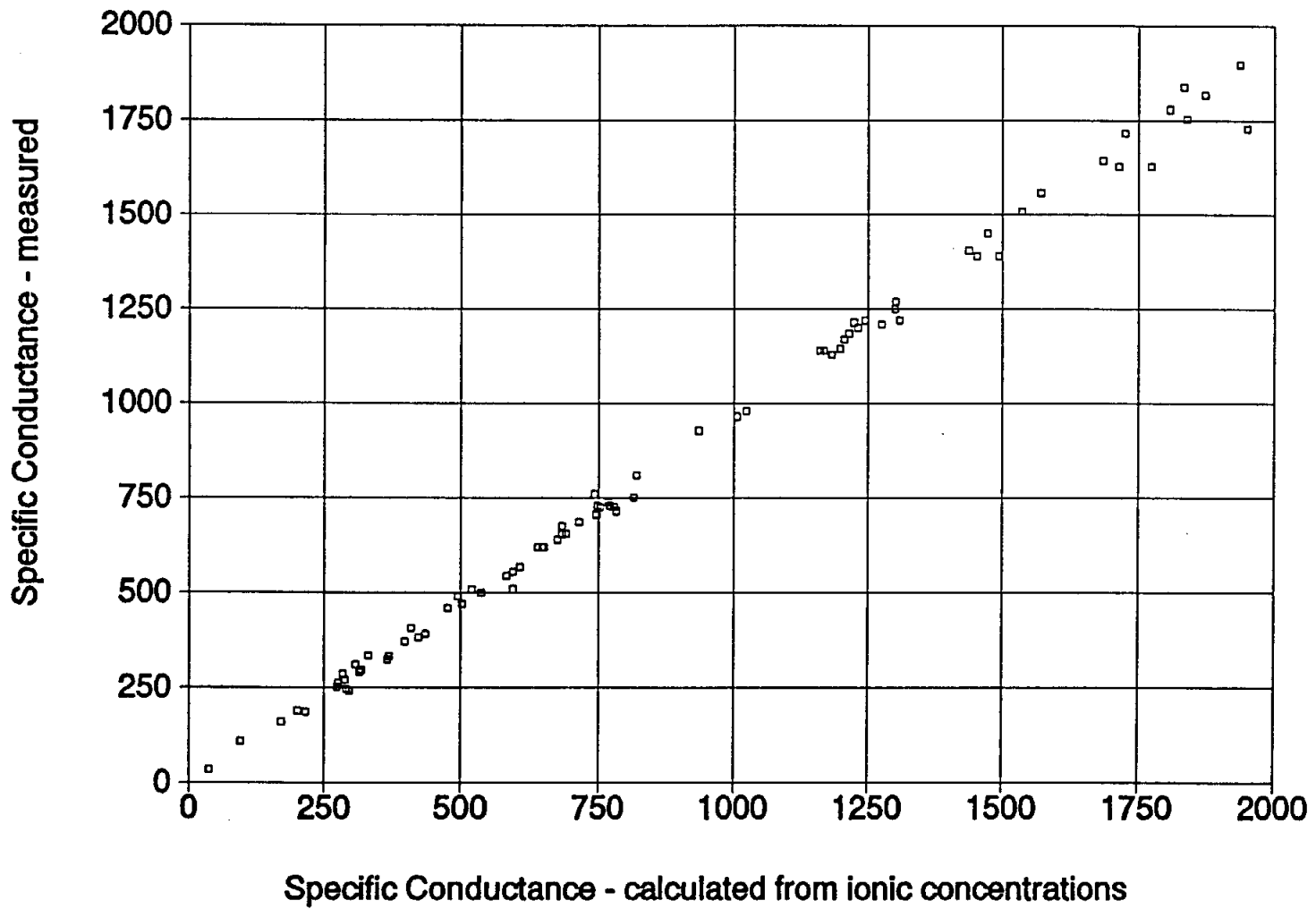
Figure 2-8. A graph of C_{w, \text{Measured}} versus C_{w, \text{Ion Conc.}} values ranging between 0 and 2,000 \mu\text{mhos/cm} . The data are from water analyses performed by Microbiology Service Laboratories.
