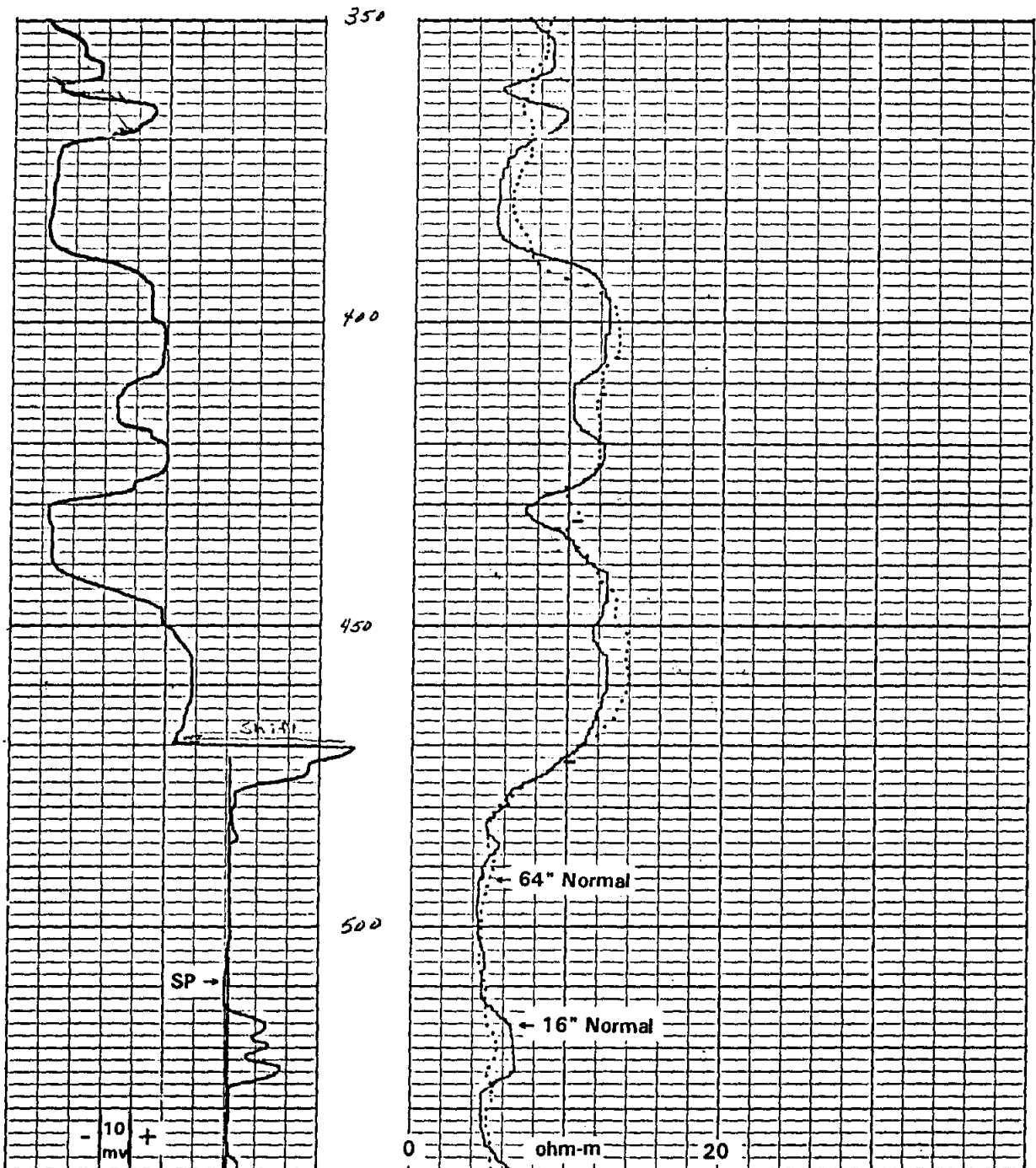
u- Figure 8-18. This log is a slimhole 16" normal, 64" normal, and SP. A comparison with the deep induction-guard curves run in the same borehole (Figure 8-19) confirms that normal curves work well in high porosity formations thicker than 20 feet. The 64" normal agrees very well with the deep induction even without borehole corrections to either curve. The 16" normal, with its deeper depth of investigation, reads higher than the guard. Another explanation for the difference is that the amount and depth of mud filtrate invasion has changed between logging runs. (The normal curves were run while the well was being drilled, 13 days before the induction log.) See Figures 8-19 and 12-7 for further details on this well.
