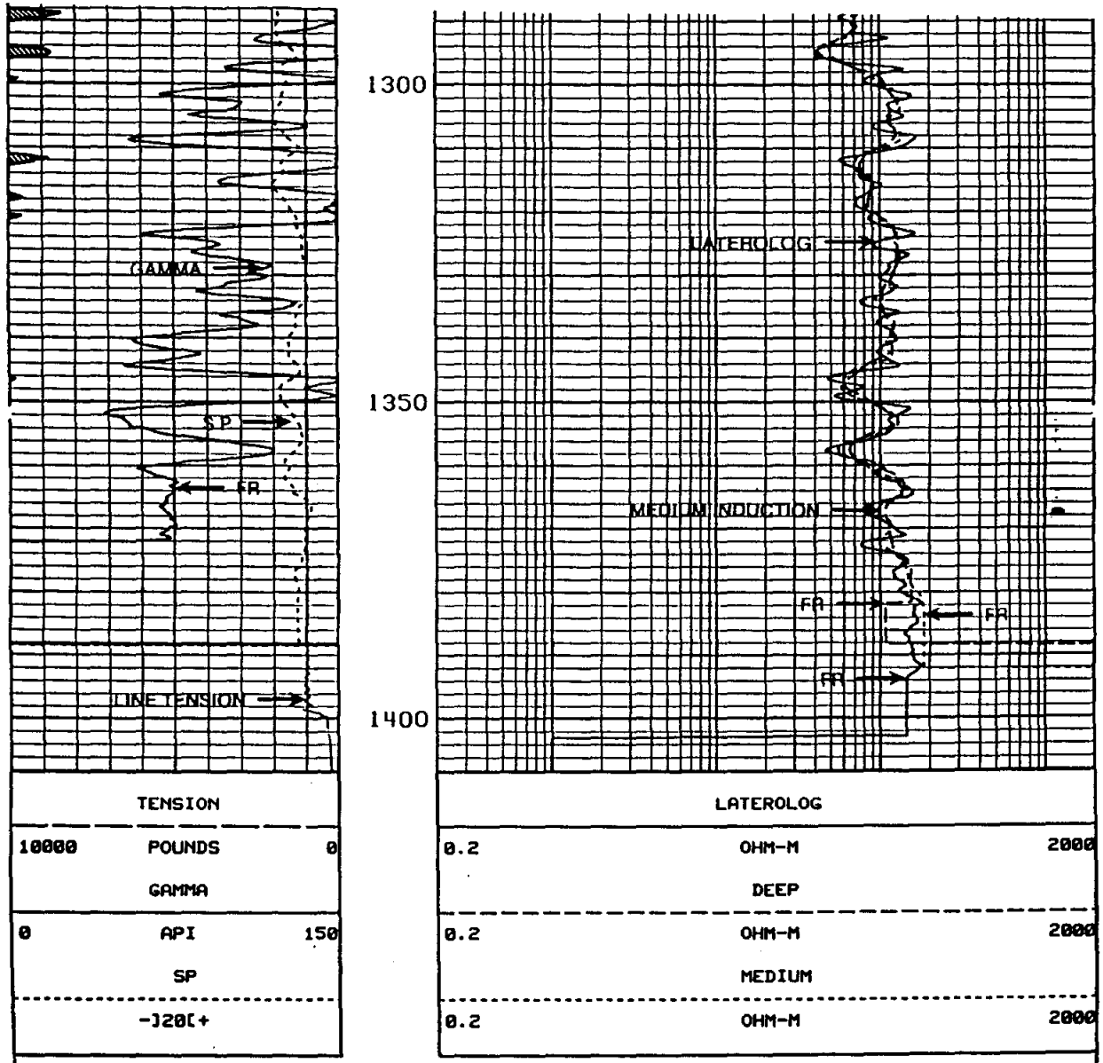
Figure 5-9. A 5 inch per 100 feet depth scale with logarithmic resistivity curves in Tracks 2 and 3. FR denotes the first reading of each curve. The gamma ray curve goes off scale at 1312 feet and wraps around to start over again on the left side of Track 1. The wrap-around scale for the gamma ray curve should be in the curve scale but it was left off. The log has been reduced in size to fit the page. For further details on this log see Figure 5-10.
