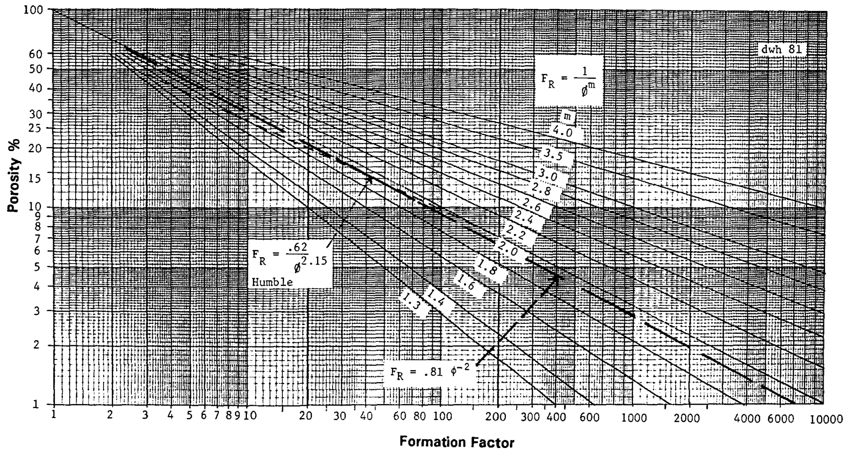
Figure 14-15. Formation Factor versus Porosity and m (modified from Hilchie, 1982). The graph is used to calculate F , given m and porosity.
