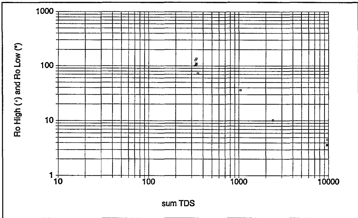
Figure 14-8. Ro_o -TDS graph for Harris County. Ro_o has been normalized to 77° F using site-specific geothermal gradients. The curve fit is no better than that of the Ro -TDS graph (Figure 14-1).
