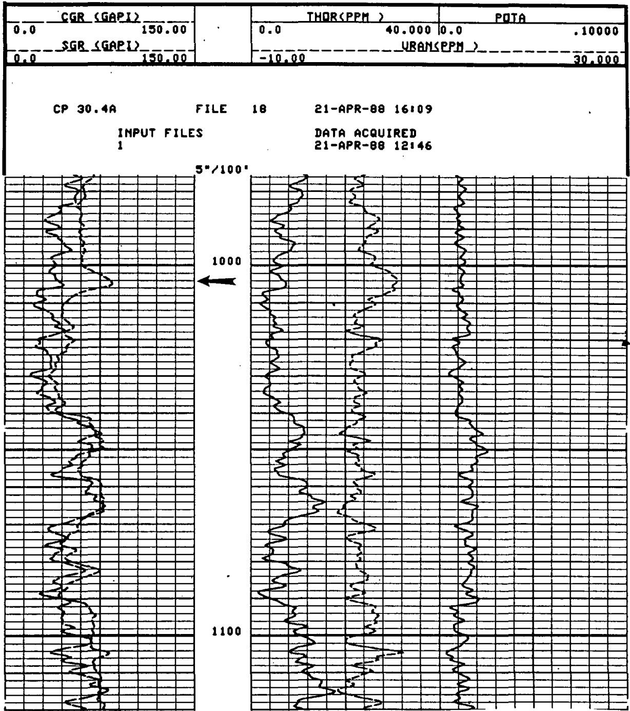
Figure 10-10. Typical spectral gamma ray log. Track 1 has both total gamma ray activity (SGR) and a gamma ray curve minus the uranium component (CGR). Tracks 2 and 3 have the individual curves. Thorium and uranium are scaled in parts per million (ppm) and potassium is scaled in weight percent. The gamma ray kick at 1004 feet (arrow) is due to uranium. The sandstone at 1006 to 1040 feet is slightly shaly. The shale below this sandstone has fairly typical radioactivities: thorium about 12 ppm, uranium 2 to 3 ppm, and potassium about 2 percent. The bit size is 9 7/8 inches and the borehole fluid is a 9 lb/gal native gel. The log is an interval in the Gulf Coast Aquifer. The well is the Alsay, NW Harris County MUD 21 and 22 #2. Figures 11-1, 13-3, 13-4, and 13-9 are from the same well.
