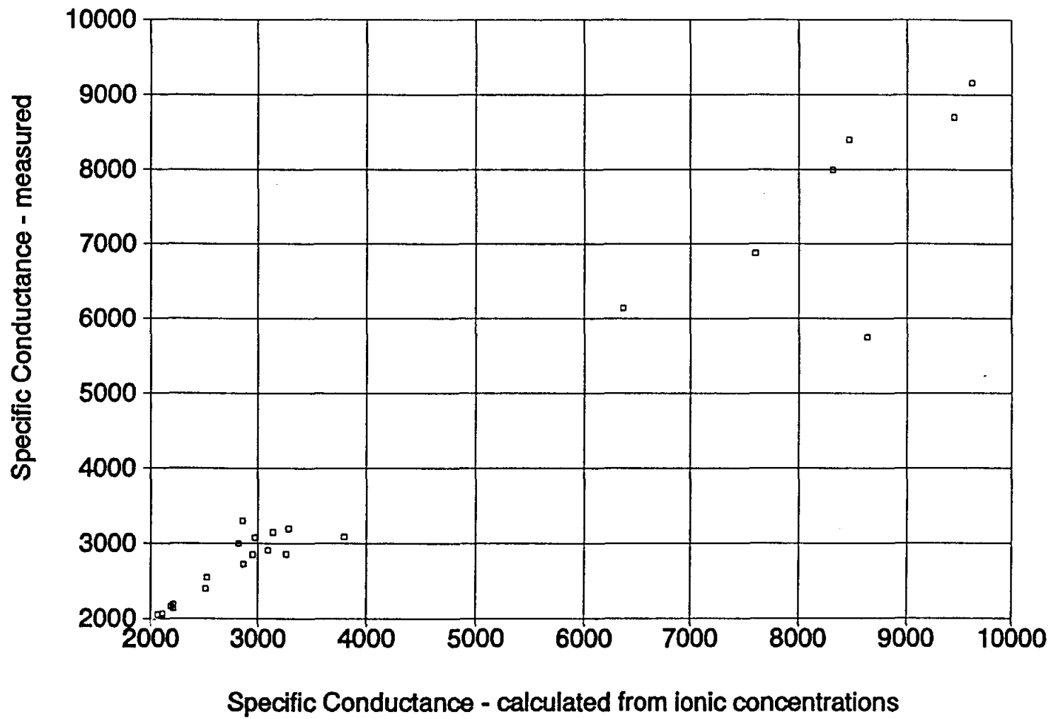
Figure 2-9. A graph of C_{W_{\text{Measured}}} versus C_{W_{\text{Ion Conc.}}} values ranging between 2,000 and 10,000 \mu\text{mhos/cm} . The data are from water analyses performed by Microbiology Service Laboratories.
