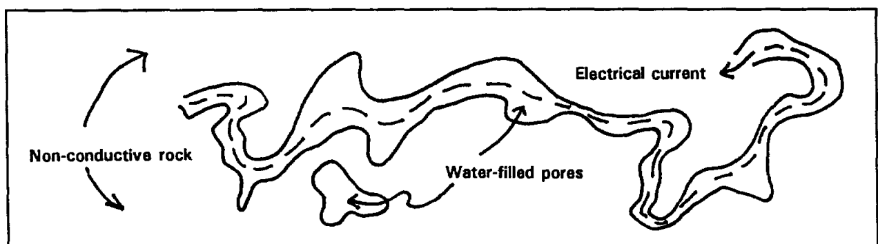
Figure 8-2. This figure depicts the heterogeneous, tortuous pore system that is often present in carbonates. The formation water still conducts all of the electrical current, but the route the current follows is longer and therefore resistivity is higher than in an intergranular pore system.
