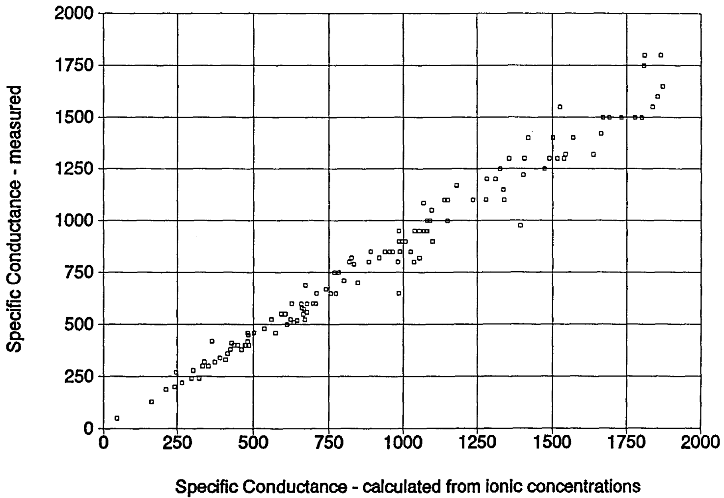
Figure 2-10. A graph of C_{W, \text{Measured}} versus C_{W, \text{Ion Conc.}} values ranging between 0 and 2,000 \mu\text{mhos/cm} . The data are from water analyses performed by Pope Testing Laboratories.
