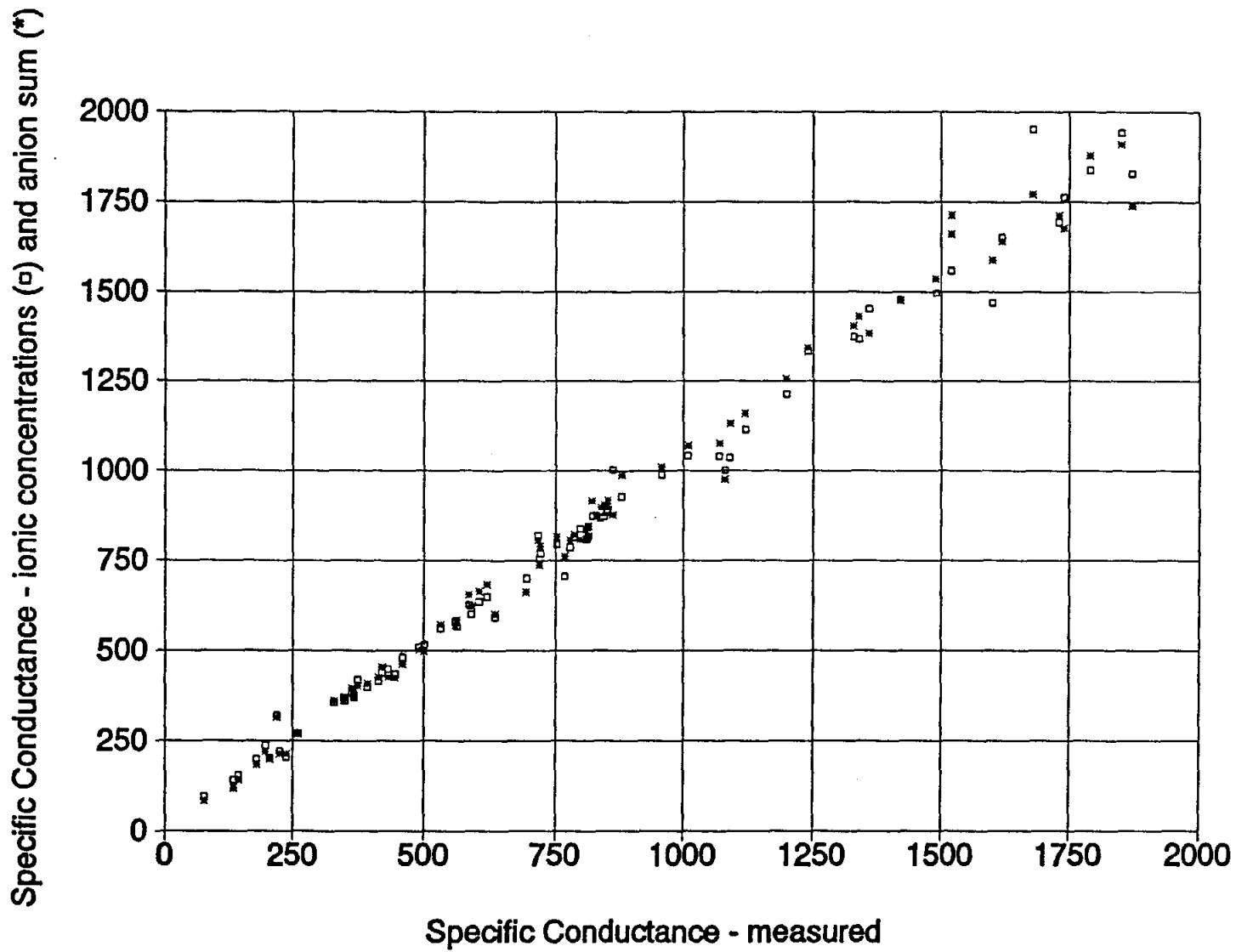
Figure 2-19. A graph of C_{W\text{Measured}} versus C_{W\text{Ion Conc.}} and C_{W\text{Anion Sum}} values ranging between 0 and 2,000 \mu\text{mhos/cm} . The data are from water analyses performed by Edna Wood Laboratories.
