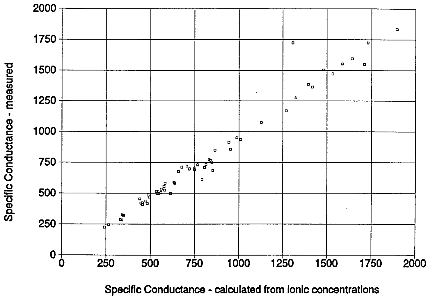
Figure 2-4. A graph of C_{W, \text{Measured}} versus C_{W, \text{Ion Conc.}} values ranging between 0 and 2,000 \mu\text{mhos/cm} . The data are from water analyses performed by Curtis Laboratories.
