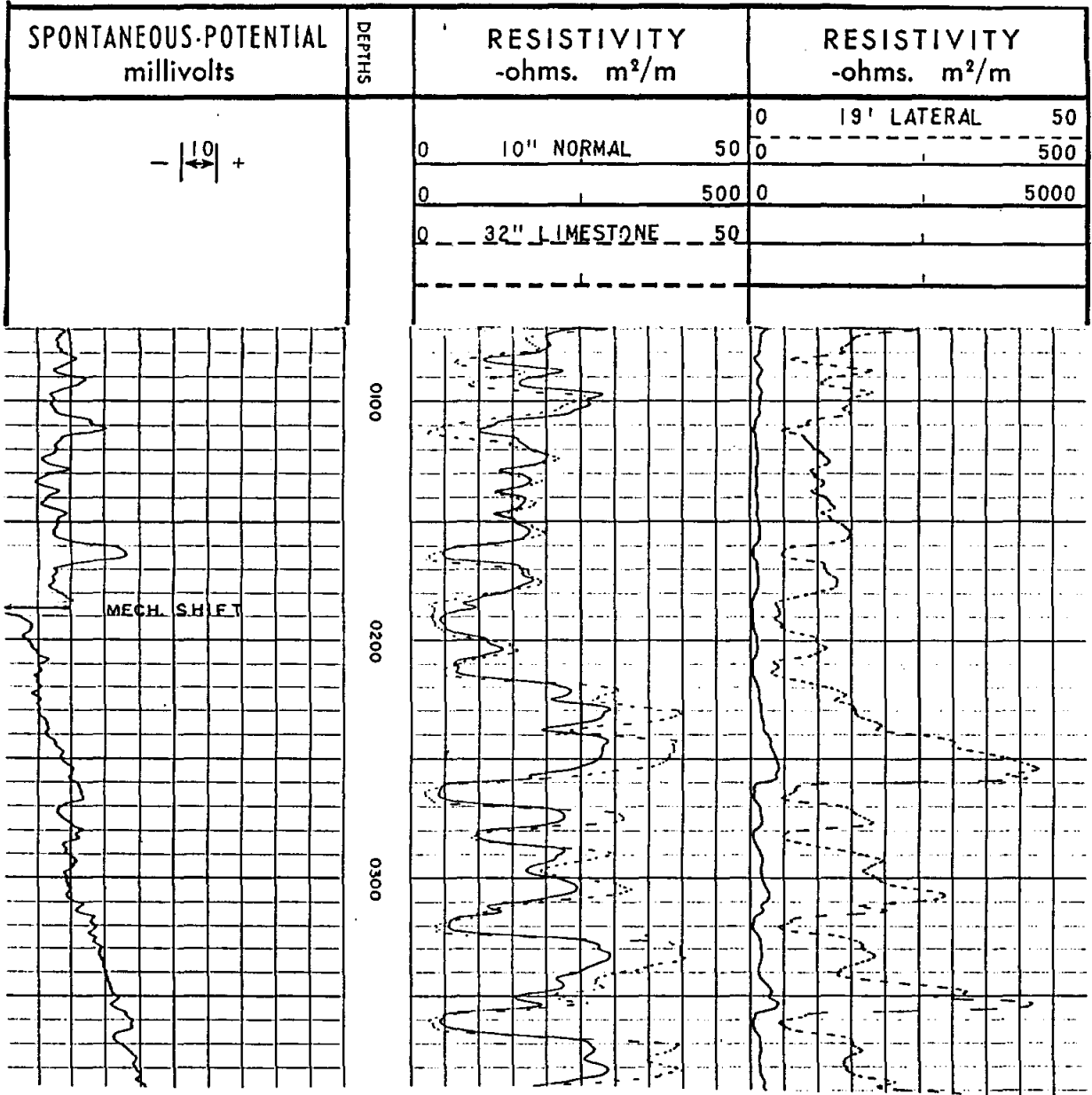
Figure 8-28. Example of a limestone lateral in a water well. The formations are not low porosity, so the limestone and 10 inch normal curves are very similar. The well is the Layne Texas, Phelps Dodge #4, El Paso County, Texas. Bit size is 7 1/4 inches. R m is 6.6 ohm-meters at 76° F. Bottom hole temperature was not recorded.
