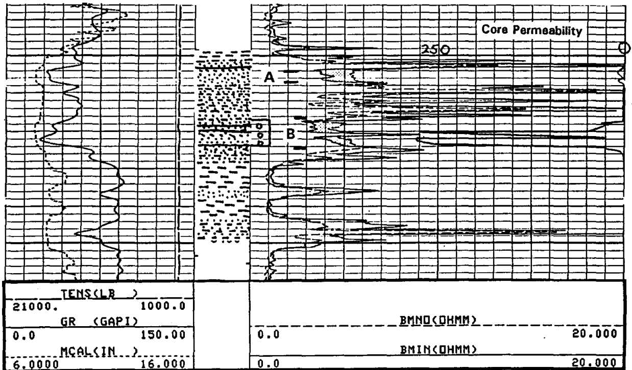
Figure 8-32. Two intervals with similar positive microlog separation but very different permeabilities. Zone A has core permeabilities from 2.5 md to 10 md. Zone B, which has a microlog character similar to Zone A, has permeabilities ranging from 20 md to 342 md, with three feet having 245 to 340 md. The core permeabilities are plotted in Track 3. A lithologic description of the core is in the depth column. The letter "B" on the scale refers to a particular version of Schlumberger's microlog. The log is an oil well in the Paluxy sandstone in East Texas. The well is producing from Zone B. The bit size is 7 7/8 inches. R_m is 1.13 ohm-meters and R_{mf} is 1 ohm-meter at formation temperature (167° F).
