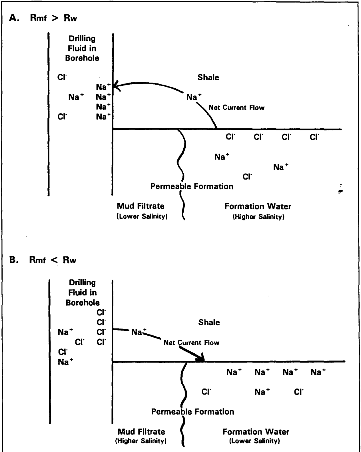
Figure 12-2. Shale membrane potential generated with a NaCl formation water, when R_{mf} is greater than R_w and when R_{mf} is less than R_w .
