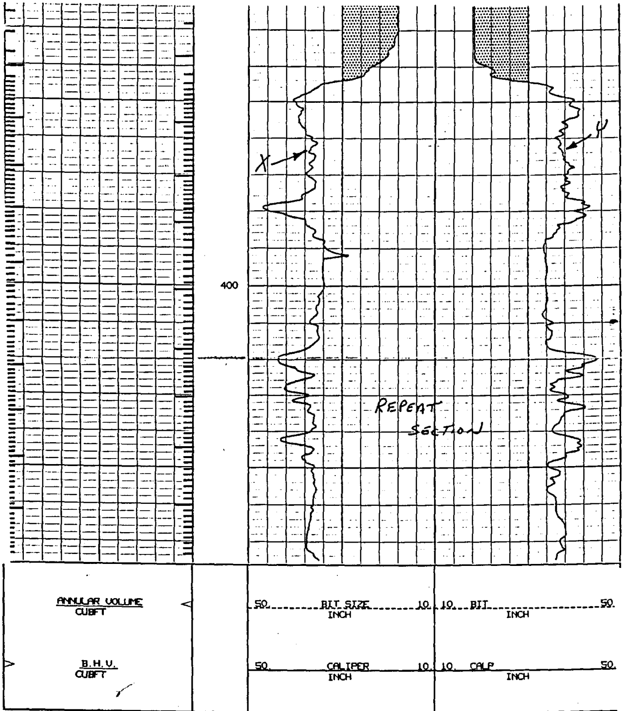
Figure 11-2. Welex X-Y caliper. The casing extends to 340 feet and its diameter is 18 inches. The hole was underreamed from 340 feet to T.D. with a 30 inch bit. Bit size is represented by a dashed line (barely visible on the 30 inch lines). The entire borehole has washouts. Two caliper measurements perpendicular to each other do a much better job of characterizing the borehole diameter. Along the left margin of Track 1 is the integrated borehole volume (B.H.V.). The annular volume for a particular casing size is noted along the right side of Track 1. Unfortunately, the casing size used in the calculation is not specified on the log. Each tic mark is one cubic foot.
