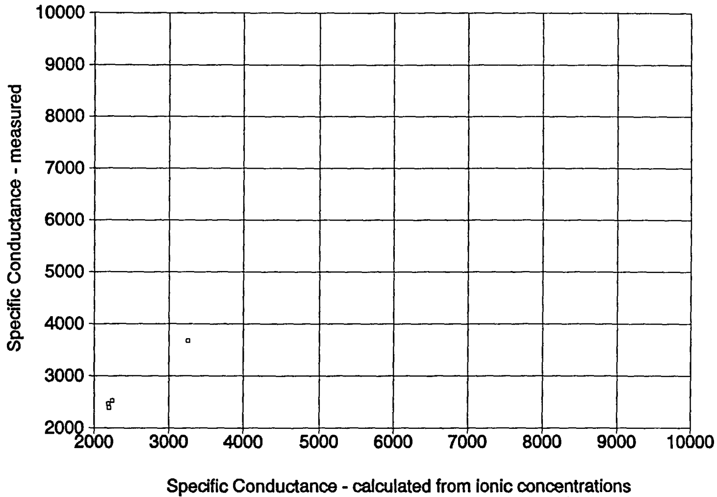
Figure 2-14. A graph of C_{w, \text{Measured}} versus C_{w, \text{Ion Conc.}} values ranging between 2,000 and 10,000 \mu\text{mhos/cm} . The data are from water analyses performed by Texas Department of Health Laboratories.
