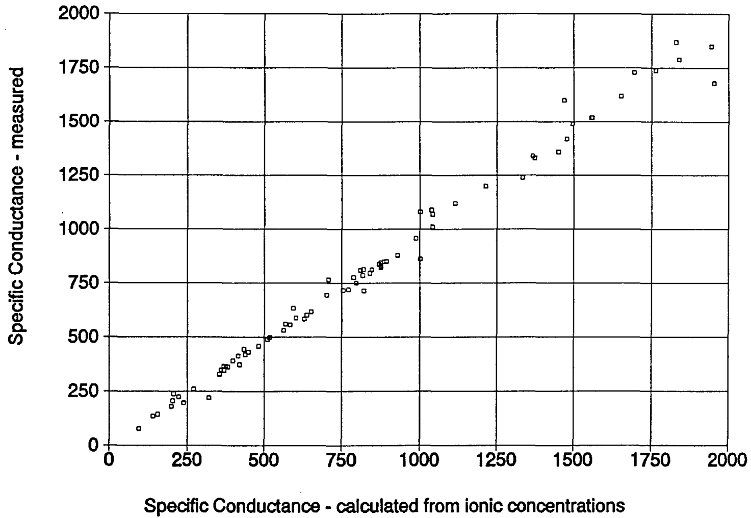
Figure 2-6. A graph of C_{w, \text{Measured}} versus C_{w, \text{Ion Conc.}} values ranging between 0 and 2,000 \mu\text{mhos/cm} . The data are from water analyses performed by Edna Wood Laboratories.
