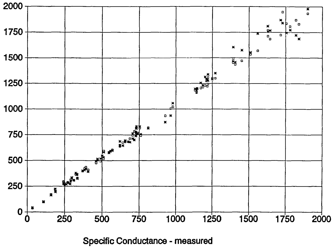
Figure 2-17. A graph of C_{w, \text{Measured}} versus C_{w, \text{Ion Conc.}} and C_{w, \text{Anion Sum}} values ranging between 0 and 2,000 \mu\text{mhos/cm} . The data are from water analyses performed by Microbiology Service Laboratories.
