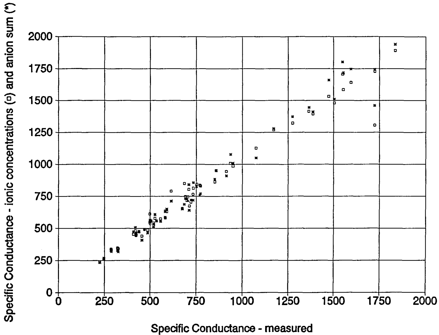
Figure 2-15. A graph of C_{w, \text{Measured}} versus C_{w, \text{Ion Conc.}} and C_{w, \text{Anion Sum}} values ranging between 0 and 2,000 \mu\text{mhos/cm} . The data are from water analyses performed by Curtis Laboratories.
