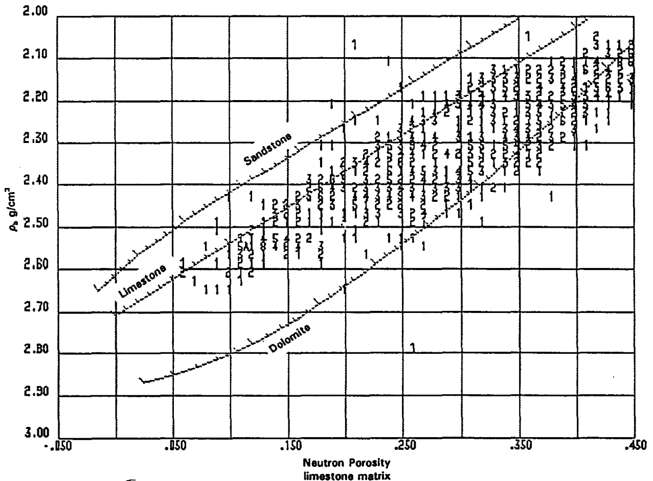
Figure 13-32. A density-neutron crossplot. The sampling interval is 0.5 feet. The numbers on the graph denote the occurrences of a particular point. The lithology is predominately limestone, dolomite, or a mixture of the two. Minor amounts of shale and chert are also present. Points that plot at isolated extremes are either other mineralogies or erroneous measurements. The well is the Edwards Aquifer. Figures 9-22, 13-5, 13-8, 13-28, and 13-33 provide additional data on this well.
