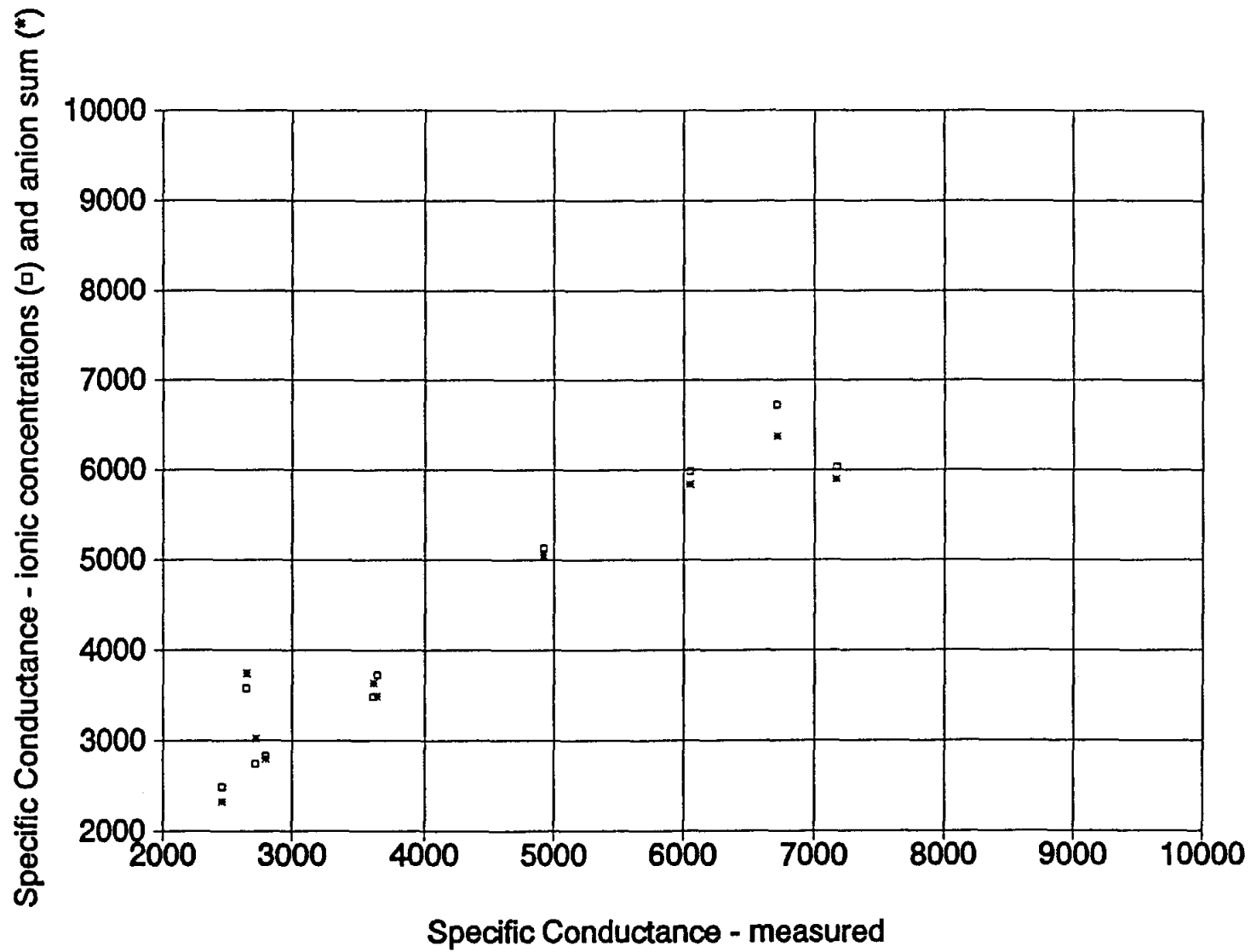
Figure 2-20. A graph of C_{w, \text{Measured}} versus C_{w, \text{Ion Conc.}} and C_{w, \text{Anion Sum}} values ranging between 2,000 and 10,000 \mu\text{mhos/cm} . The data are from water analyses performed by Edna Wood Laboratories.
