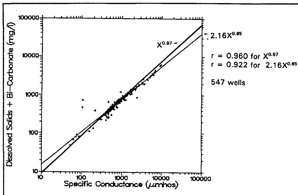
Figure 4-4. Comparison of the line fits generated by equations 4-2 and 4-4. Equation 4-2 gives the more accurate line fit. Dissolved solids includes 100 percent of the bicarbonate value. Most of the specific conductance values are diluted conductance. The plot is all the Harris County water analyses in the Texas Water Development Board Ground-Water Data Base.
