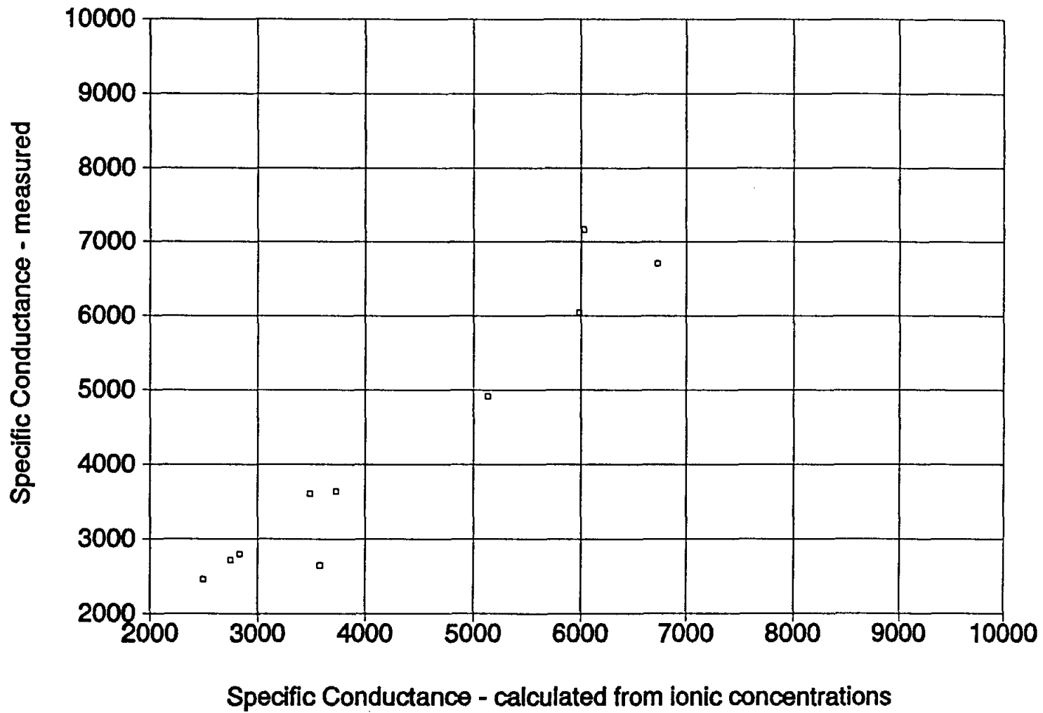
Figure 2-7. A graph of C_{W\text{Measured}} versus C_{W\text{Ion Conc.}} values ranging between 2,000 and 10,000 \mu\text{mhos/cm} . The data are from water analyses performed by Edna Wood Laboratories.
