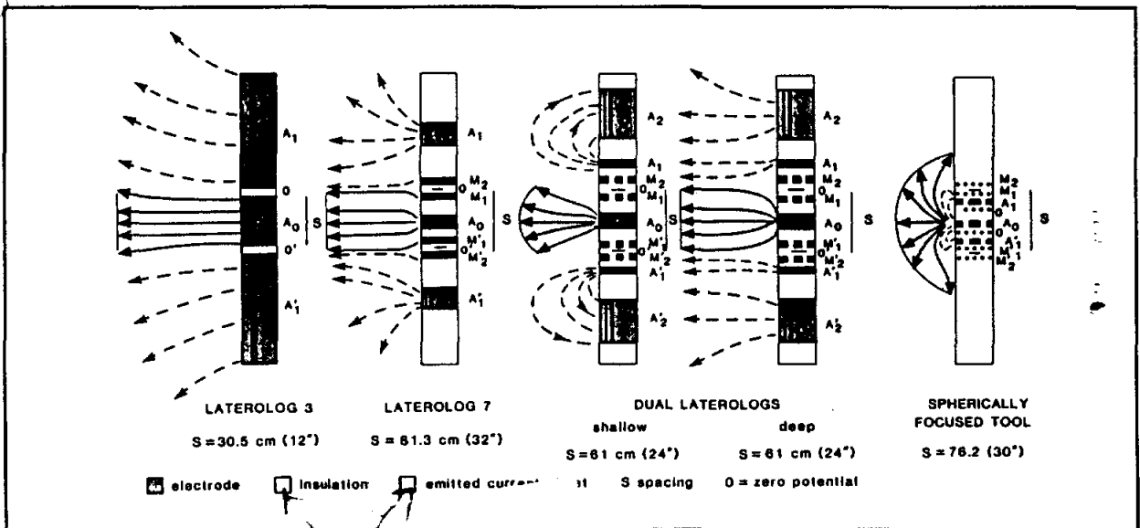
Figure 9-3. Schematic of Schlumberger focused mandrel resistivity tools. A = electrode, M =
