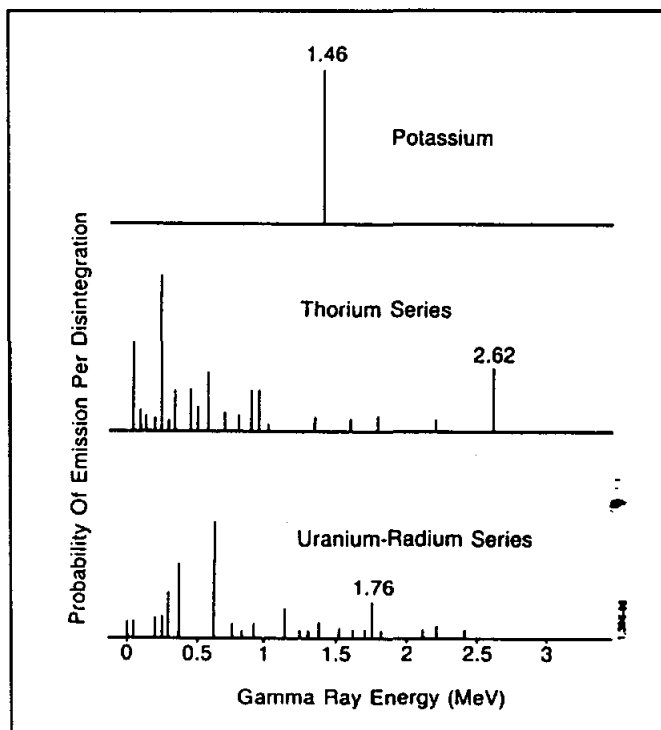
Figure 10-8. Gamma ray emission spectra of radioactive minerals. The energy level of the principal peak of each element is noted (From Schlumberger, 1989).
