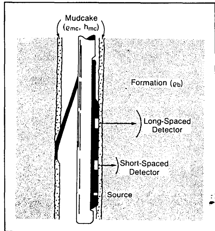
Figure 13-1. Schematic drawing of a compensated density tool (From Schlumberger, 1989, modified from Wahl, et al., 1964).
