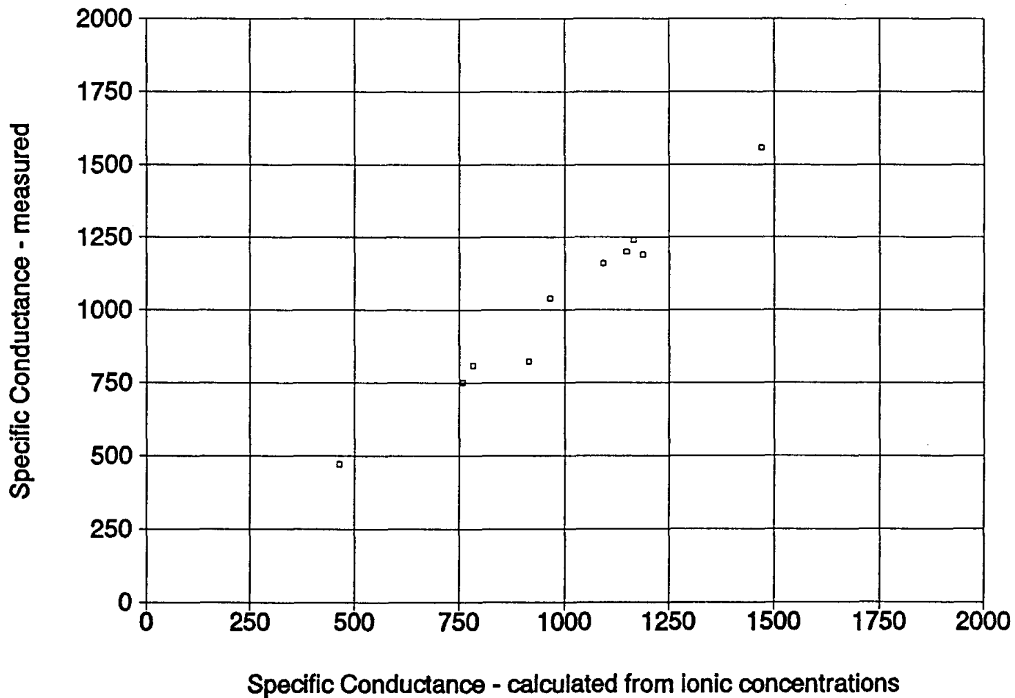
Figure 2-13. A graph of C_{W_{Measured}} versus C_{W_{Ion Conc.}} values ranging between 0 and 2,000 \mu\text{mhos/cm} . The data are from water analyses performed by Texas Department of Health Laboratories.
