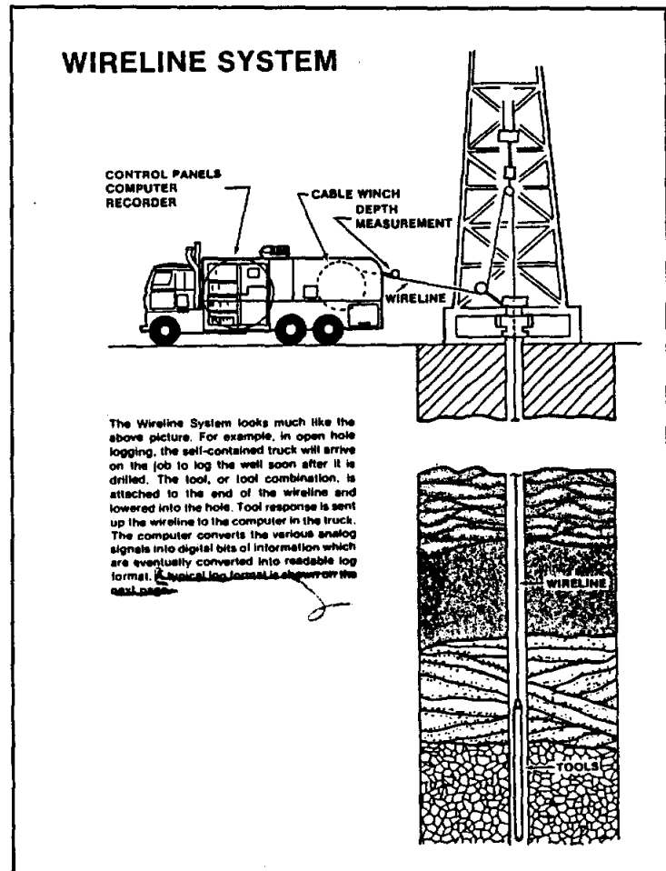
Figure 5-1. A typical petroleum logging system (From Gearhart, 1981).
