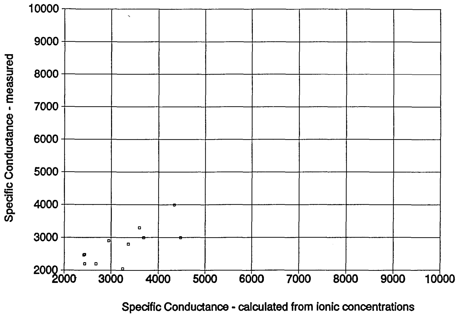
Figure 2-11. A graph of C_{w, \text{Measured}} versus C_{w, \text{Ion Conc.}} values ranging between 2,000 and 10,000 \mu\text{mhos/cm} . The data are from water analyses performed by Pope Testing Laboratories.
