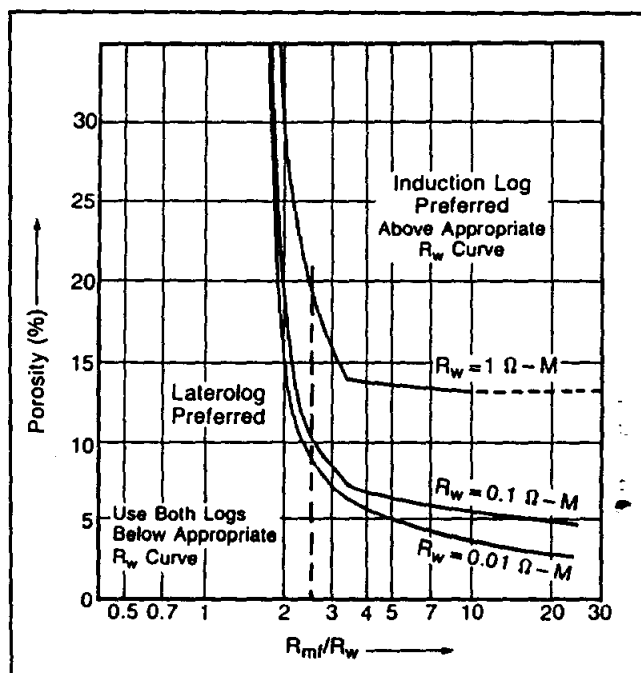
Figure 9-8. Preferred ranges for using induction logs and laterologs under normal borehole conditions (From Schlumberger, 1989).
