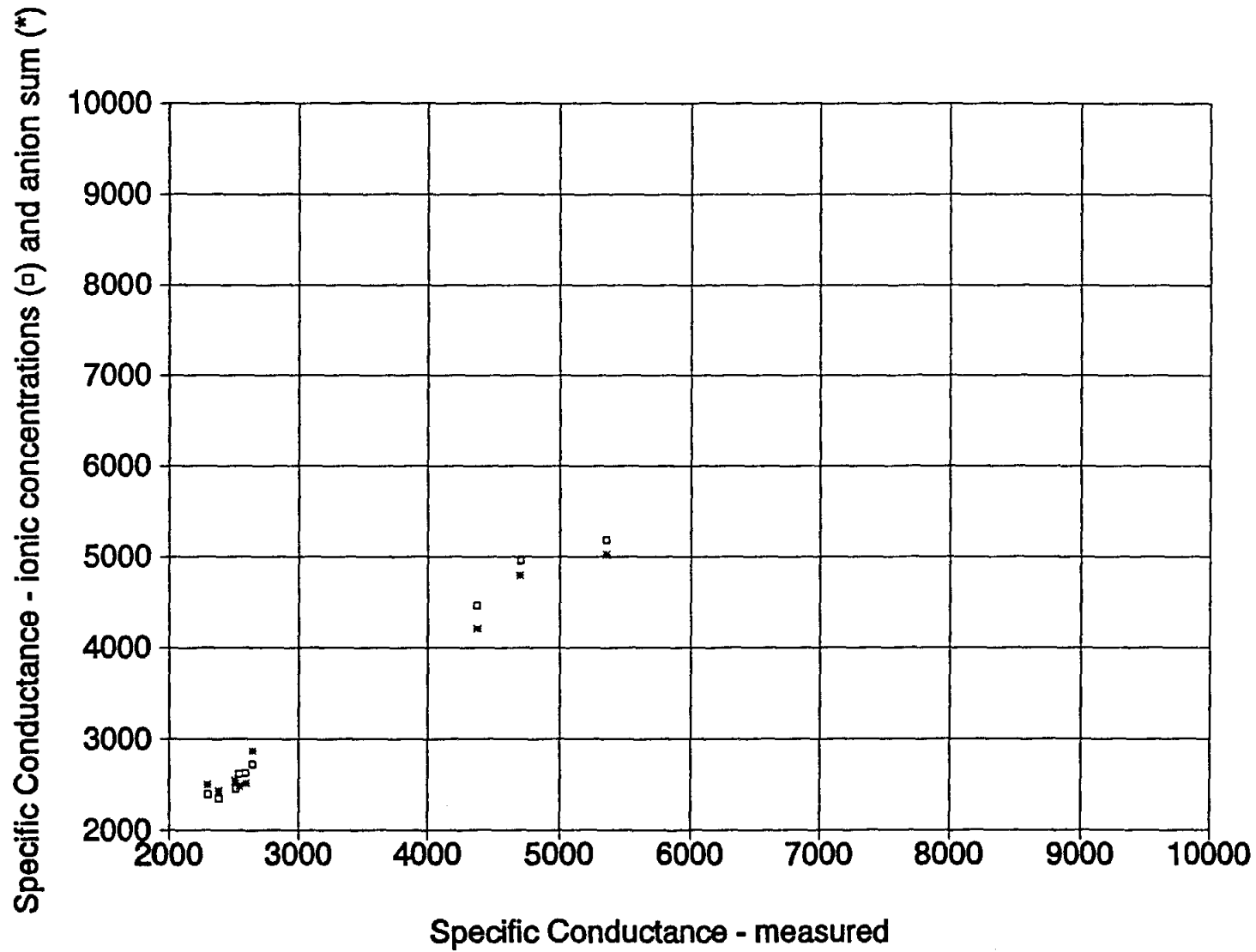
Figure 2-16. A graph of C_{w, \text{Measured}} versus C_{w, \text{Ion Conc.}} and C_{w, \text{Anion Sum}} values ranging between 2,000 and 10,000 \mu\text{mhos/cm} . The data are from water analyses performed by Curtis Laboratories.
