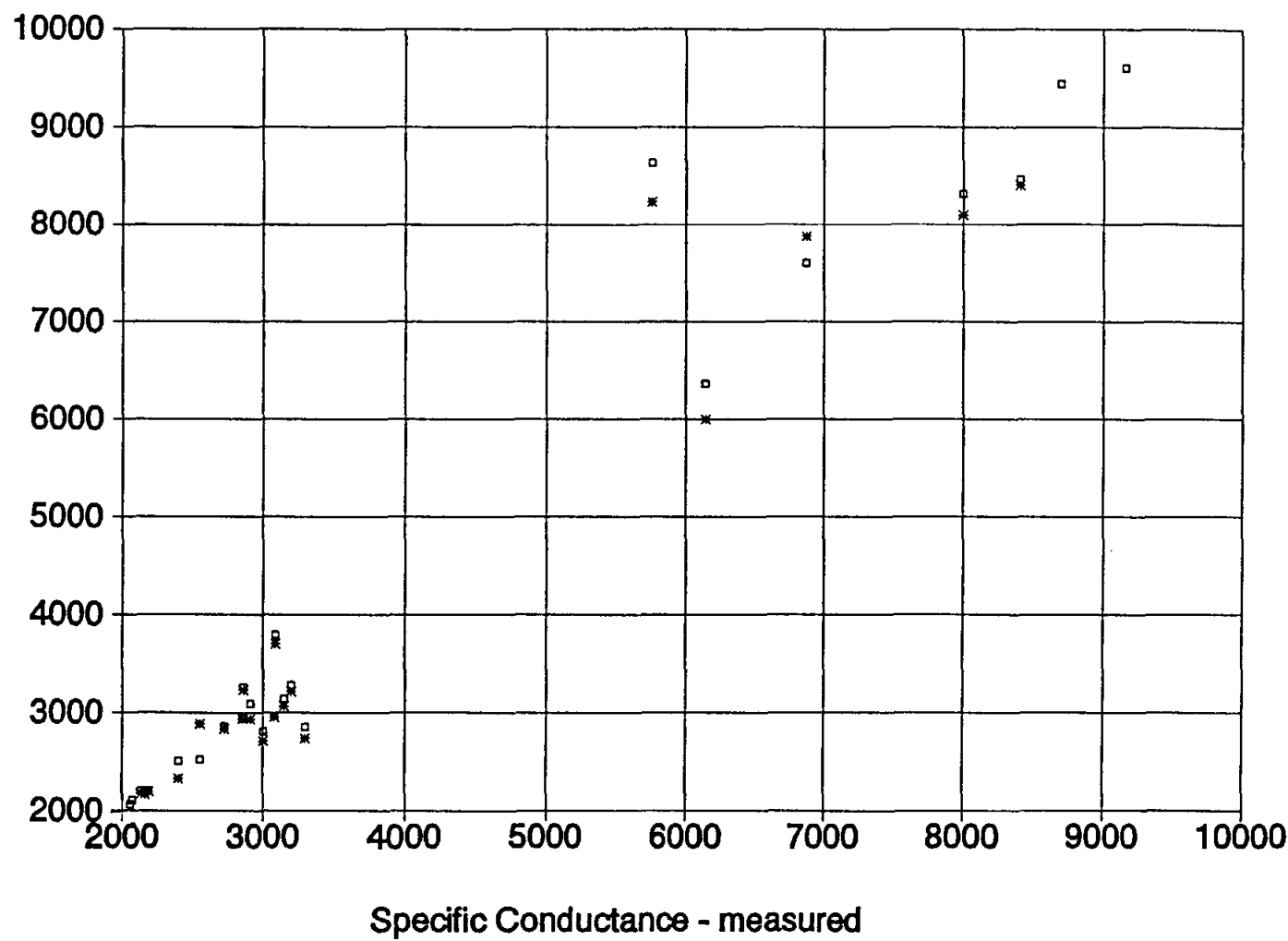
Figure 2-18. A graph of C_{w\text{Measured}} versus C_{w\text{Ion Conc.}} and C_{w\text{Anion Sum}} values ranging between 2,000 and 10,000 \mu\text{mhos/cm} . The data are from water analyses performed by Microbiology Service Laboratories.
