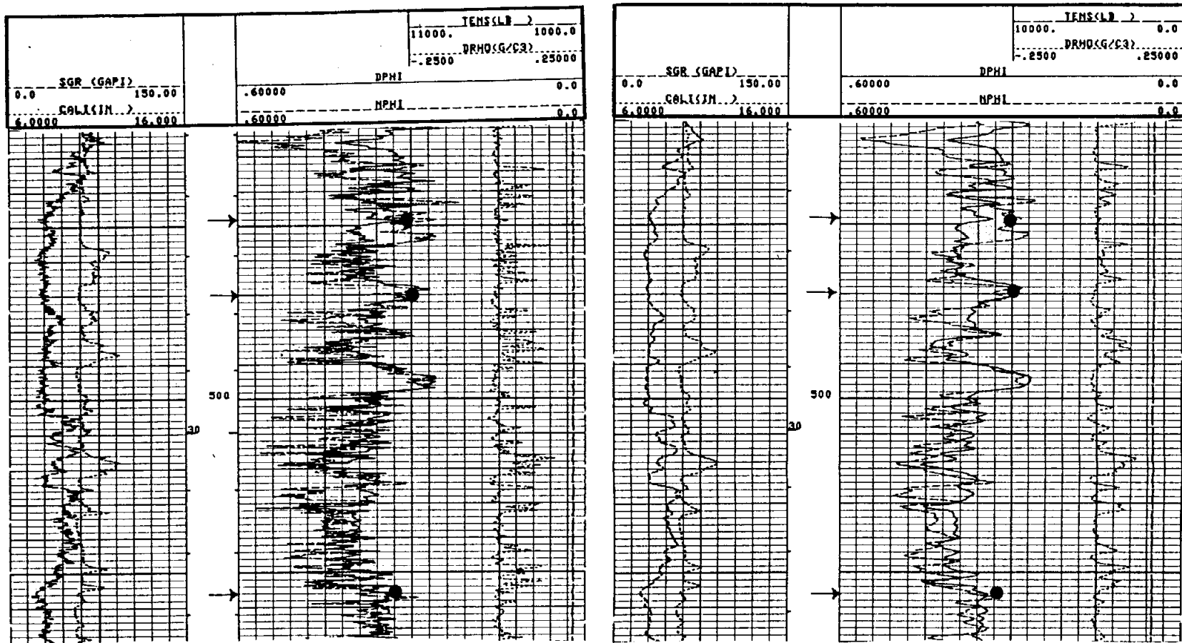
Figure 13-3 a & b. Comparison of high resolution (1.2 inch sampling rate) compensated density-neutron logs (13-3a) and normal density-neutron logs (13-3b). The high resolution pass has better vertical resolution. These logs illustrate the standard log presentation for conventional density and neutron porosity curves. In addition to the two porosity curves, the logs contain gamma ray (SGR), caliper (CALI), tension (TENS), and bulk density correction (DRHO) curves. Both porosity curves are plotted on a sandstone matrix. In shaly sandstones and shales neutron porosity (NPHI) reads greater than density porosity (DPHI). The curves overlay in shale-free sandstones. Zones in which density porosity reads greater than the neutron are due to either gas in the pores or mineralogical variations. Percussion sidewall cores were taken at the depths indicated by the arrows. Core porosities (plotted on the log) agree within 3 pu of the log porosities. Horizontal air permeabilities were 2565 md at 470 feet and 6541 md at 556 feet. See Figure 13-30 for a photomicrograph of a sidewall core. The negative DRHO corrections are due to the tool being miscalibrated. Positive corrections are due to washouts. The bit size is 9 7/8 inches and the borehole fluid is 9 lb/gal, native gel. The log is the Gulf Coast Aquifer. The well is the Alsay, NW Harris County MUD 21 and 22 #2, Harris County, Texas. Figures 10-10, 11-1, 13-4, and 13-9 provide additional data on this well.
