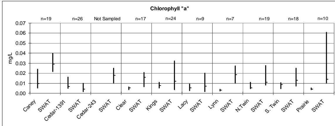
Figure 34. Measured and predicted chlorophyll 'a' (median, 25 th , and 75 th percentile), 1989 to 2002 Tributary Study.
