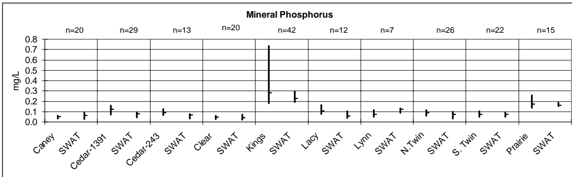
Figure 33. Measured and predicted mineral phosphorus (median, 25 th , and 75 th percentile), 1989 to 2002 Tributary Study.
