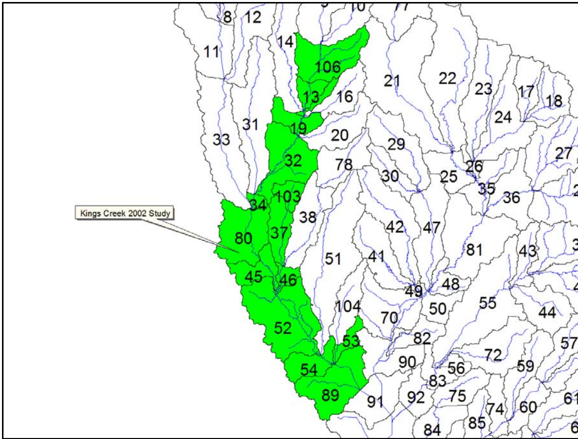
Figure 6. Kings Creek 2002 Study subbasins.
