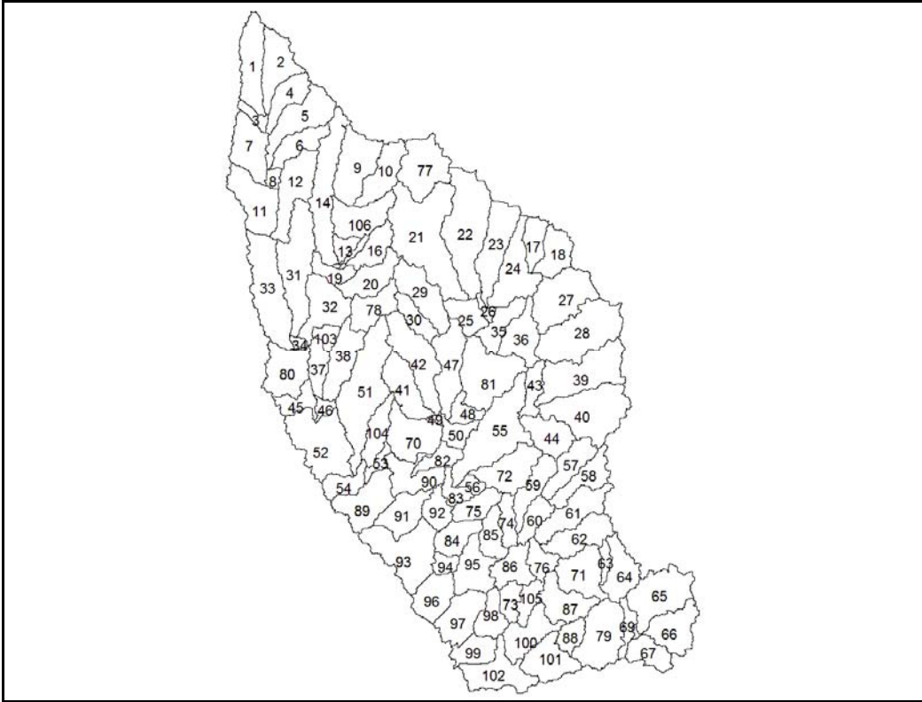
Figure 1b. Subbasins in Cedar Creek Watershed.
