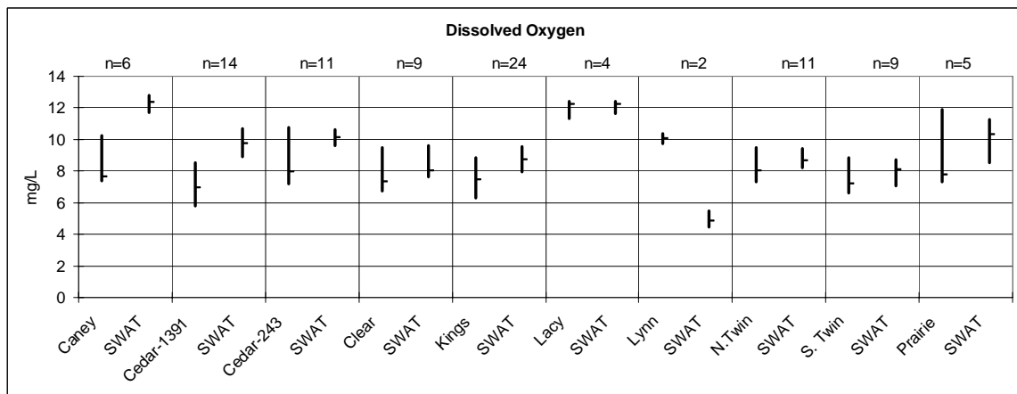
Figure 36. Measured and predicted dissolved oxygen (median, 25 th , and 75 th percentile), 1989 to 2002 Tributary Study.
