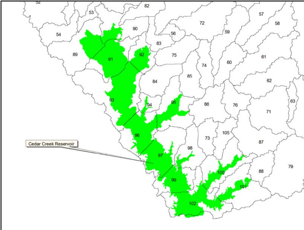
Figure 2. Subbasins submerged by Cedar Creek Reservoir.
