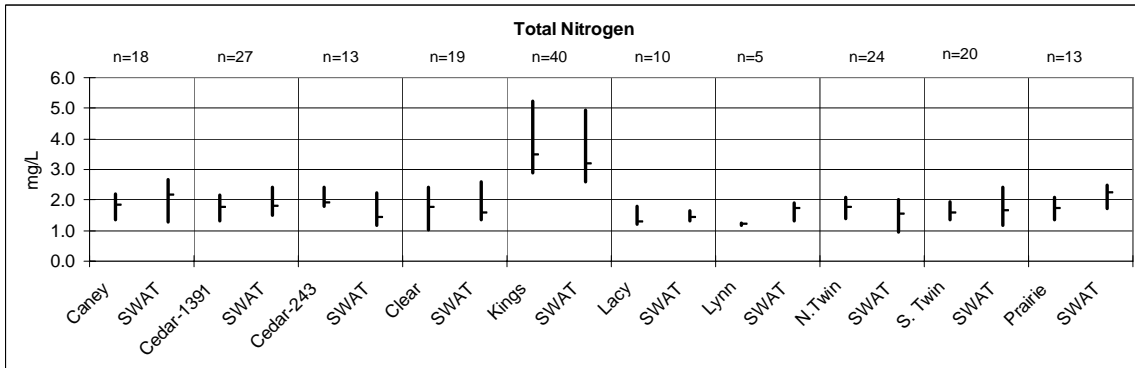
Figure 27. Measured and predicted total nitrogen (median, 25 th , and 75 th percentile), 1989 to 2002 Tributary Study.
