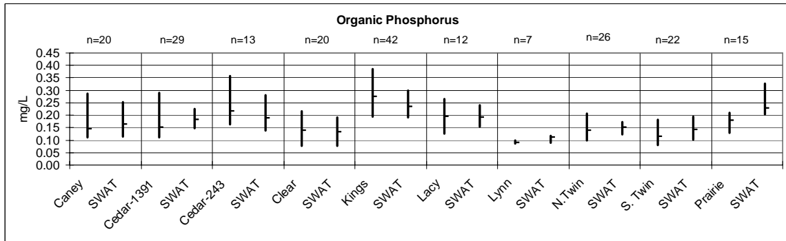
Figure 30. Measured and predicted organic phosphorus (median, 25 th , and 75 th percentile), 1989 to 2002 Tributary Study.
