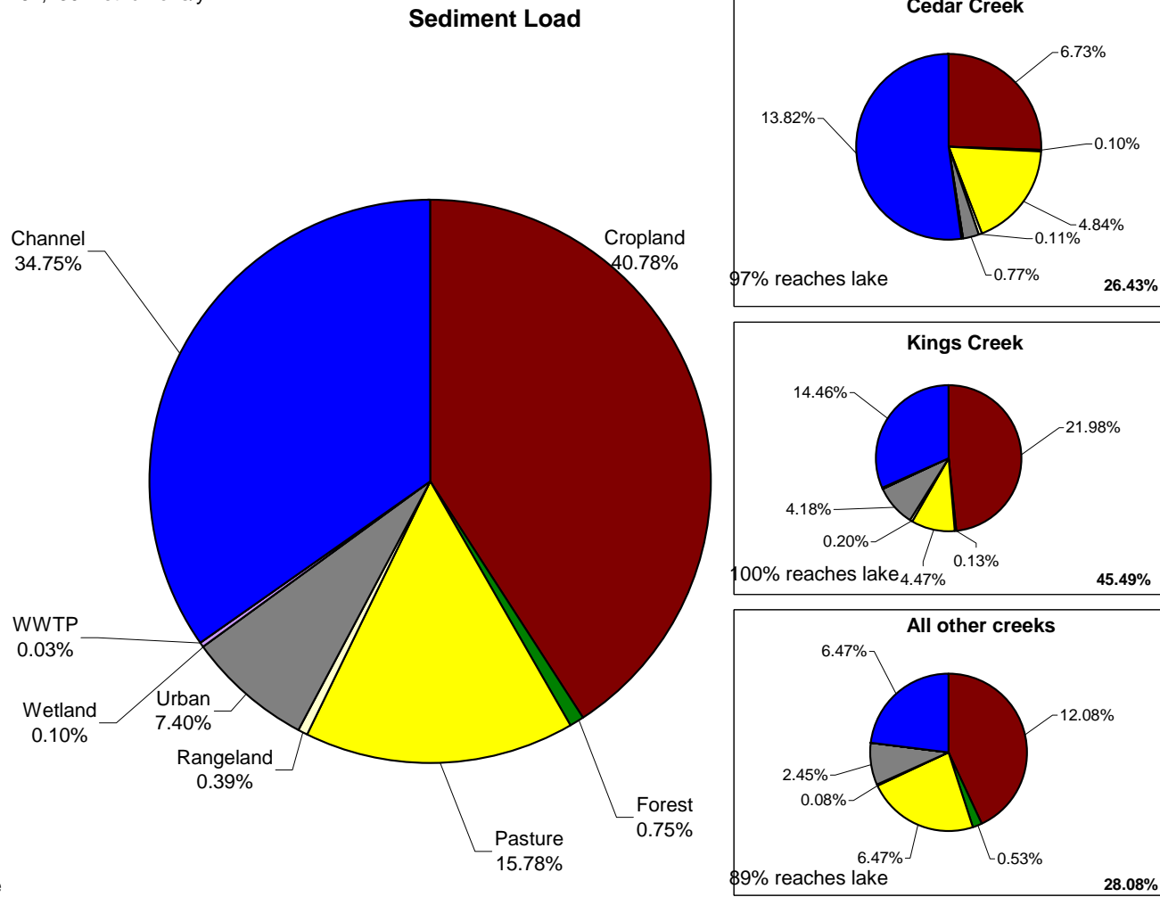
Figure 40. Sediment load by landuse and major creeks.
