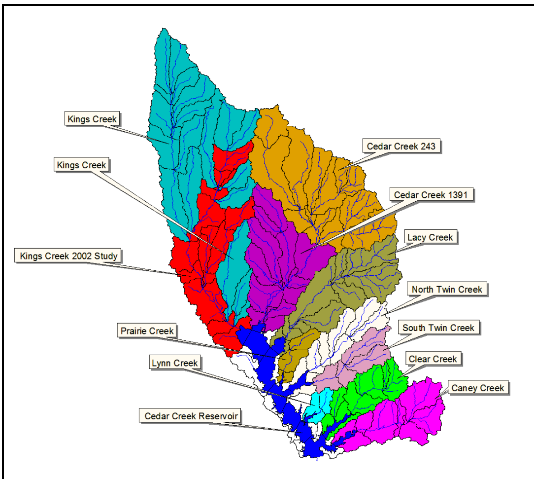
Figure 5. Tributaries of Cedar Creek Watershed.
