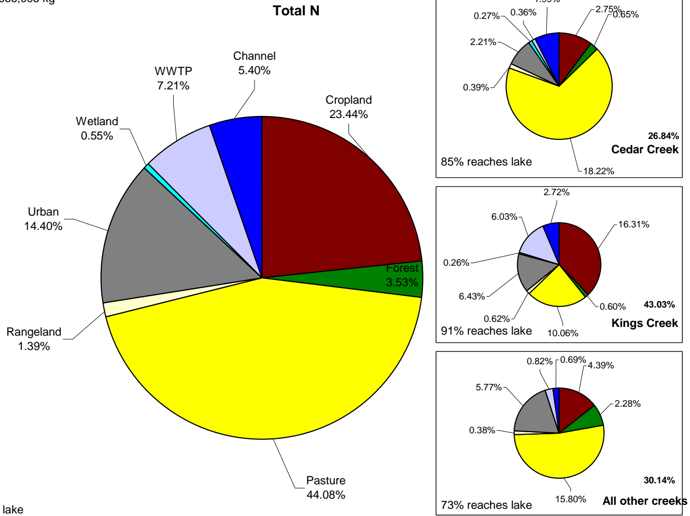
Figure 45. Total Nitrogen load by landuse and major creeks.
