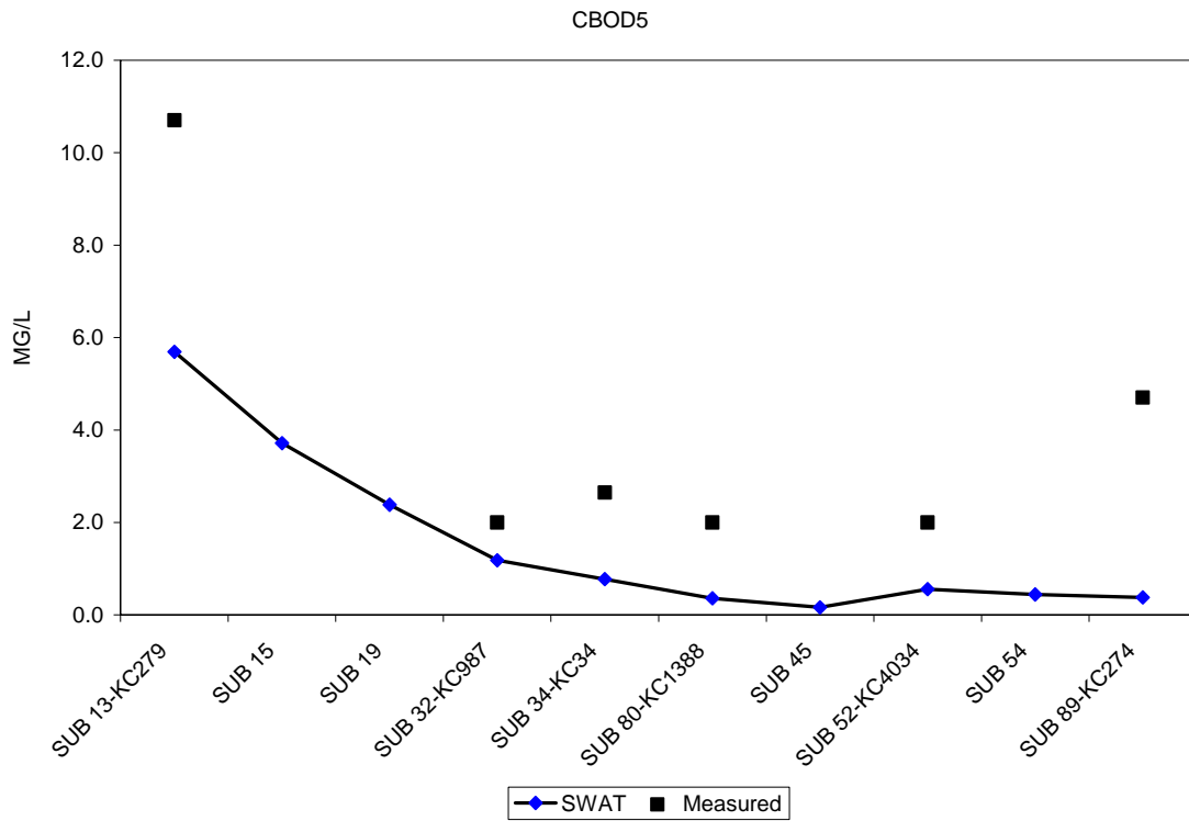
Figure 24. Measured and predicted CBOD5, Kings Creek 2002 Study.
