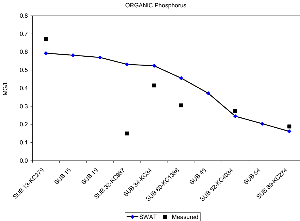
Figure 19. Measured and predicted organic phosphorus, Kings Creek 2002 Study.
