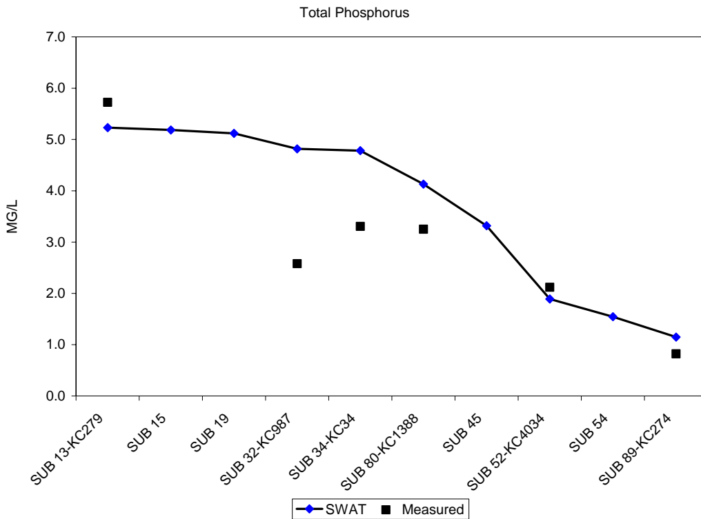
Figure 17. Measured and predicted total phosphorus, Kings Creek 2002 Study.
