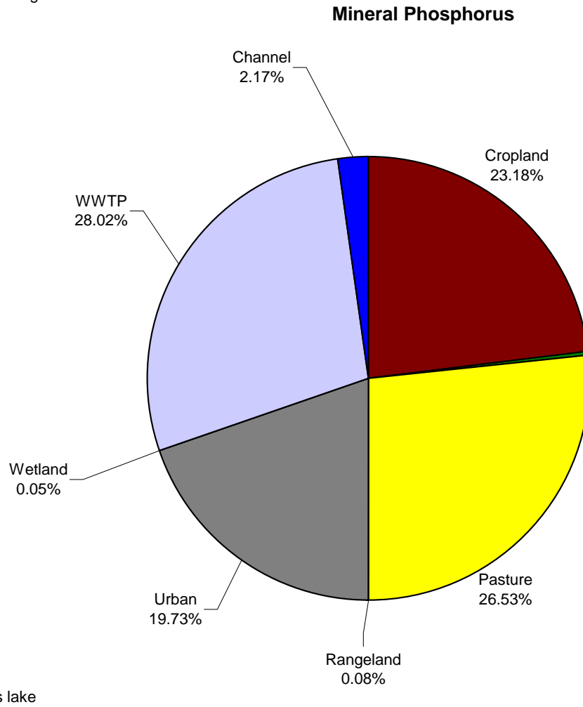
Figure 44. Mineral Phosphorus load by landuse and major creeks.
