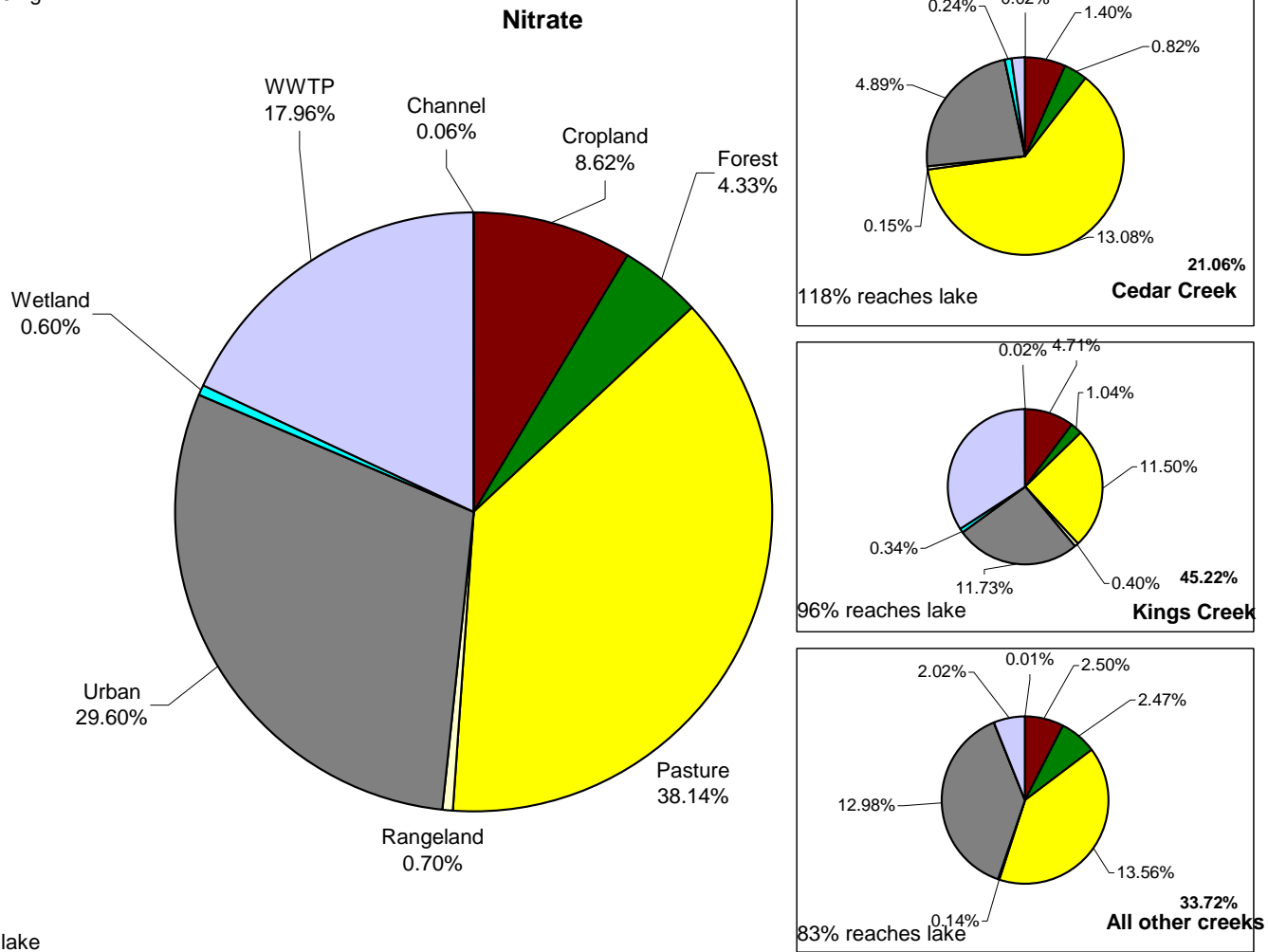
Figure 43. Nitrate load by landuse and major creeks.
