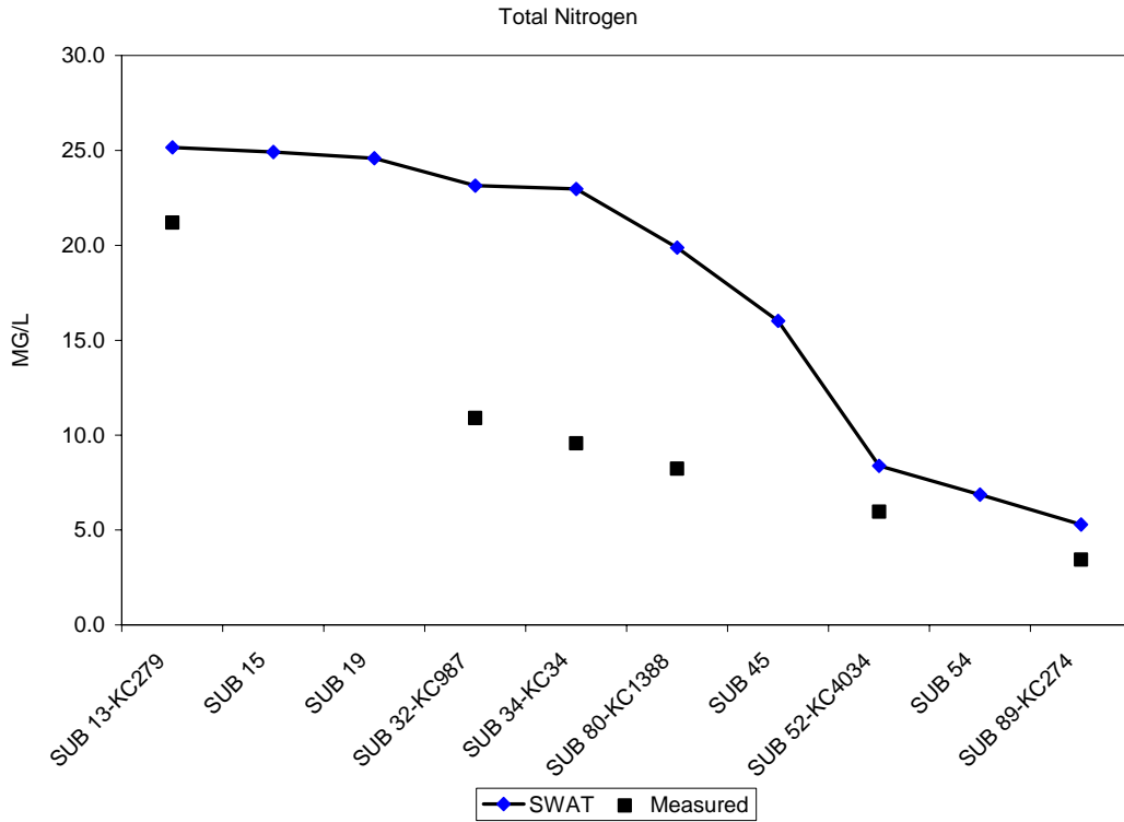
Figure 16. Measured and predicted total nitrogen, Kings Creek 2002 Study.
