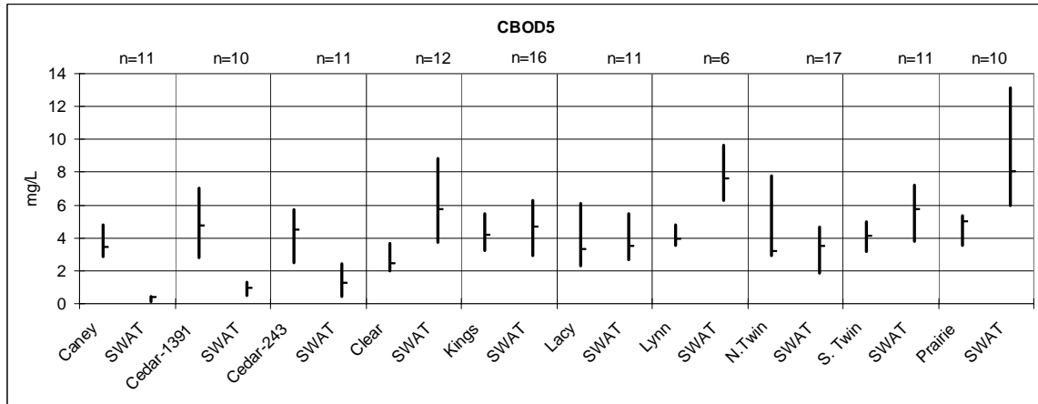
Figure 35. Measured and predicted CBOD5 (median, 25 th , and 75 th percentile), 1989 to 2002 Tributary Study.
