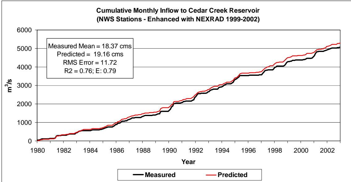
Figure 9. Cumulative monthly measured and predicted inflow to Cedar Creek Reservoir, January 1980 through December 2002.
