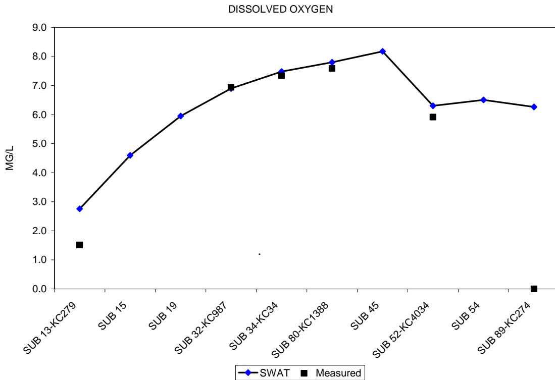
Figure 25. Measured and predicted dissolved oxygen, Kings Creek 2002 Study.
