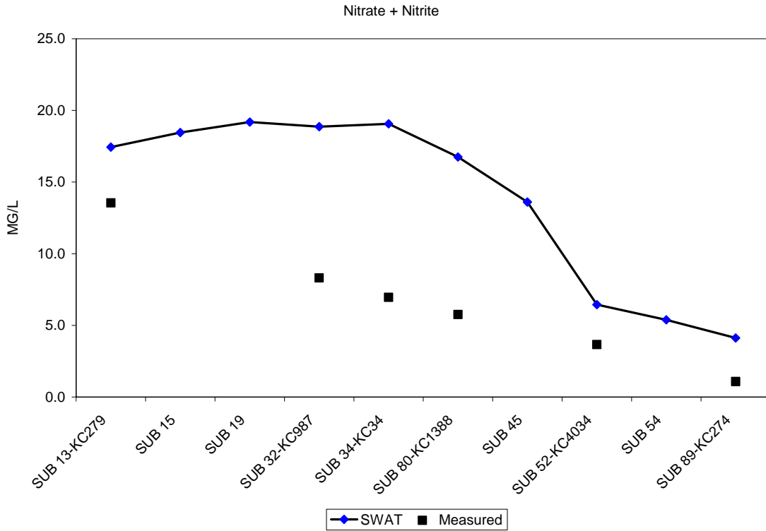
Figure 20. Measured and predicted nitrate + nitrite nitrogen, Kings Creek 2002 Study.
