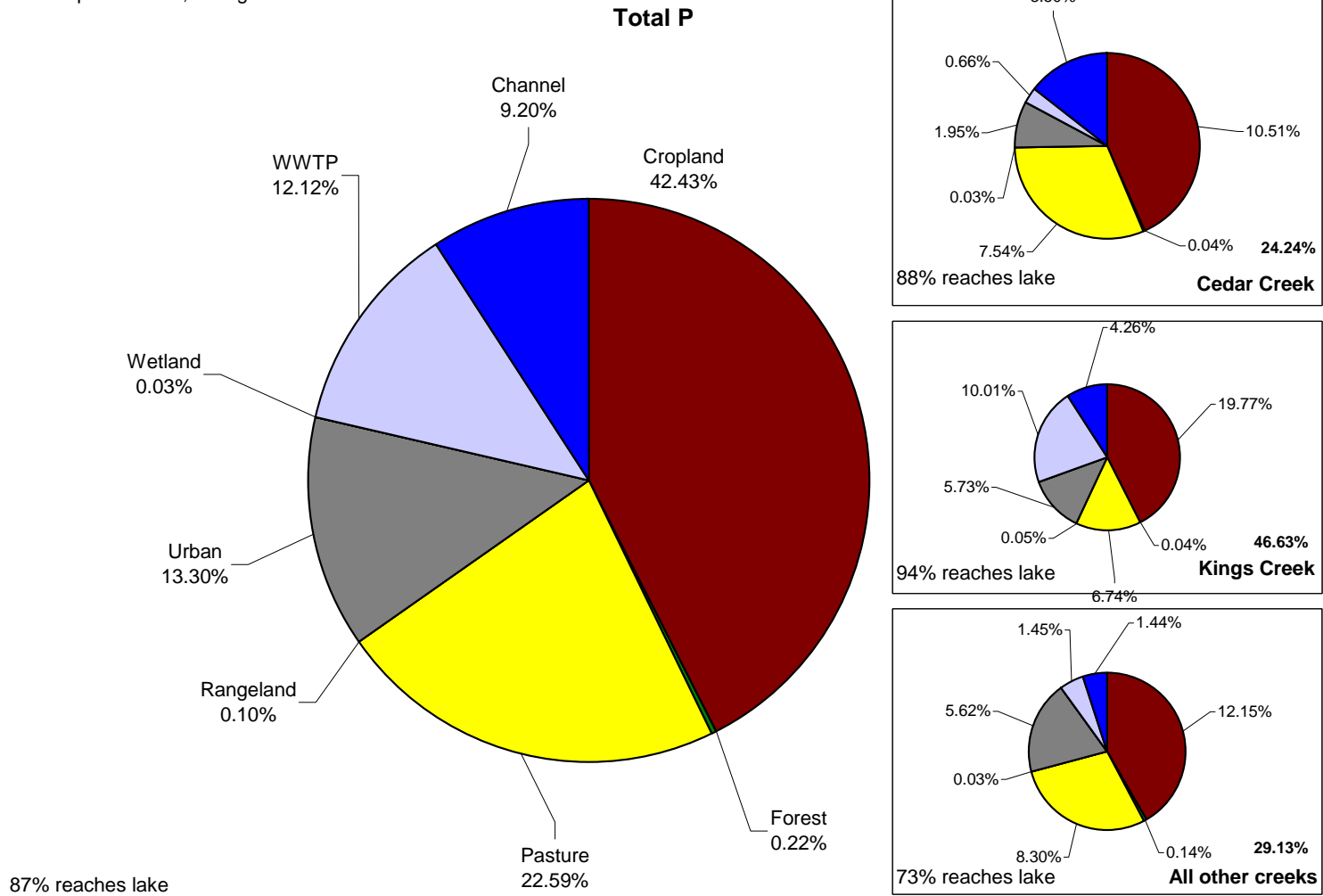
Figure 46. Total Phosphorus load by landuse and major creeks.
