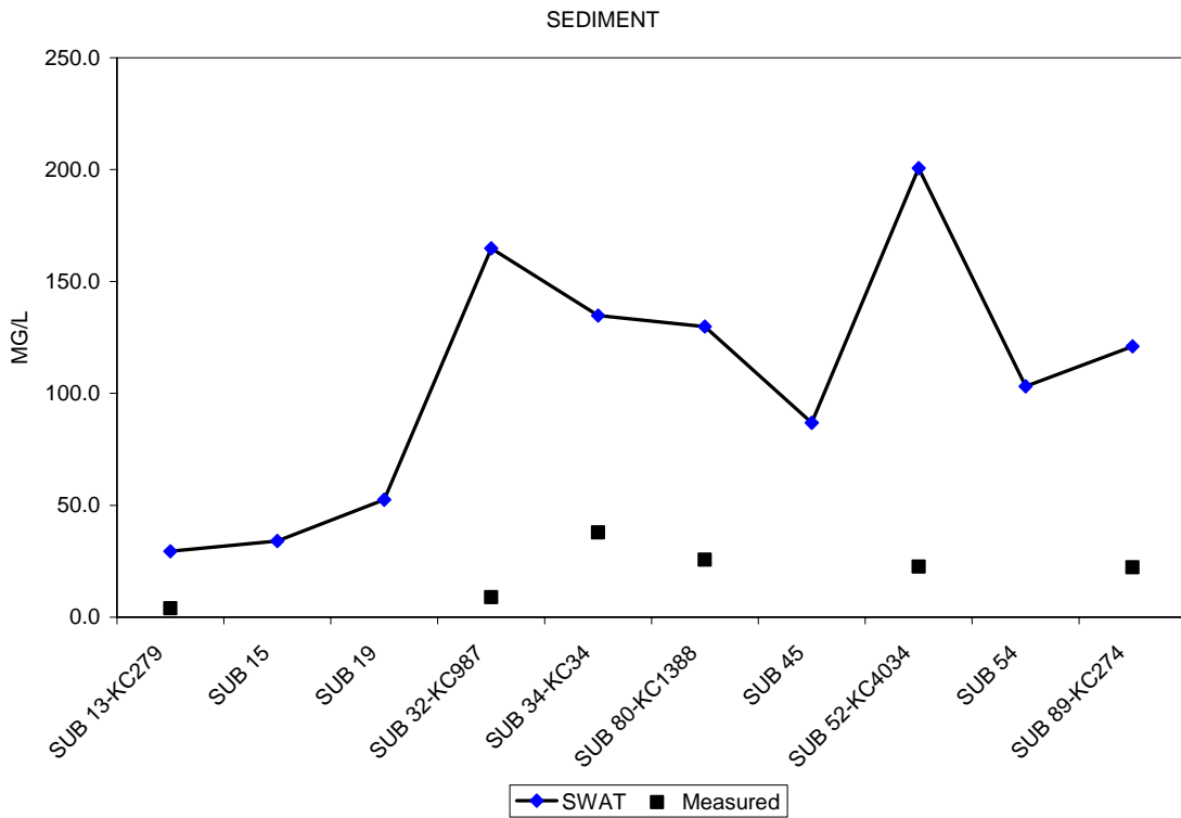
Figure 15. Measured and predicted sediment, Kings Creek 2002 Study.
