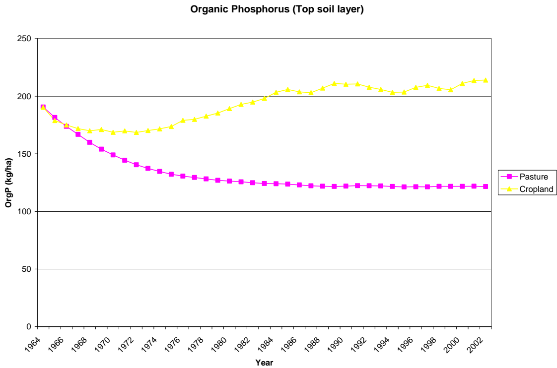
Figure 4. Organic Phosphorus build-up due to fertilizer application.
