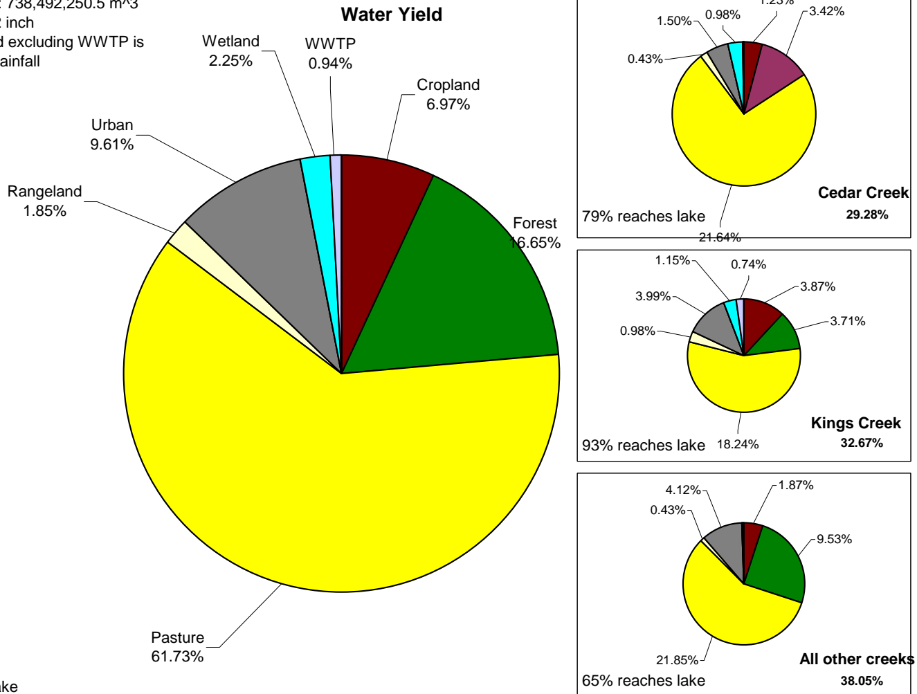
Figure 39. Water Yield by landuse and major creeks.
