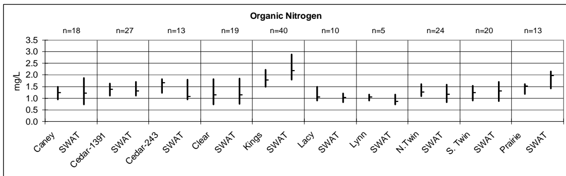
Figure 29. Measured and predicted organic nitrogen (median, 25 th , and 75 th percentile), 1989 to 2002 Tributary Study.
