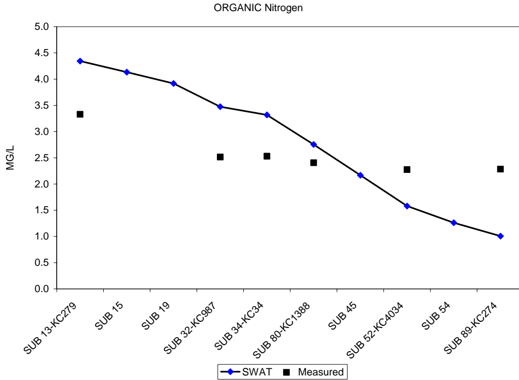
Figure 18. Measured and predicted organic nitrogen, Kings Creek 2002 Study.
