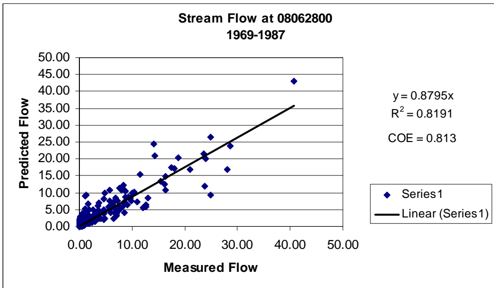
Figure 10. Measured versus predicted flow at stream gage 08062800.
