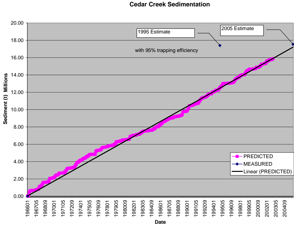
Figure 13. Measured and predicted sediment accumulation in Cedar Creek Reservoir from 1966 through 1994.
