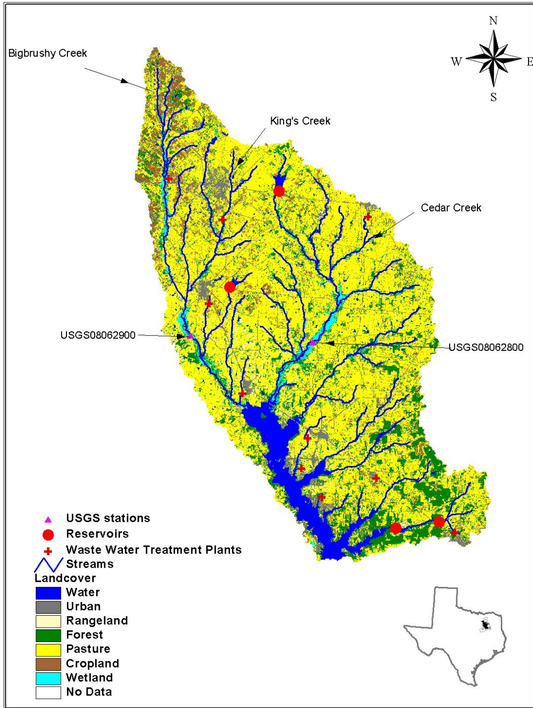
Figure 1a. Landcover of Cedar Creek Watershed (1992 NLCD + 2001 Urban).
