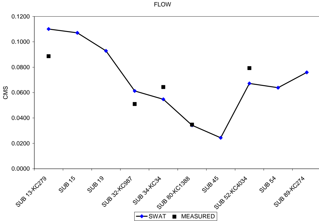
Figure 14. Measured and predicted flow, Kings Creek 2002 Study.
