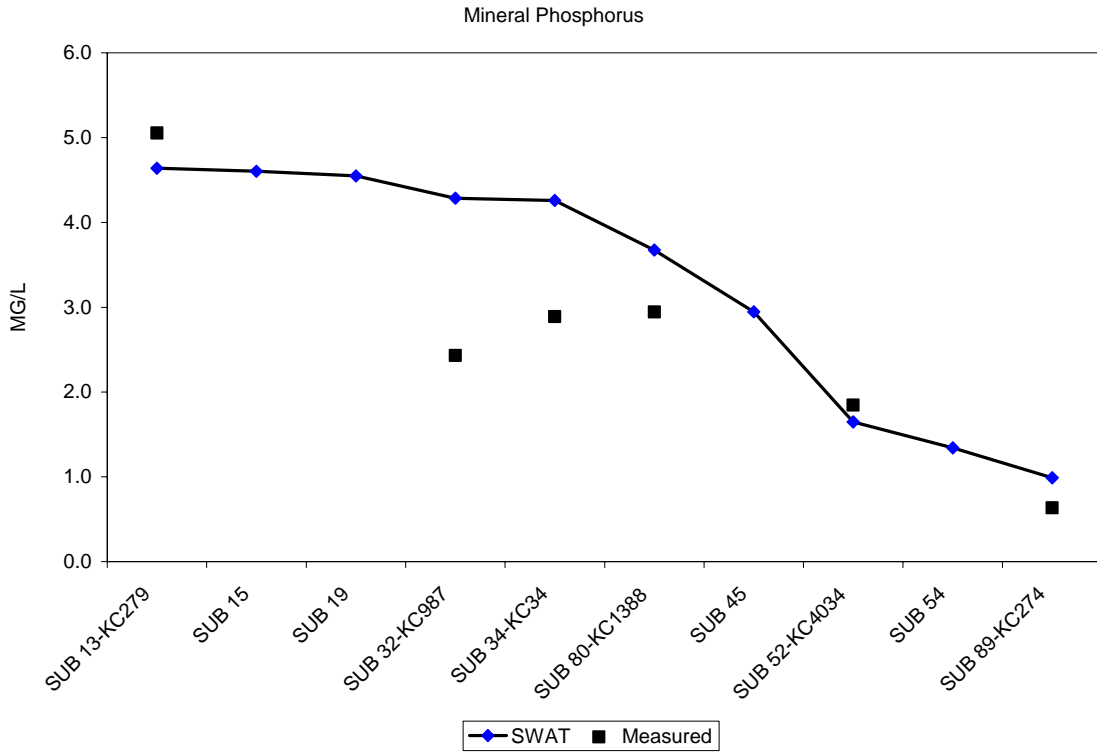
Figure 22. Measured and predicted mineral phosphorus, Kings Creek 2002 Study.
