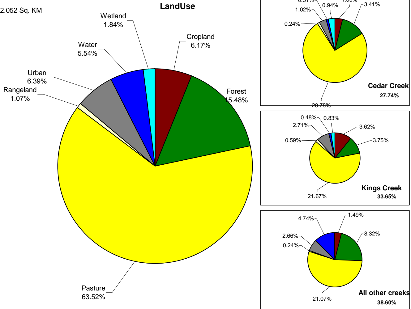
Figure 38. Landuse distribution by major creeks.
