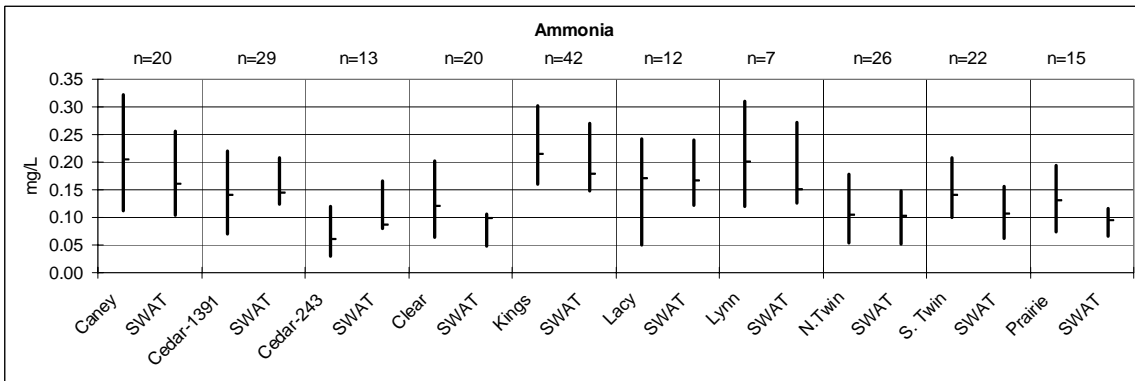
Figure 32. Measured and predicted ammonia (median, 25 th , and 75 th percentile), 1989 to 2002 Tributary Study.
