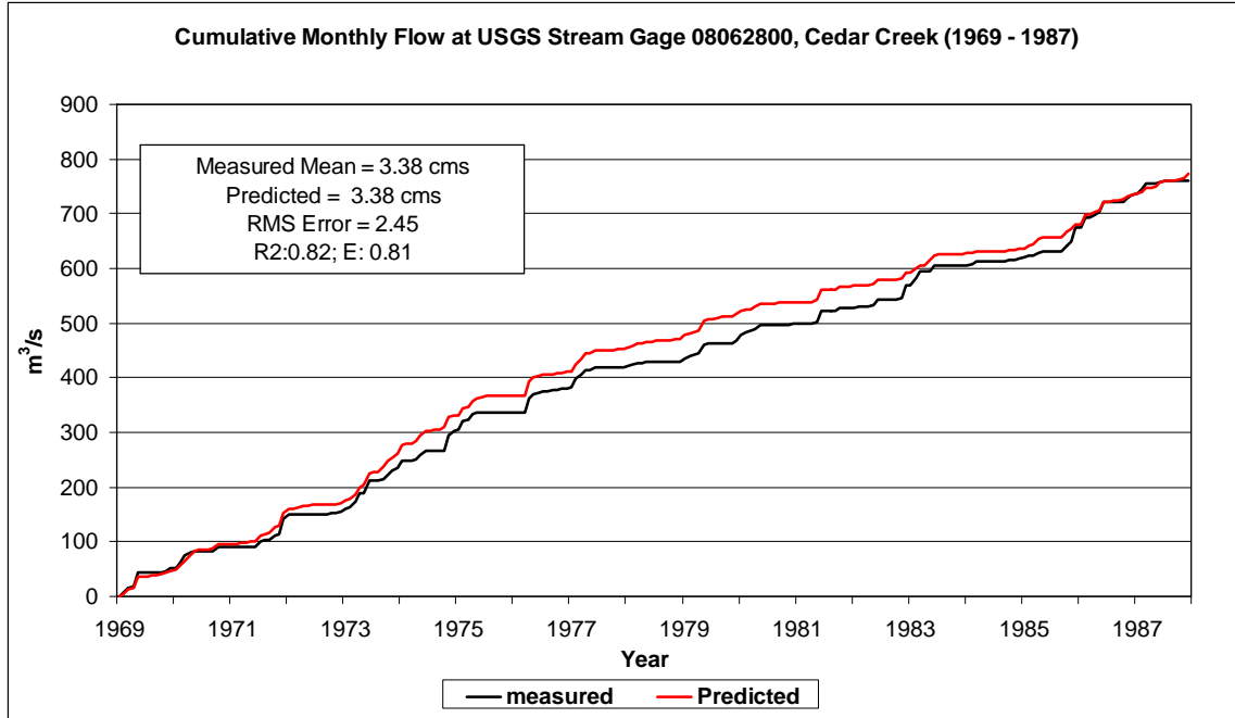
Figure 7. Cumulative monthly measured and predicted flow at stream gage 08062800 (subbasin 81), January 1969 through September 1987.
