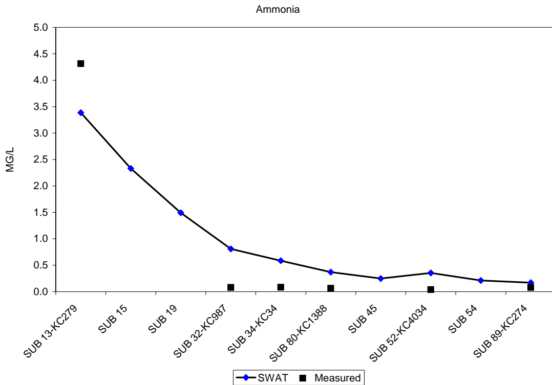
Figure 21. Measured and predicted ammonia nitrogen, Kings Creek 2002 Study.
