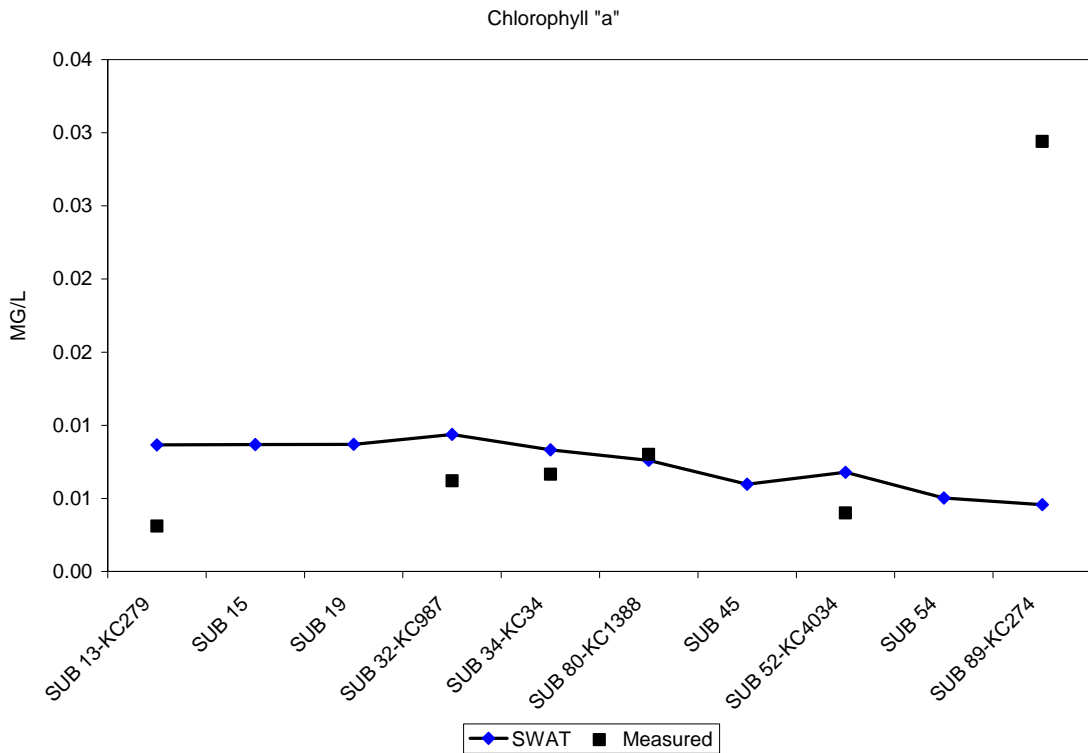
Figure 23. Measured and predicted chlorophyll 'a', Kings Creek 2002 Study.
