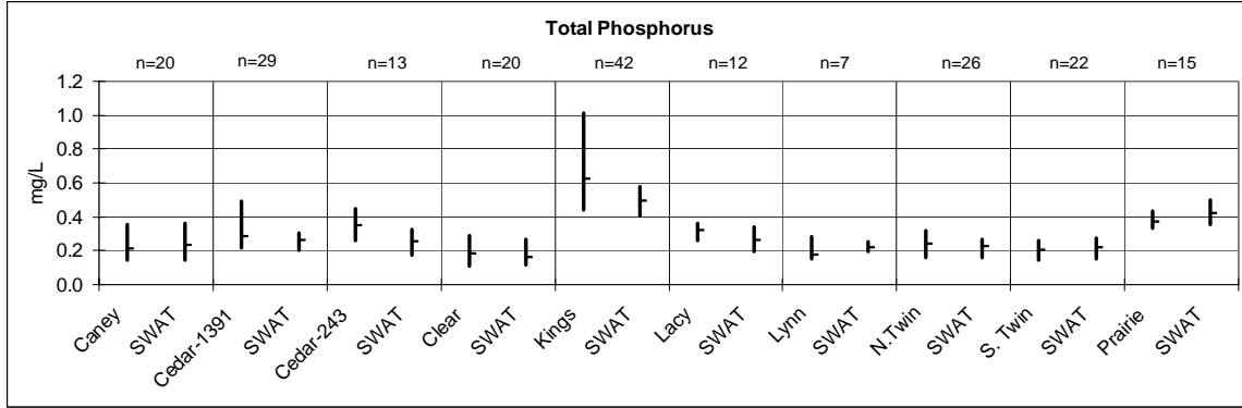
Figure 28. Measured and predicted total phosphorus (median, 25 th , and 75 th percentile), 1989 to 2002 Tributary Study.
