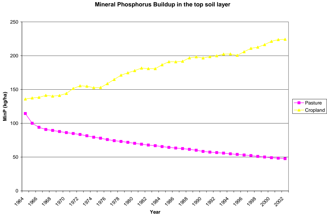
Figure 3. Mineral Phosphorus build-up due to fertilizer application.
