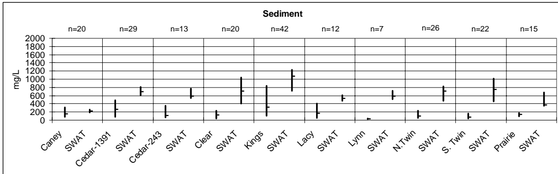
Figure 26. Measured and predicted sediment (TSS) (median, 25 th , and 75 th percentile), 1989 to 2002 Tributary Study.
