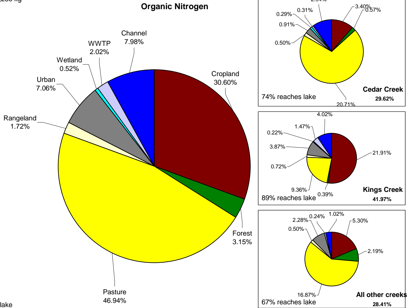
Figure 41. Organic Nitrogen load by landuse and major creeks.
