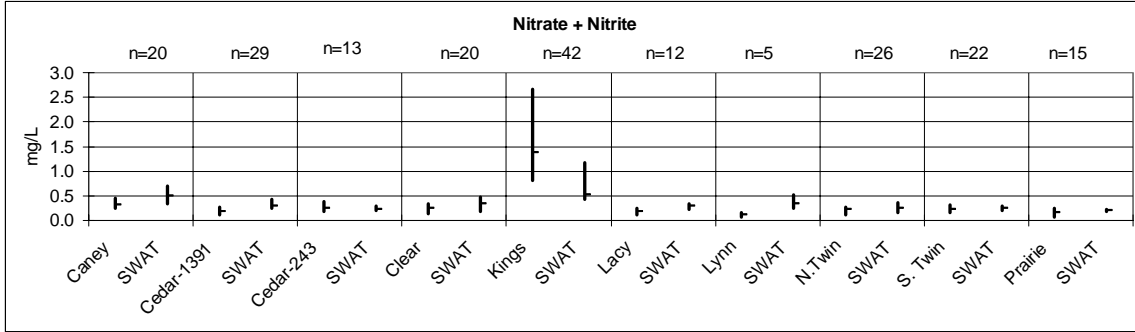
Figure 31. Measured and predicted nitrate + nitrite (median, 25 th , and 75 th percentile), 1989 to 2002 Tributary Study.
