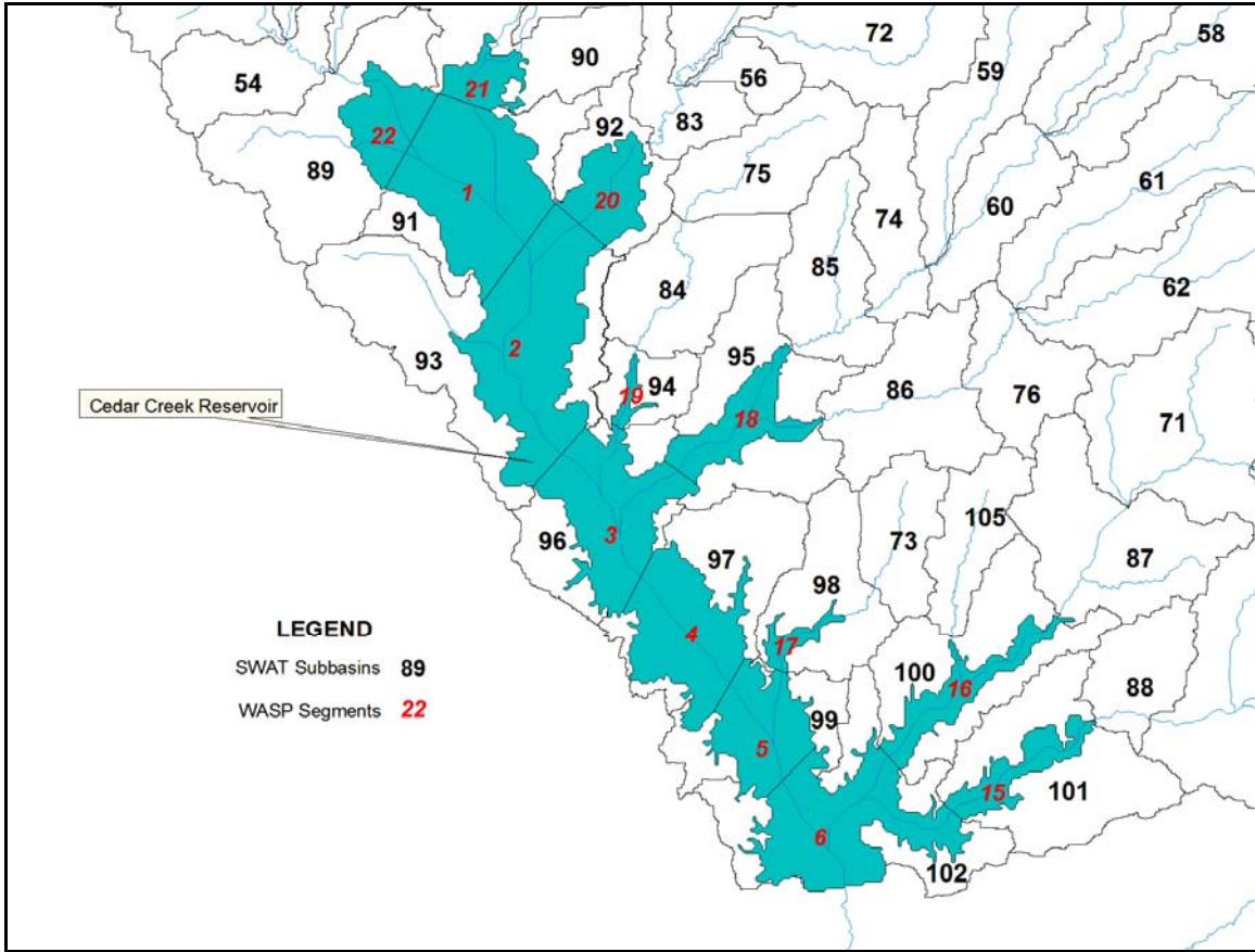
Figure 37. WASP segments and corresponding SWAT subbasins for Cedar Creek Reservoir.
