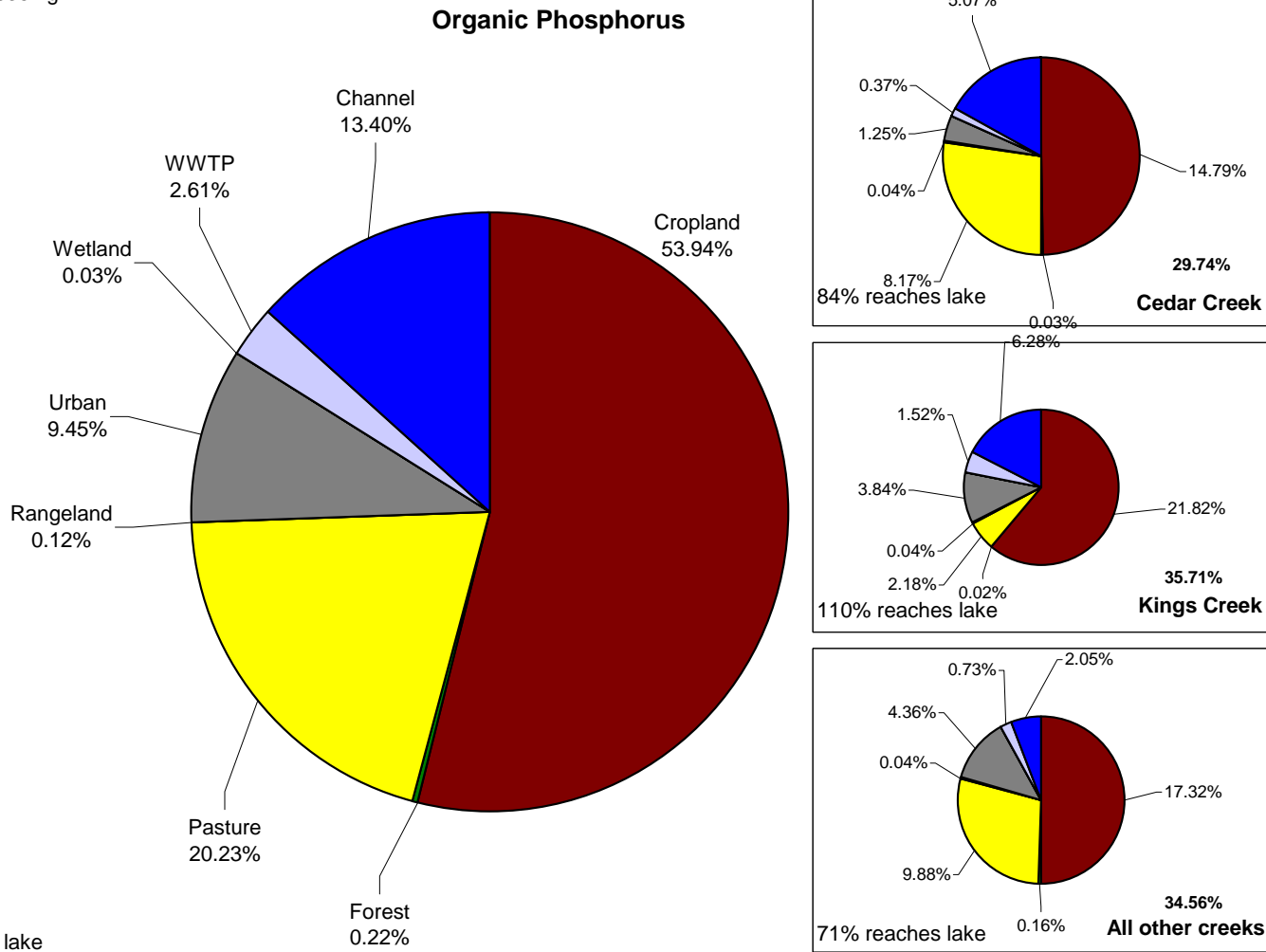
Figure 42. Organic Phosphorus load by landuse and major creeks.
