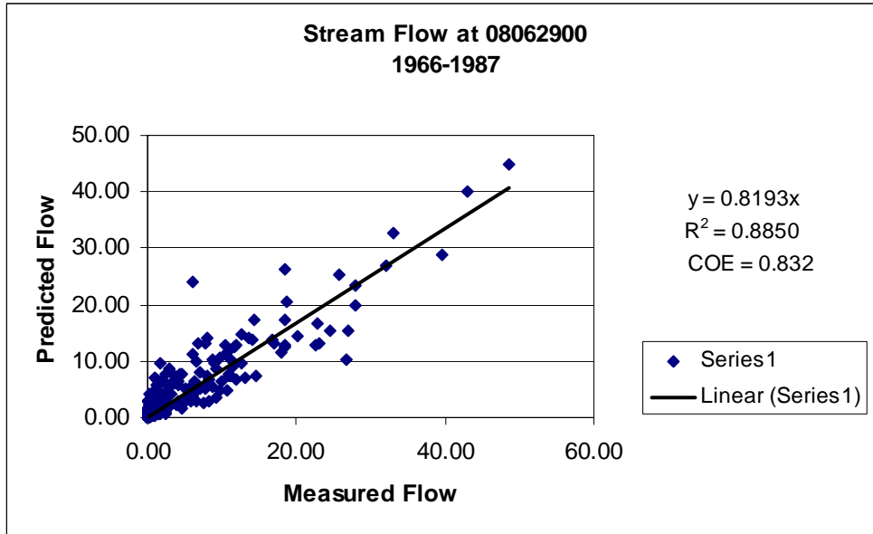
Figure 11. Measured versus predicted flow at stream gage 08062900.
