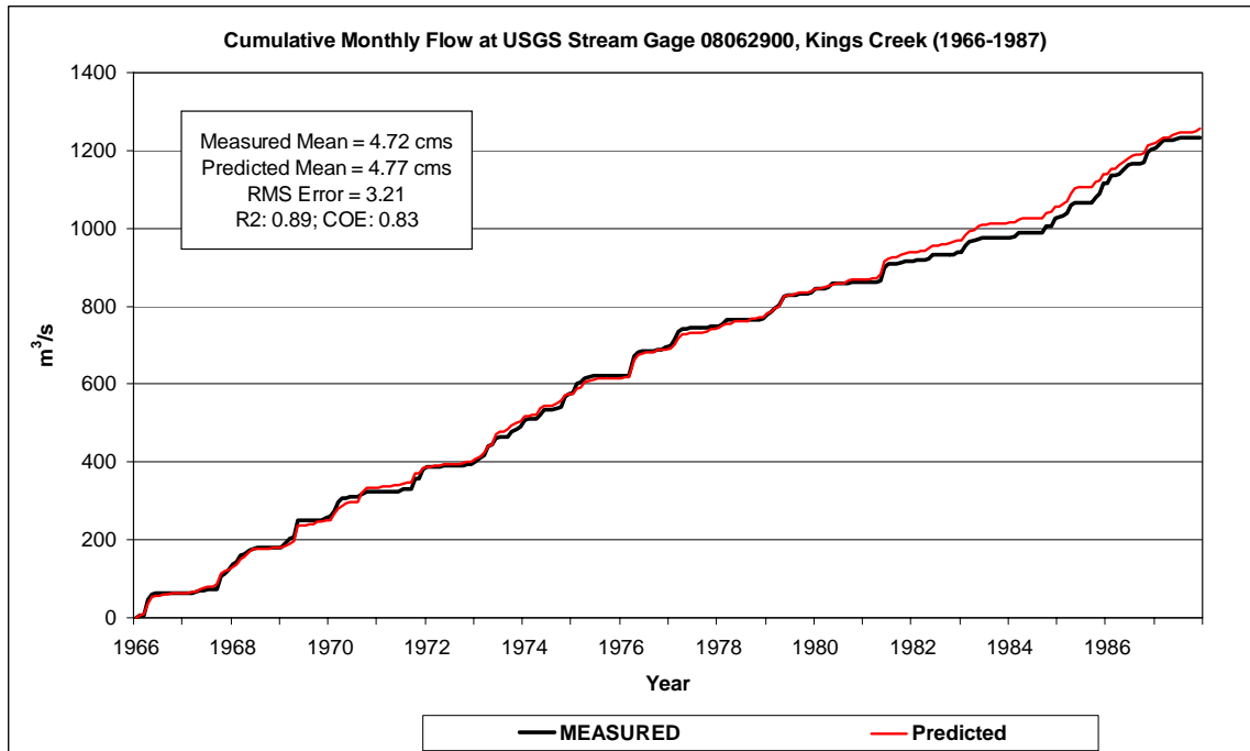
Figure 8. Cumulative monthly measured and predicted flow at stream gage 08062900 (subbasin 80), January 1963 through September 1987.
