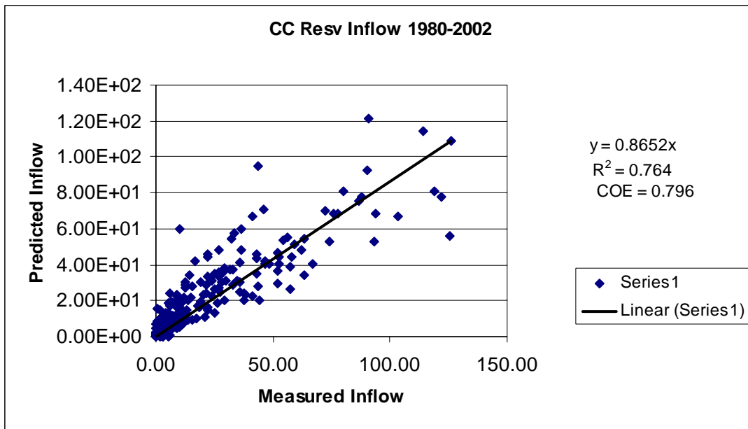
Figure 12. Measured versus predicted inflow to Cedar Creek Reservoir, 1980 through 2002.
