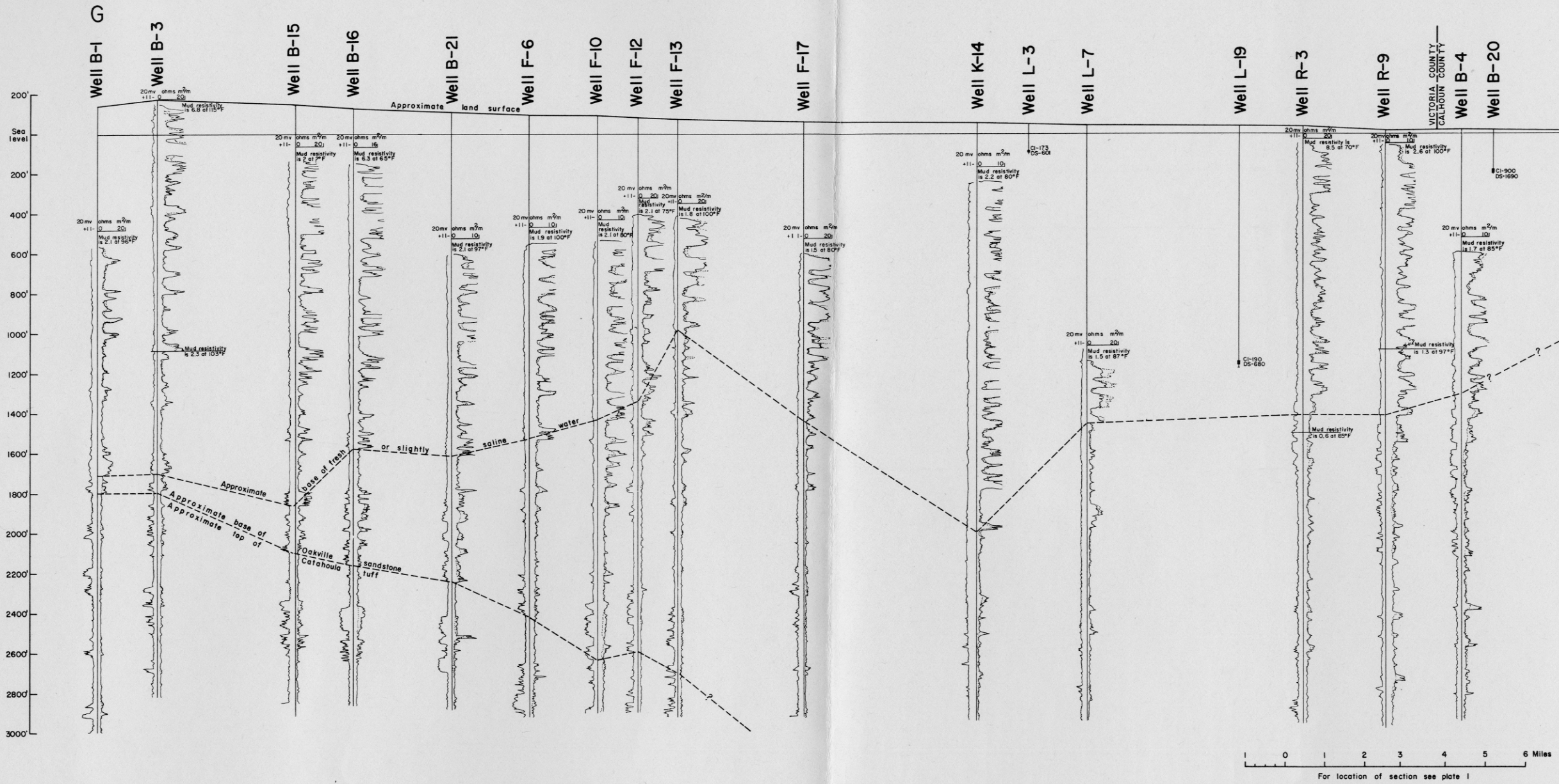
CROSS SECTION G-G', VICTORIA AND CALHOUN COUNTIES, TEXAS
