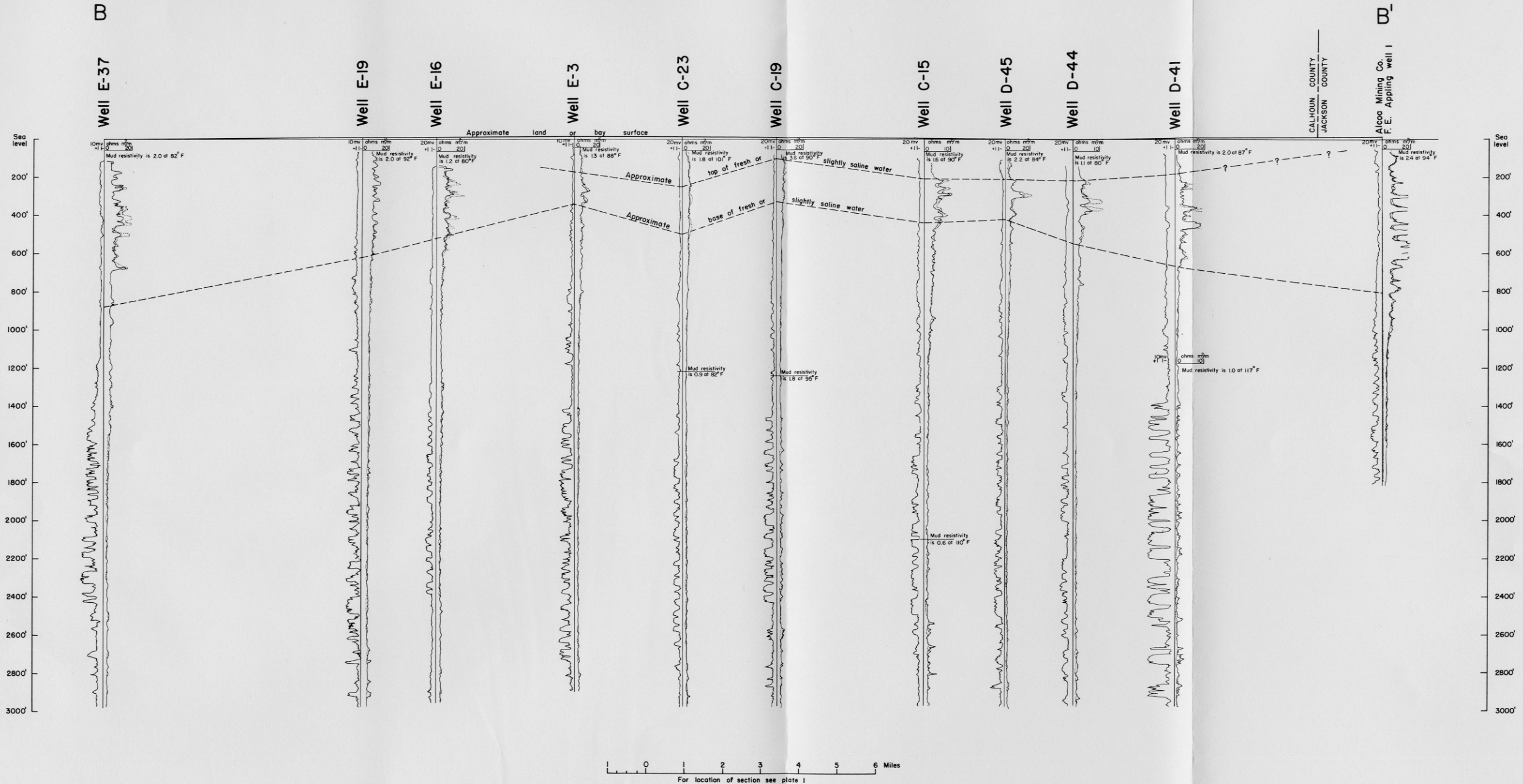
CROSS SECTION B-B', CALHOUN COUNTY, TEXAS
