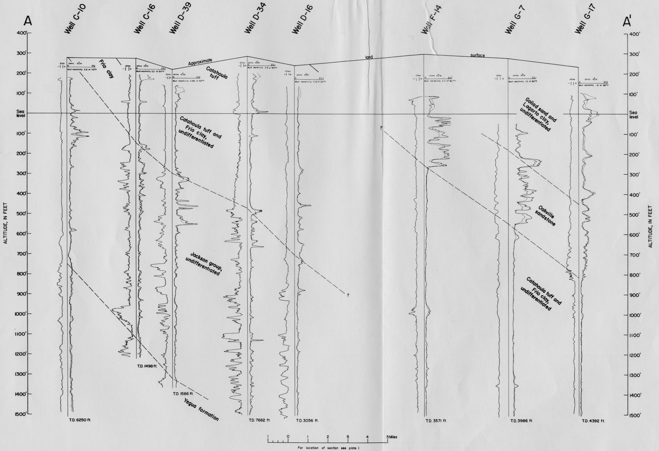
GEOLOGIC SECTION A-A', LIVE OAK COUNTY
