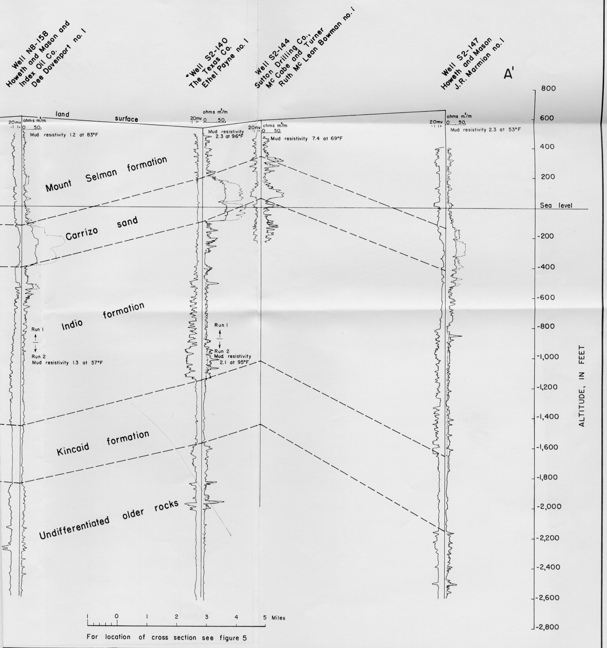
CROSS SECTION A-A', DIMMIT COUNTY, TEXAS.
